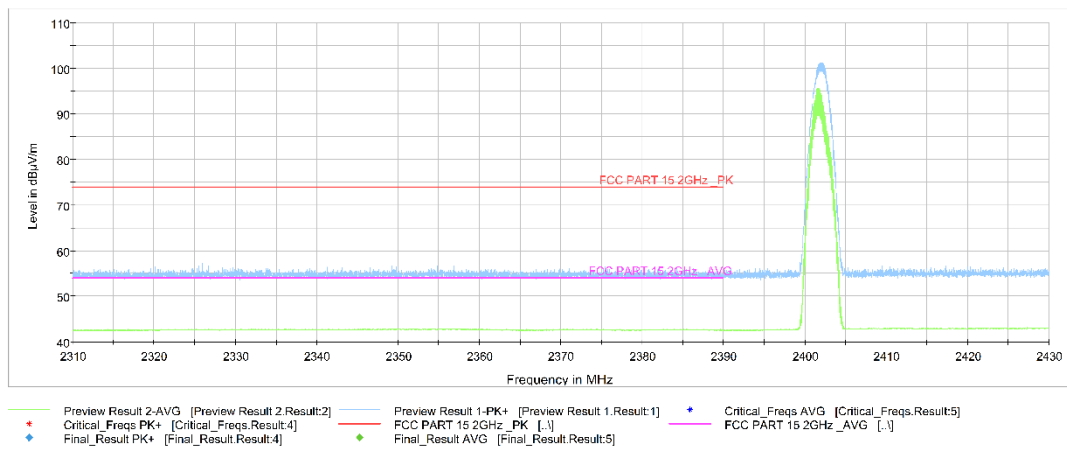
Fig.15. Frequency Band Edges: \pi/4 DQPSK, Channel 0, Hopping Off, 2.31 GHz - 2.43GHz
