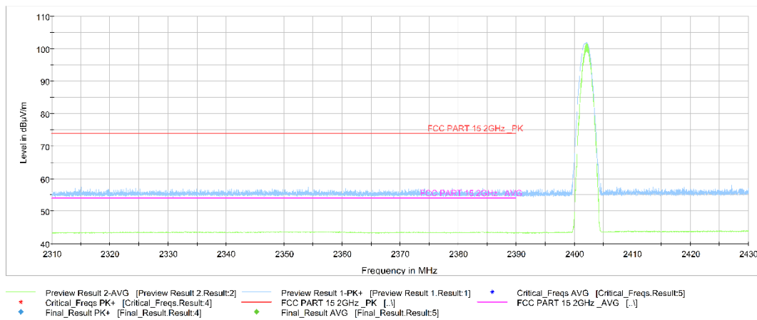
Fig.13. Frequency Band Edges: GFSK, Channel 0, Hopping Off, 2.31 GHz – 2.43GHz
