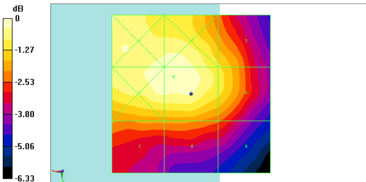
Fig B.3 HAC RF E-Field LTE Band48 16QAM CH55340
