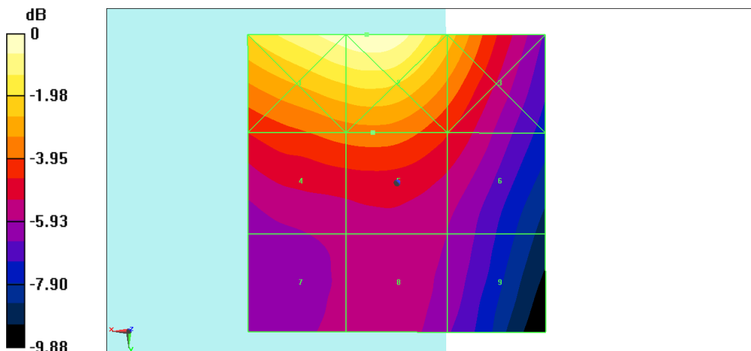
Fig B.1 HAC RF E-Field GSM 850 High
