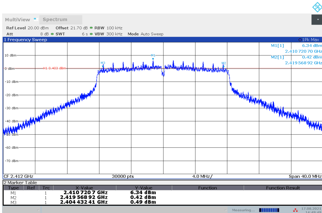
Fig.A.4.4 Occupied 6dB Bandwidth (802.11g, Ch 1)
