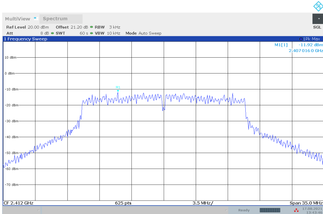
Fig.A.3.7 Power Spectral Density (802.11n-HT20, Ch 1)
