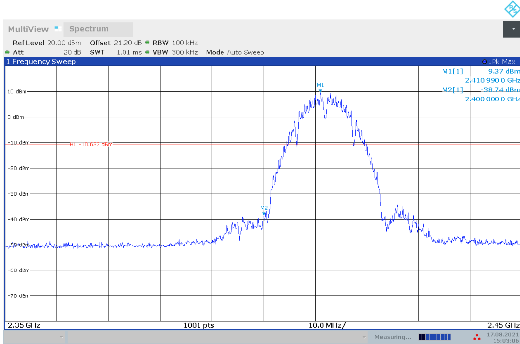
Fig.A.5.1 Band Edges (802.11b, Ch 1)
