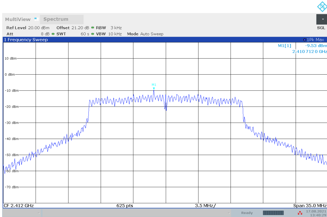
Fig.A.3.4 Power Spectral Density (802.11g, Ch 1)
