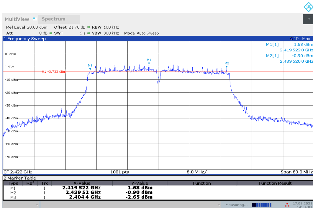
Fig.A.4.10 Occupied 6dB Bandwidth (802.11n-40MHz, Ch 3)
