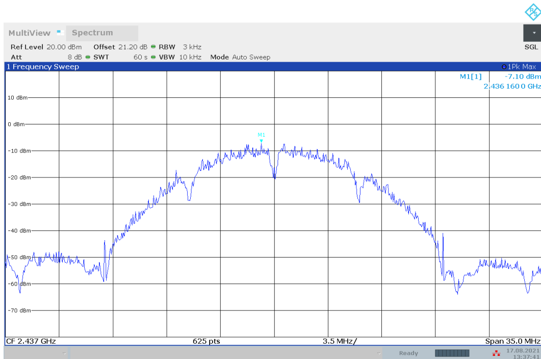
Fig.A.3.2 Power Spectral Density (802.11b, Ch 6)
