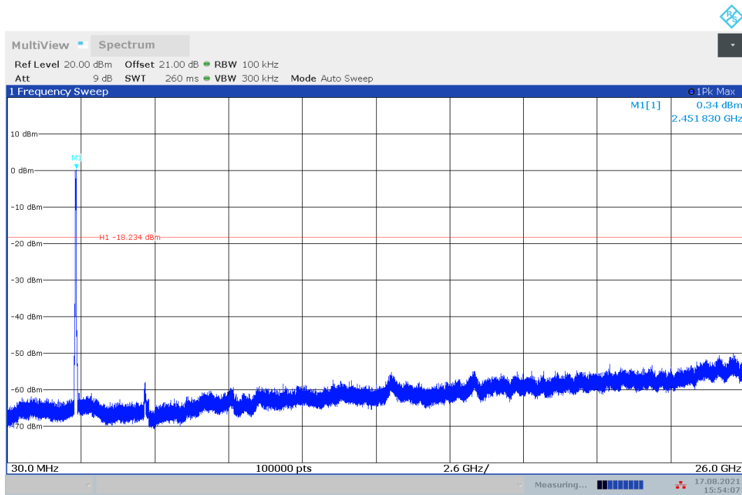
Fig.A.6.1.4 Transmitter Spurious Emission - Conducted (802.11n-HT40, Ch6, 30 MHz-26 GHz)
