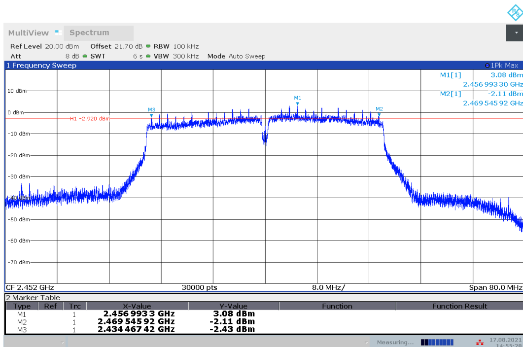
Fig.A.4.12 Occupied 6dB Bandwidth (802.11n-HT40, Ch 9)
