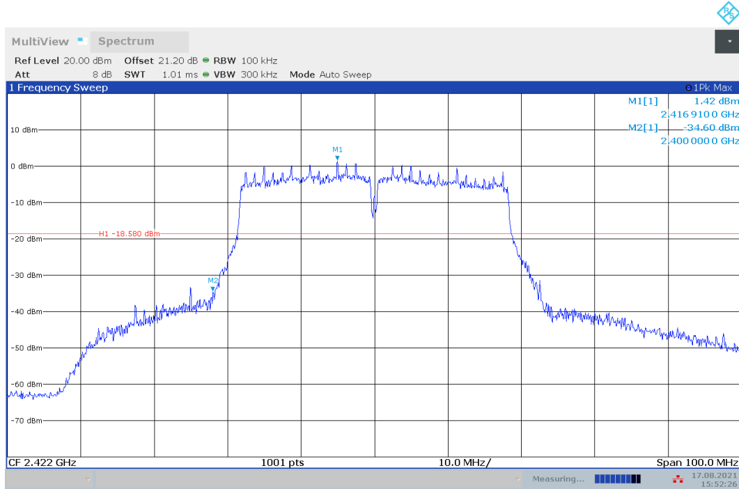
Fig.A.6.1.1 Transmitter Spurious Emission - Conducted (802.11n-HT40, Ch3, Center Frequency)
