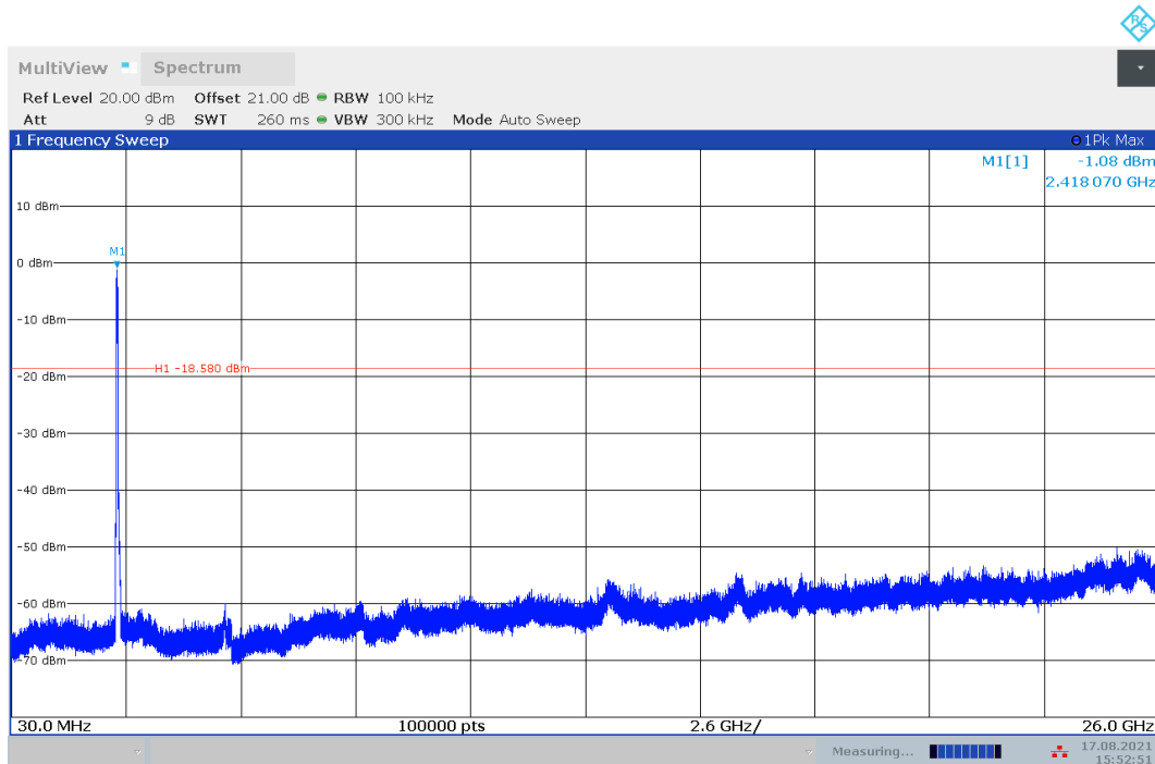
Fig.A.6.1.2 Transmitter Spurious Emission - Conducted (802.11n-HT40, Ch3, 30 MHz-26 GHz)
