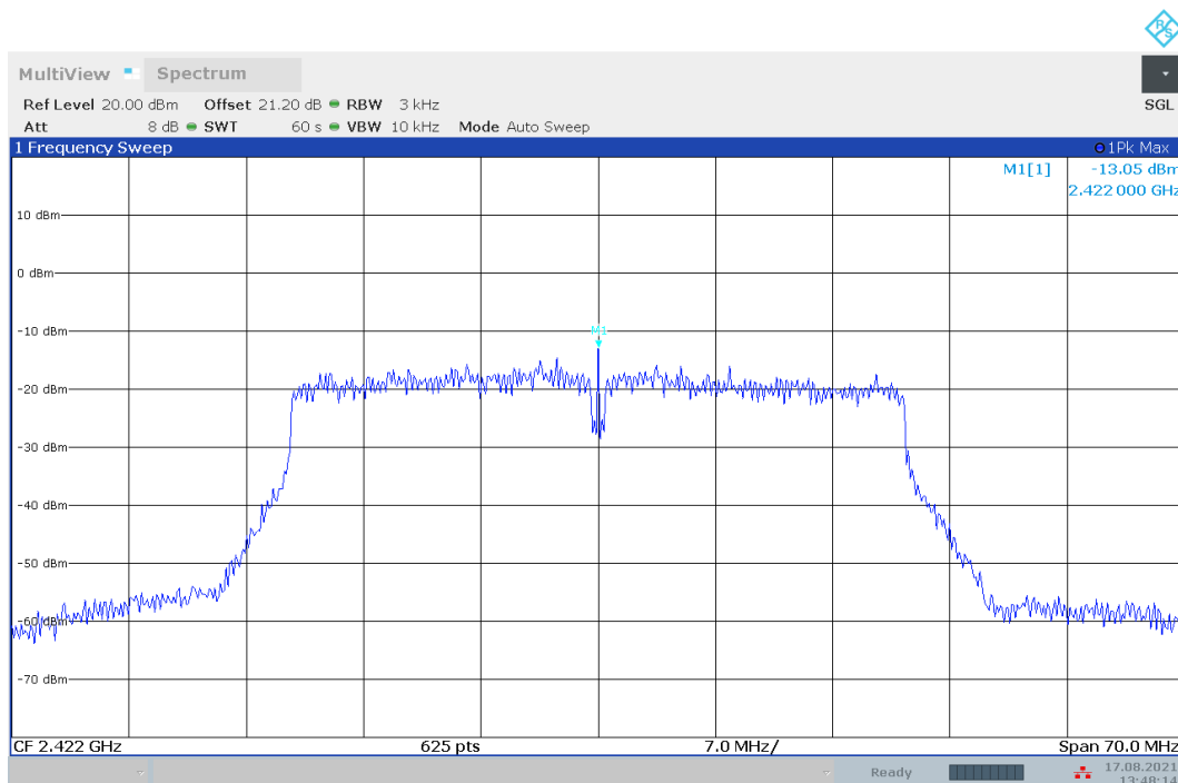
Fig.A.3.10 Power Spectral Density (802.11n-HT40, Ch 3)
