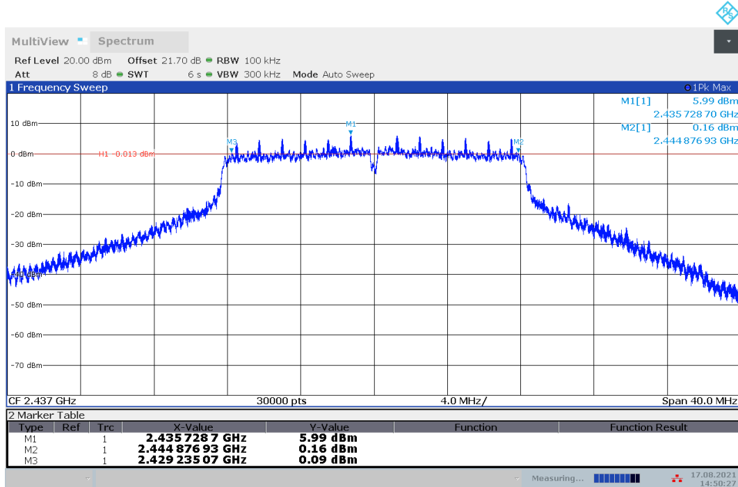
Fig.A.4.5 Occupied 6dB Bandwidth (802.11g, Ch 6)
