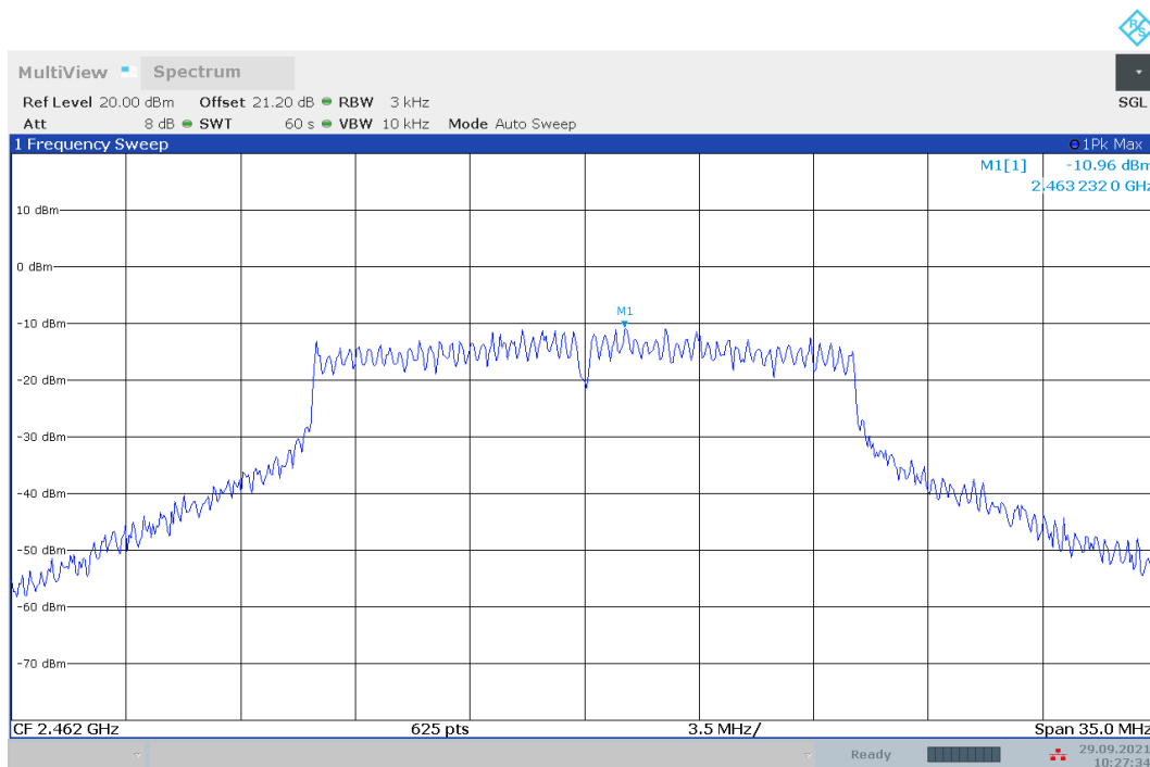
Fig.A.3.6 Power Spectral Density (802.11g, Ch 11)
