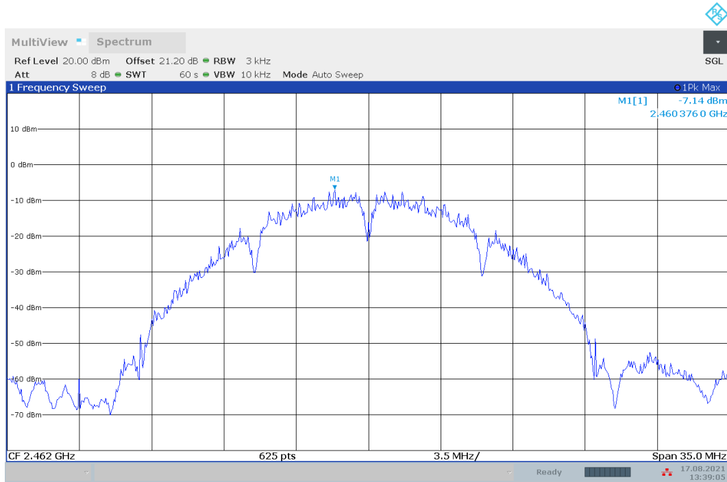
Fig.A.3.3 Power Spectral Density (802.11b, Ch 11)
