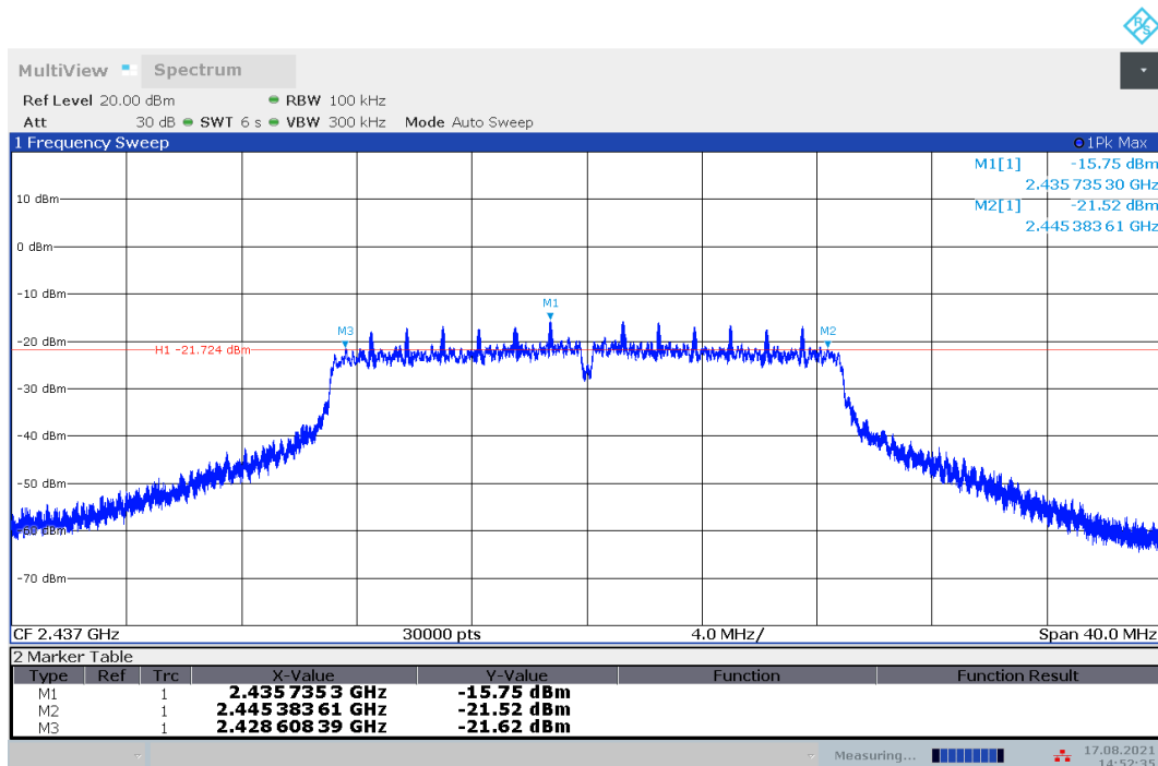
Fig.A.4.8 Occupied 6dB Bandwidth (802.11n-HT20, Ch 6)
