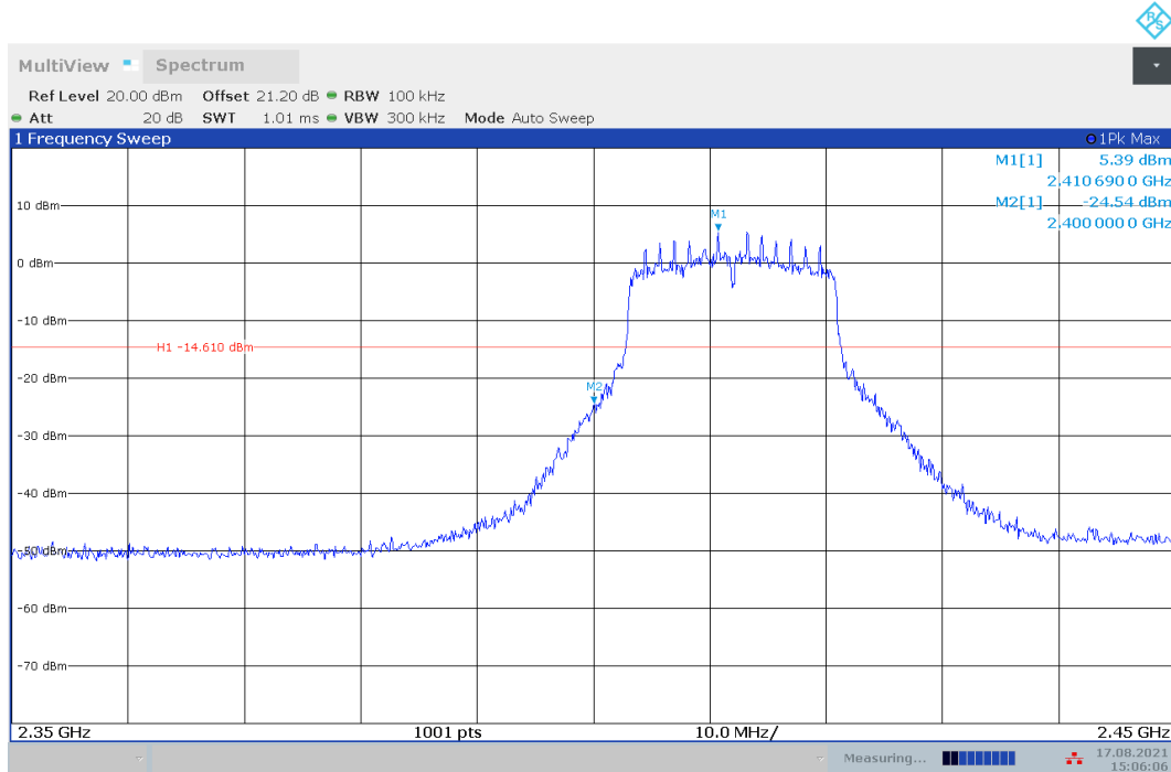
Fig.A.5.5 Band Edges (802.11n-HT20, Ch 1)
