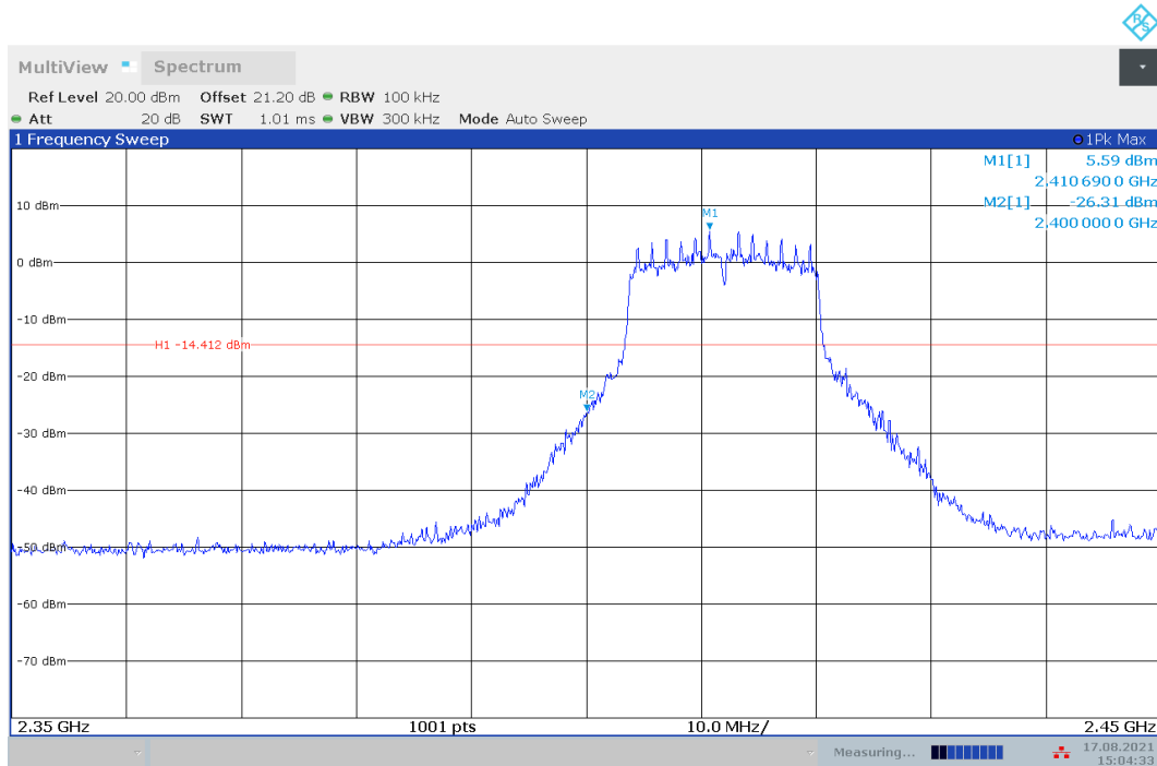
Fig.A.5.3 Band Edges (802.11g, Ch 1)
