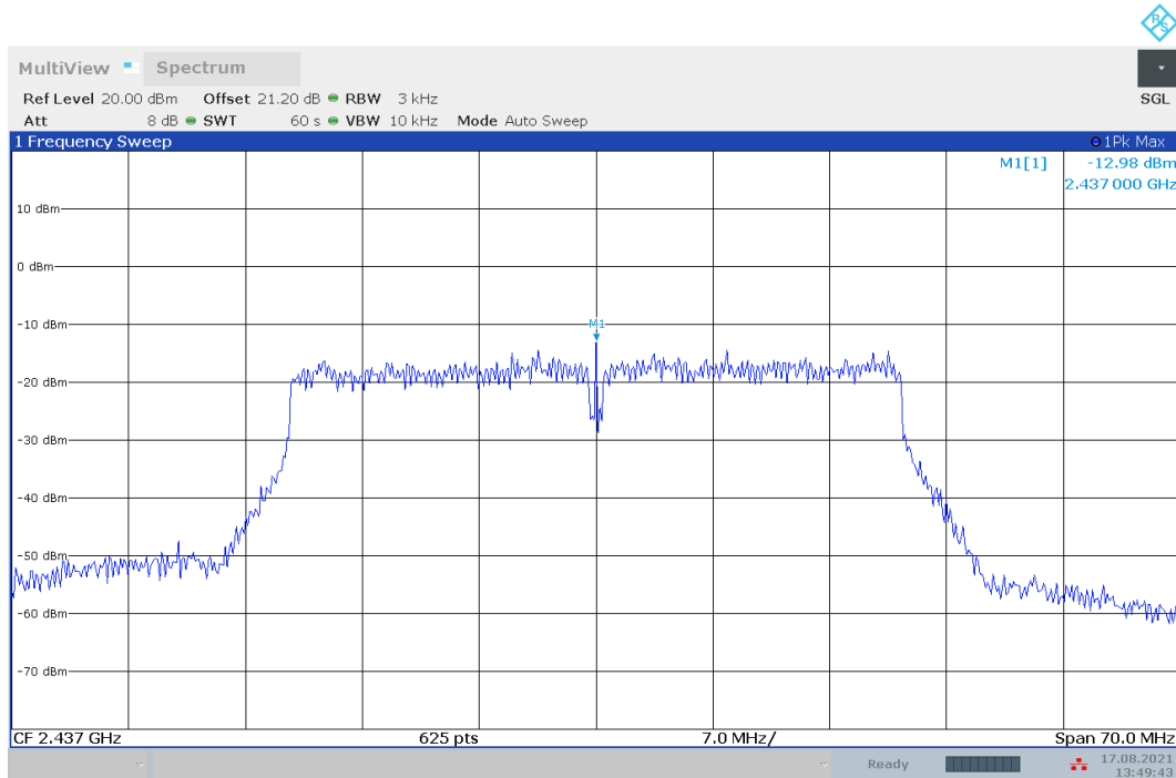
Fig.A.3.11 Power Spectral Density (802.11n-HT40, Ch 6)
