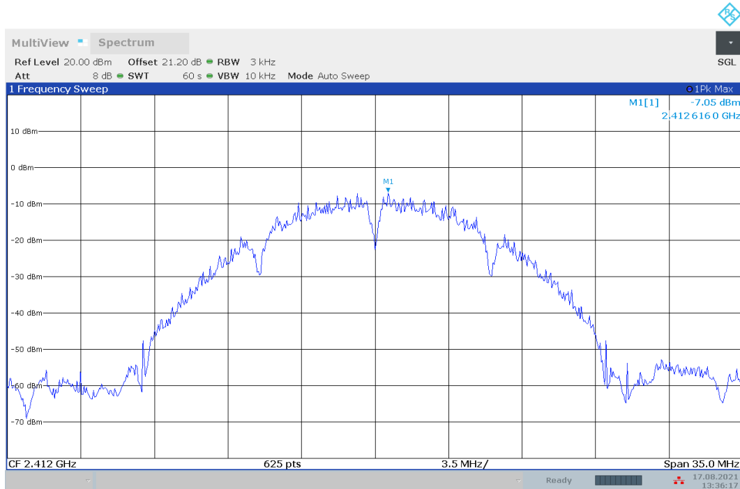
Fig.A.3.1 Power Spectral Density(802.11b,Ch1)
