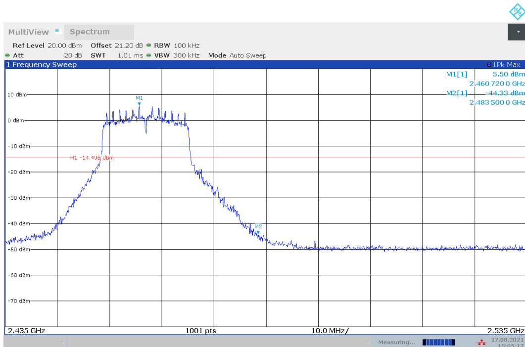
Fig.A.5.6 Band Edges (802.11n-HT20, Ch 11)
