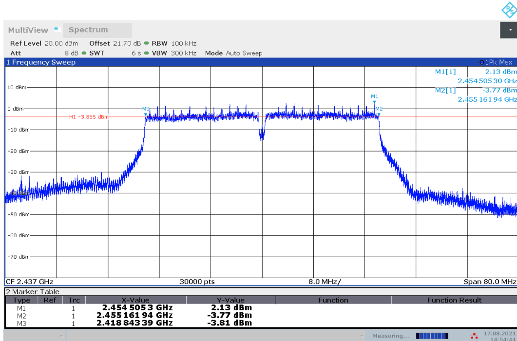
Fig.A.4.11 Occupied 6dB Bandwidth (802.11n-HT40, Ch 6)
