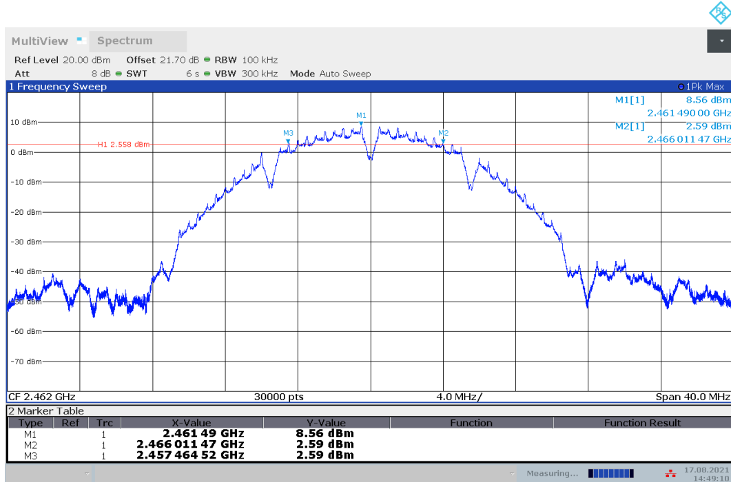
Fig.A.4.3 Occupied 6dB Bandwidth (802.11b, Ch 11)
