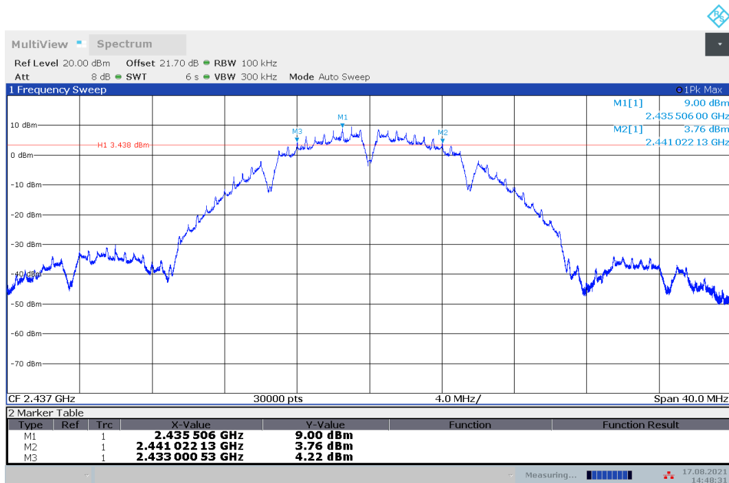
Fig.A.4.2 Occupied 6dB Bandwidth (802.11b, Ch 6)
