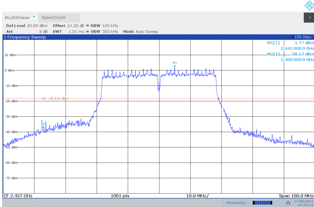
Fig.A.6.1.3 Transmitter Spurious Emission - Conducted (802.11n-HT40, Ch6, Center Frequency)
