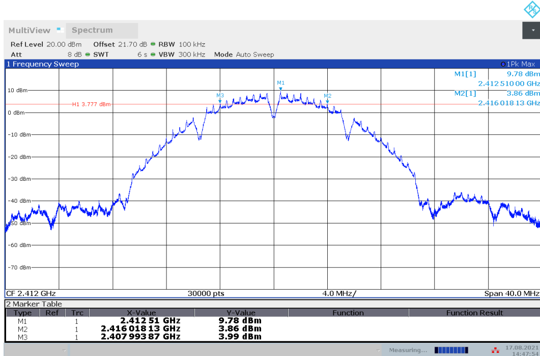
Fig.A.4.1 Occupied 6dB Bandwidth(802.11b,Ch 1)
