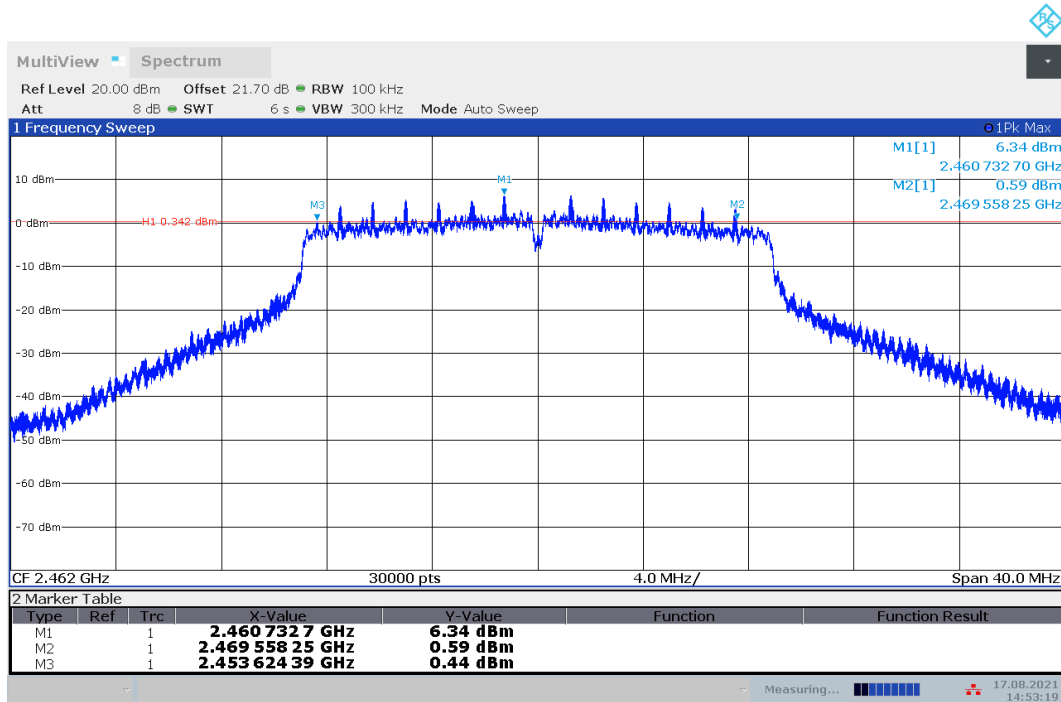
Fig.A.4.9 Occupied 6dB Bandwidth (802.11n-HT20, Ch 11)
