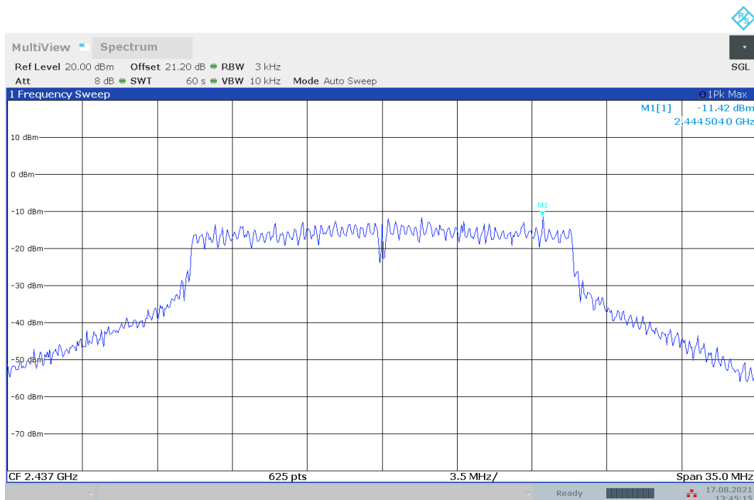
Fig.A.3.8 Power Spectral Density (802.11n-HT20, Ch 6)
