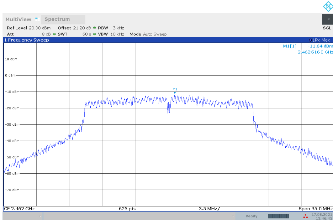
Fig.A.3.9 Power Spectral Density (802.11n-HT20, Ch 11)
