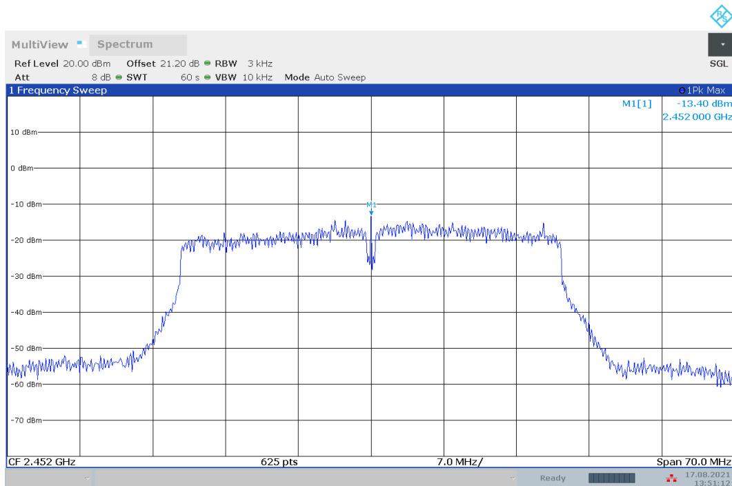
Fig.A.3.12 Power Spectral Density (802.11n-HT40, Ch 9)
