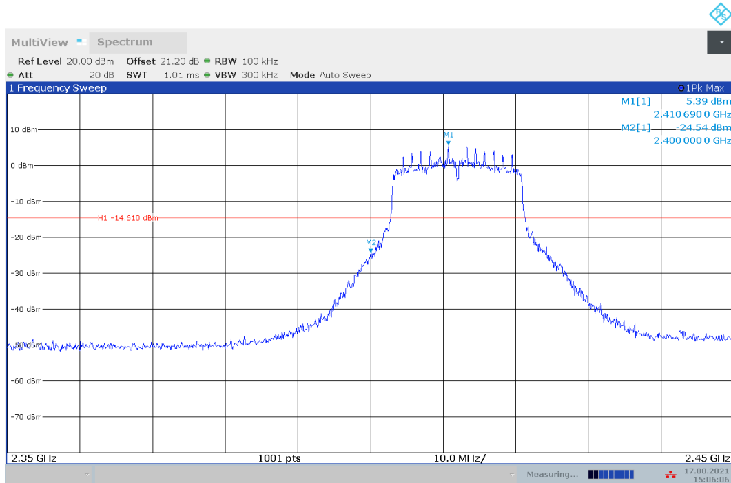
Fig.A.5.7 Band Edges (802.11n-HT40, Ch 3)
