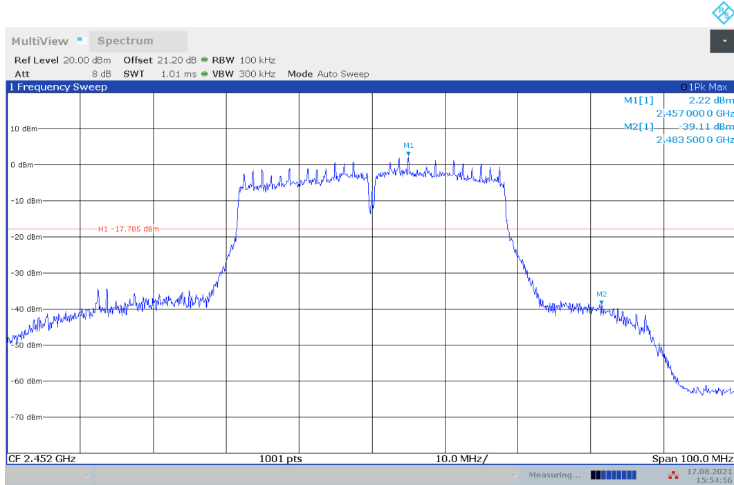
Fig.A.6.1.5 Transmitter Spurious Emission - Conducted (802.11n-HT40, Ch9, Center Frequency)
