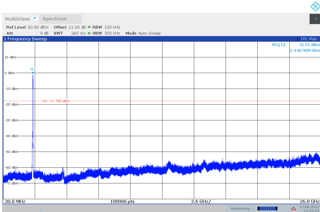
Fig.A.6.1.6 Transmitter Spurious Emission - Conducted (802.11n-HT40, Ch9, 30 MHz-26 GHz)
