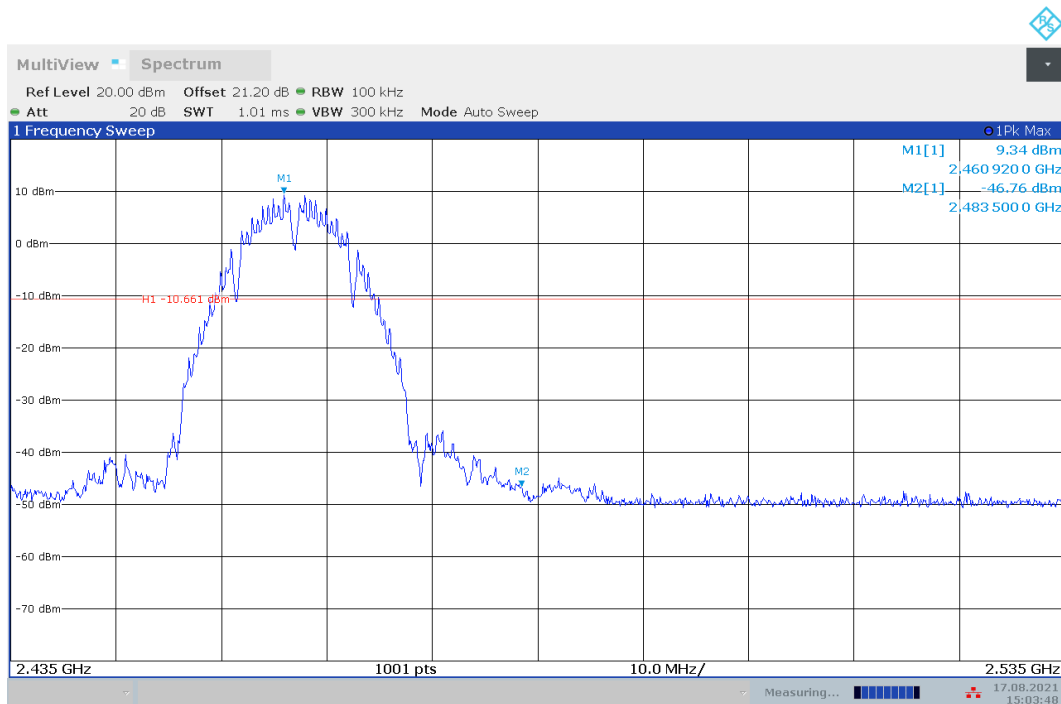
Fig.A.5.2 Band Edges (802.11b, Ch 11)
