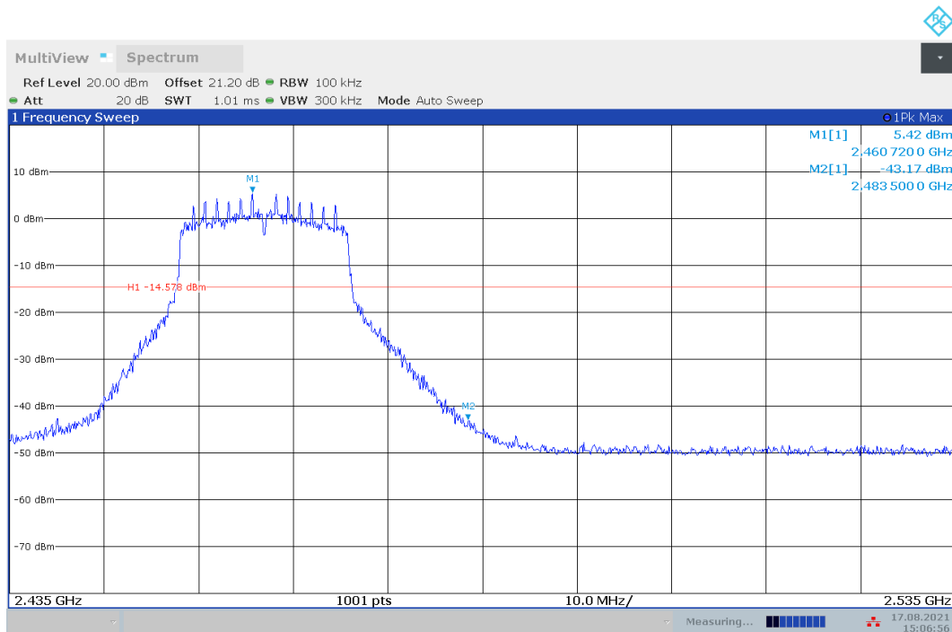
Fig.A.5.8 Band Edges (802.11n-HT40, Ch 9)
