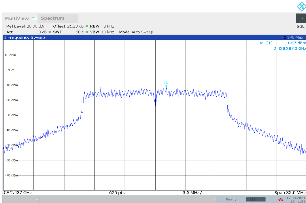
Fig.A.3.5 Power Spectral Density (802.11g, Ch 6)
