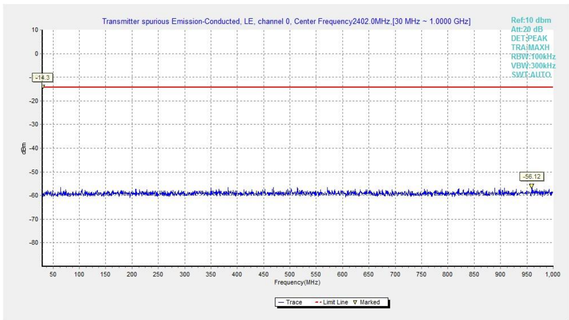
Fig.12. Transmitter Spurious Emission - Conducted: GFSK, 2402 MHz, 30MHz - 1GHz
