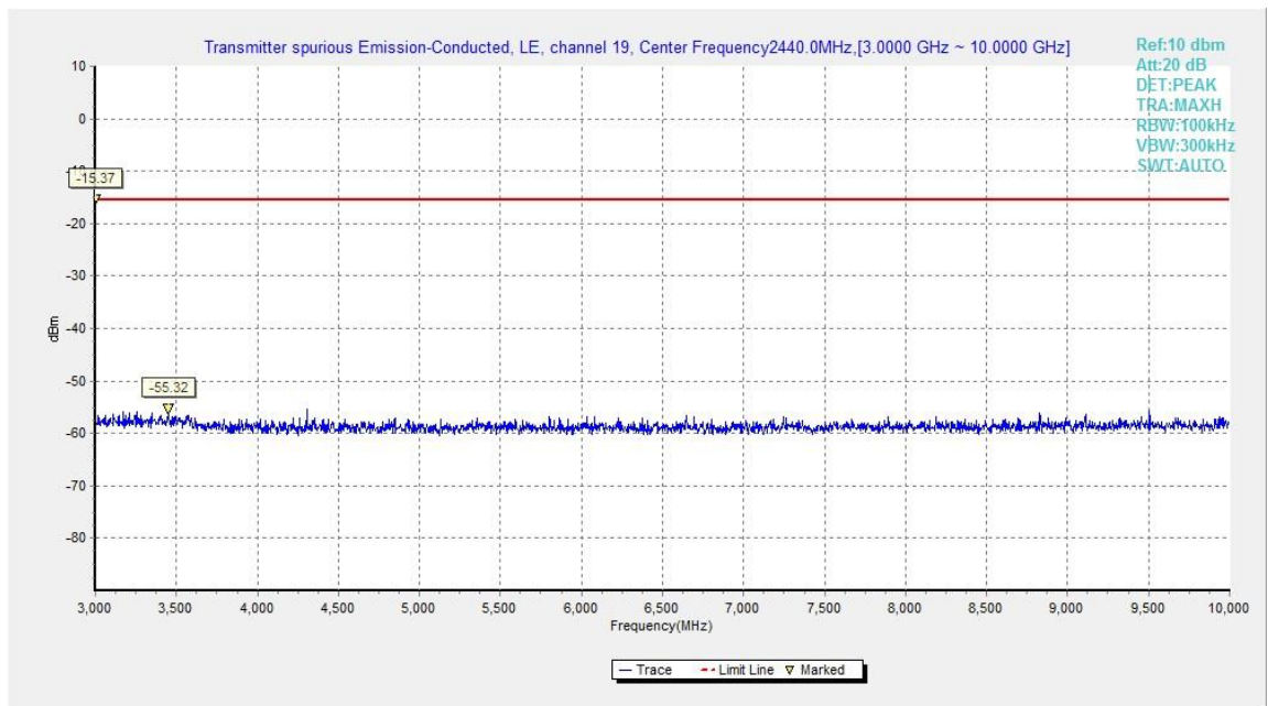
Fig.19. Transmitter Spurious Emission - Conducted: GFSK, 2440 MHz, 3GHz – 10GHz
