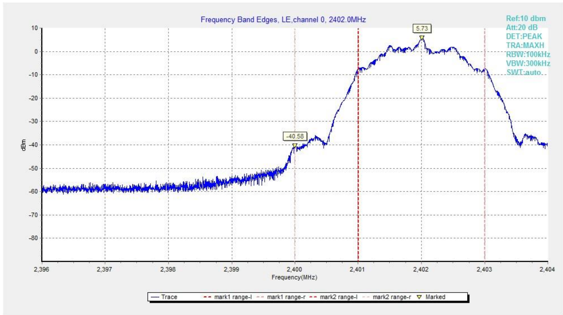
Fig.7. Frequency Band Edges: GFSK, 2402 MHz, Hopping Off
