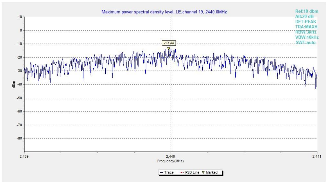
Fig.30. Maximum Power Spectral Density Level Function: GFSK, 2440 MHz
