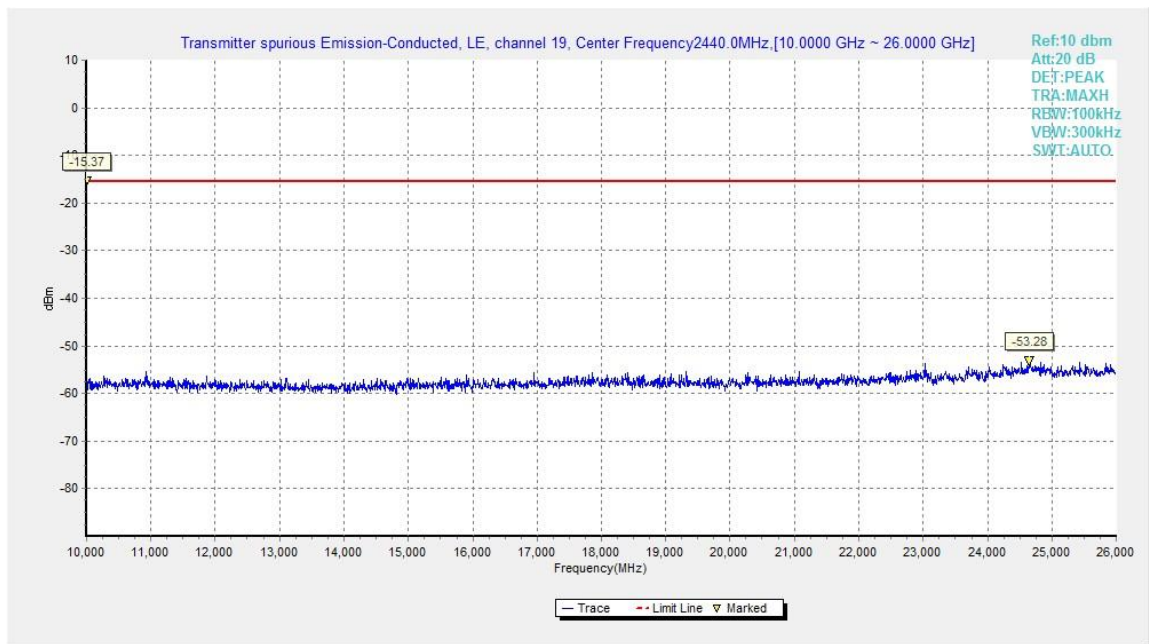
Fig.20. Transmitter Spurious Emission - Conducted: GFSK, 2440 MHz, 10GHz – 26GHz
