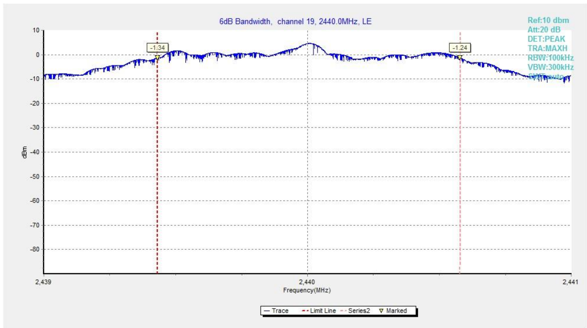
Fig.27. 6dB Bandwidth: GFSK, 2440 MHz
