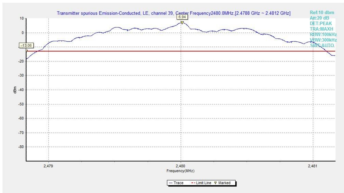
Fig.21. Transmitter Spurious Emission - Conducted: GFSK, 2480 MHz
