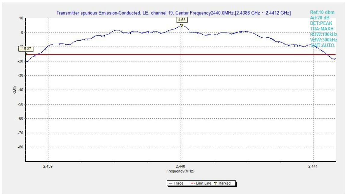
Fig.16. Transmitter Spurious Emission - Conducted: GFSK, 2440MHz
