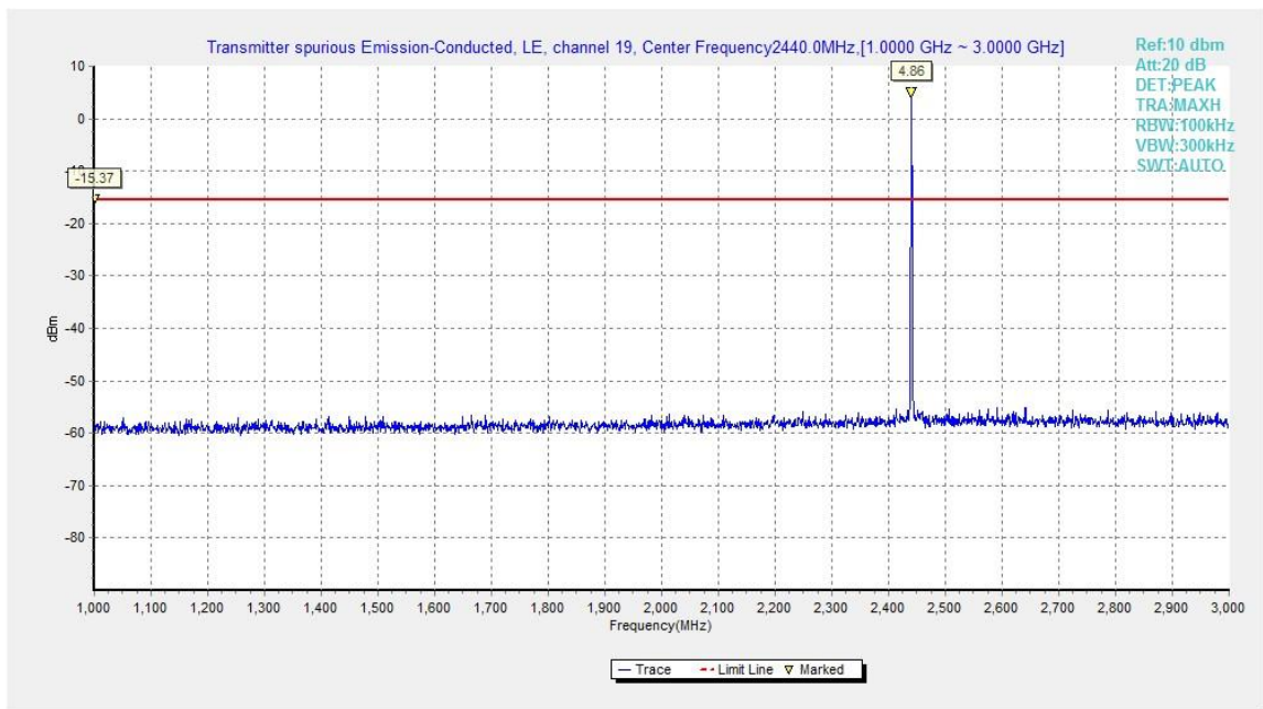
Fig.18. Transmitter Spurious Emission - Conducted: GFSK, 2440 MHz, 1GHz – 3GHz
