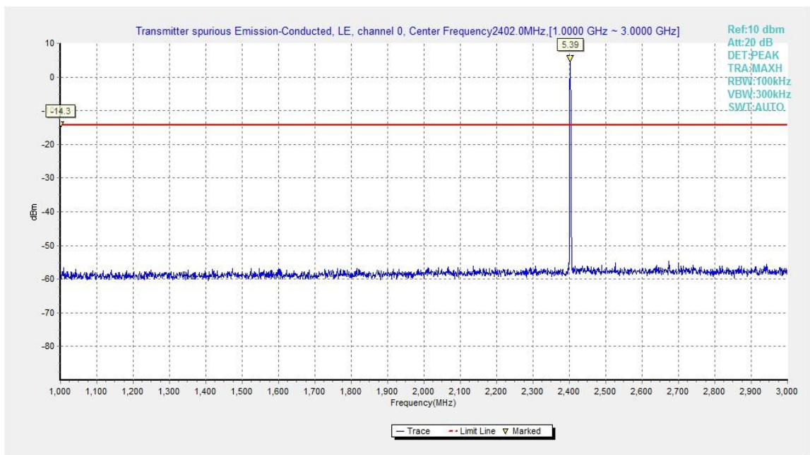
Fig.13. Transmitter Spurious Emission - Conducted: GFSK, 2402 MHz, 1GHz - 3GHz
