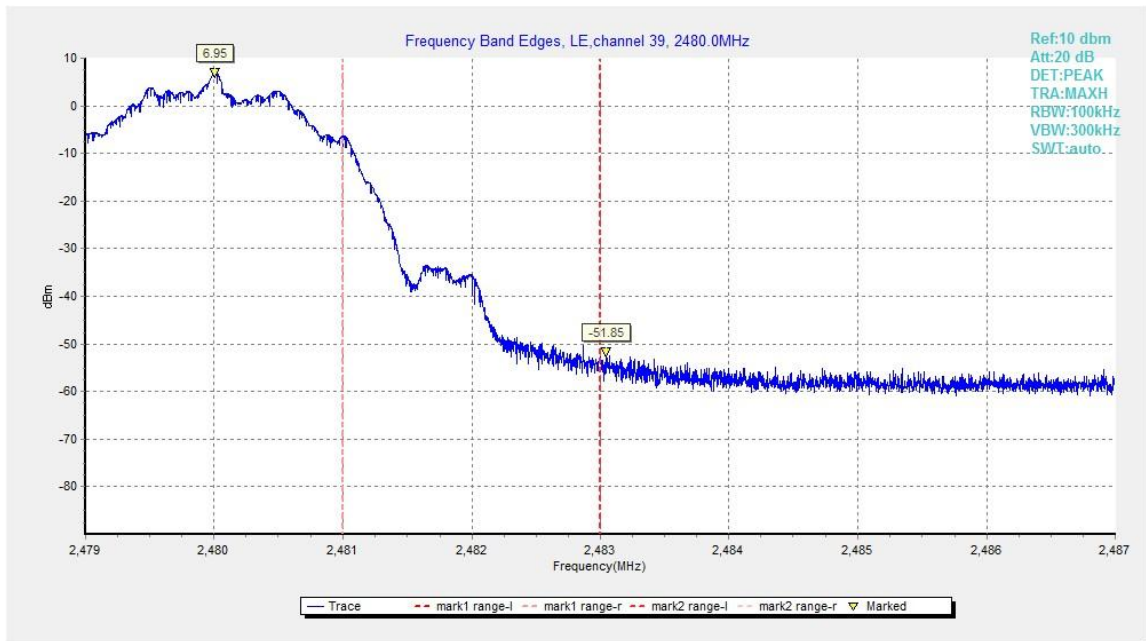
Fig.8. Frequency Band Edges: GFSK, 2480 MHz, Hopping Off
