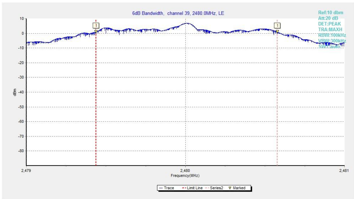
Fig.28. 6dB Bandwidth: GFSK, 2480 MHz
