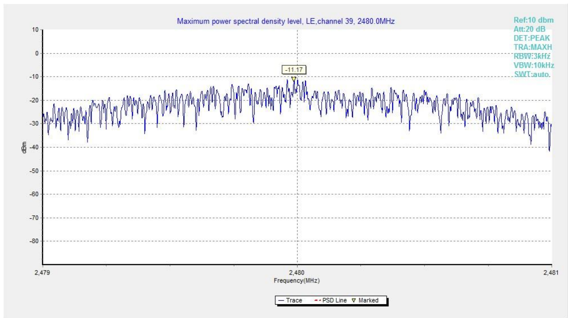
Fig.31. Maximum Power Spectral Density Level Function: GFSK, 2480 MHz
