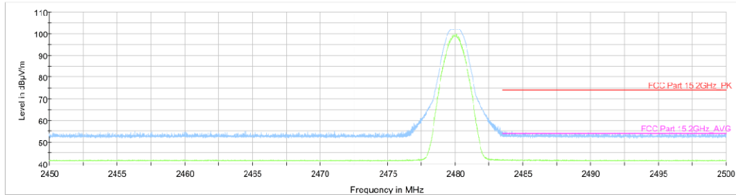
Fig.10. Frequency Band Edges: GFSK, 2480 MHz, Hopping Off , 2.45 GHz - 2.50GHz
