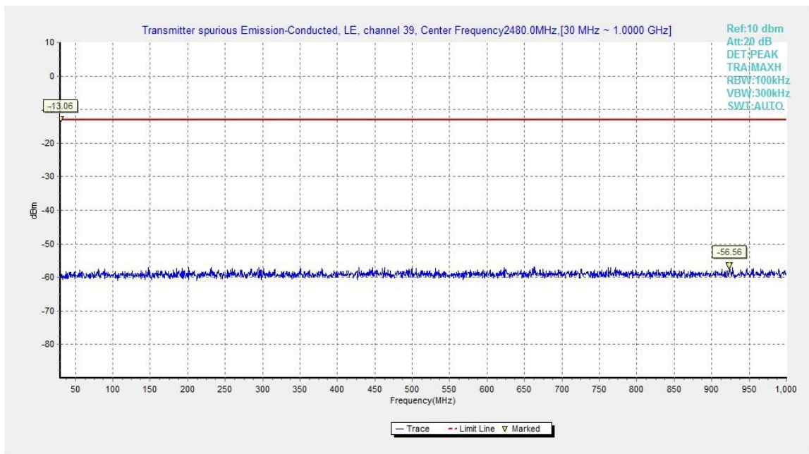
Fig.22. Transmitter Spurious Emission - Conducted: GFSK, 2480 MHz, 30MHz - 1GHz
