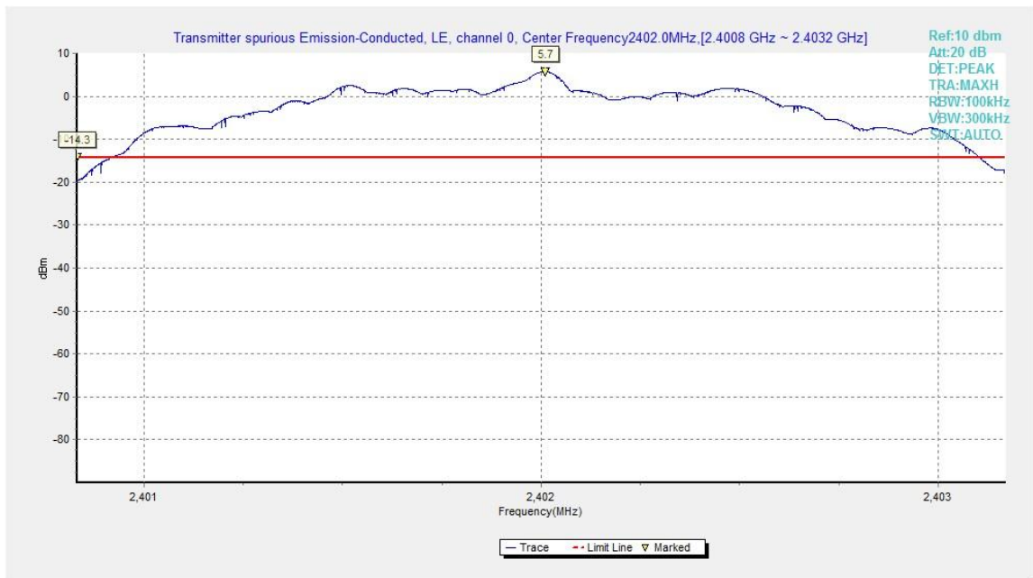
Fig.11. Transmitter Spurious Emission - Conducted: GFSK,2402MHz
