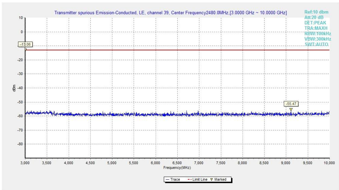
Fig.24. Transmitter Spurious Emission - Conducted: GFSK, 2480 MHz, 3GHz - 10GHz
