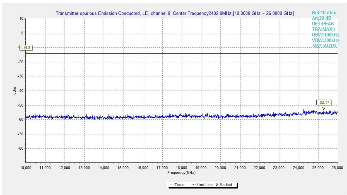
Fig.15. Transmitter Spurious Emission - Conducted: GFSK, 2402 MHz, 10GHz - 26GHz
