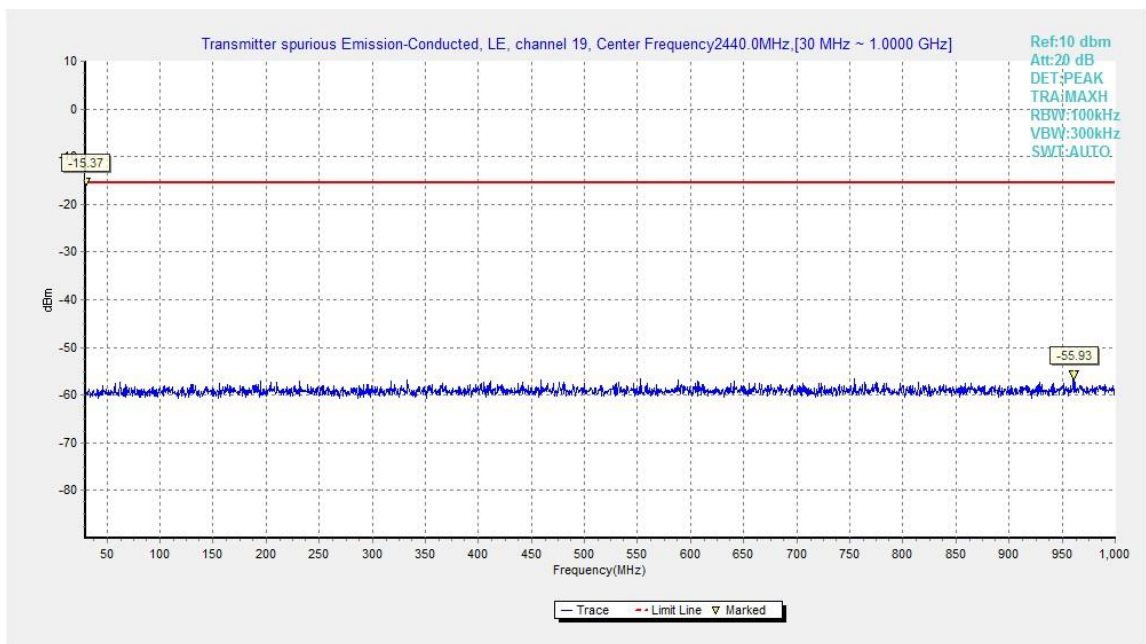
Fig.17. Transmitter Spurious Emission - Conducted: GFSK, 2440 MHz, 30MHz - 1GHz
