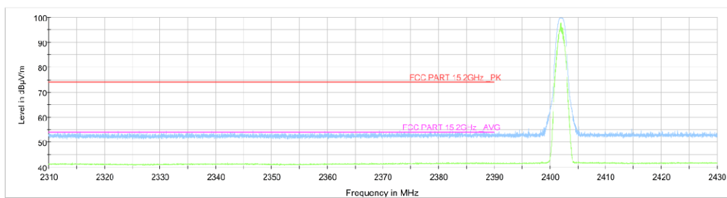
Fig.9. Frequency Band Edges: GFSK, 2402 MHz, Hopping Off, 2.31 GHz – 2.43GHz
