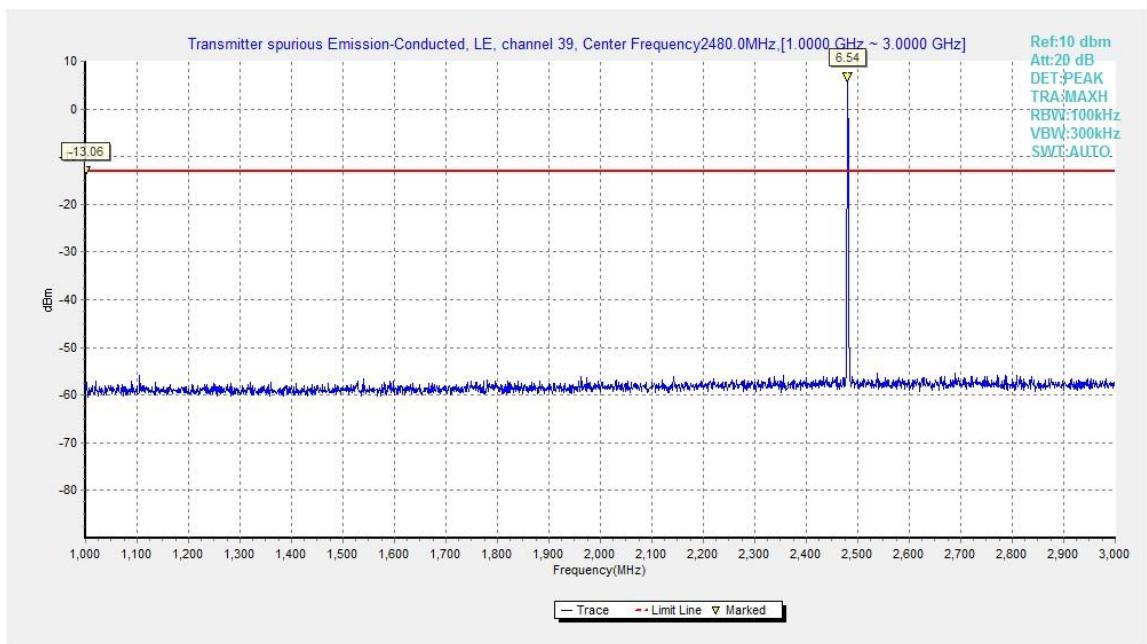
Fig.23. Transmitter Spurious Emission - Conducted: GFSK, 2480 MHz, 1GHz - 3GHz
