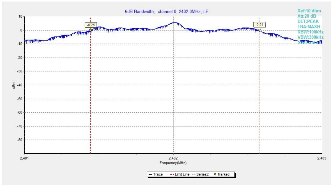
Fig.26. 6dB Bandwidth: GFSK, 2402 MHz
