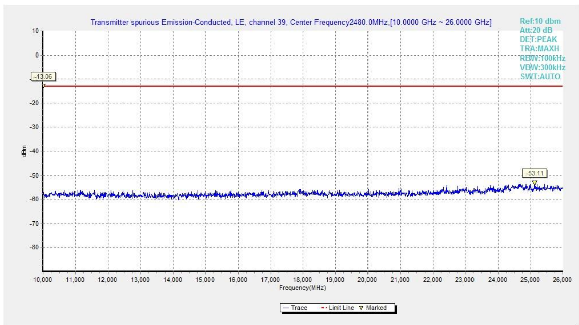
Fig.25. Transmitter Spurious Emission - Conducted: GFSK, 2480 MHz, 10GHz - 26GHz
