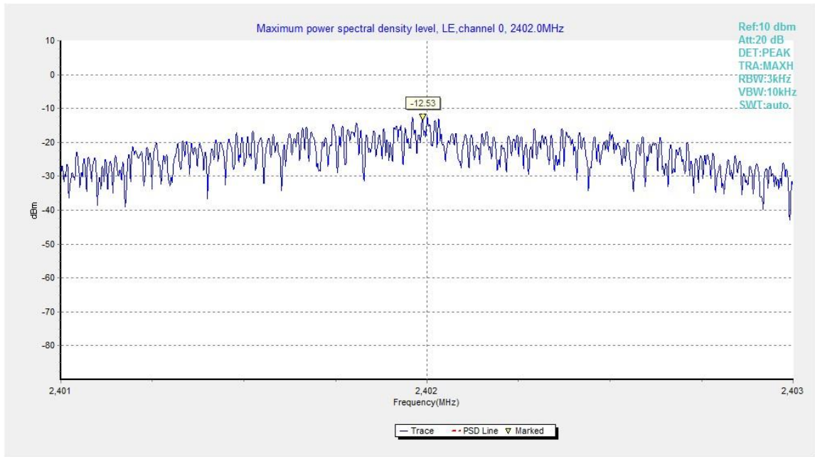
Fig.29. Maximum Power Spectral Density Level Function: GFSK, 2402 MHz
