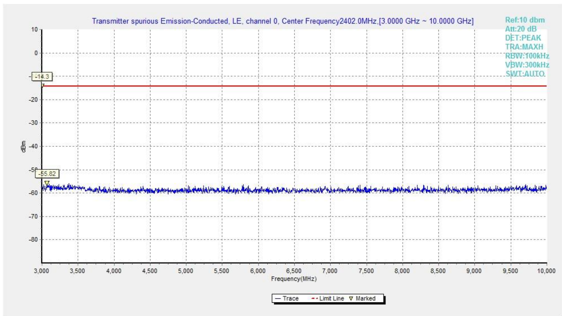
Fig.14. Transmitter Spurious Emission - Conducted: GFSK, 2402 MHz, 3GHz - 10GHz
