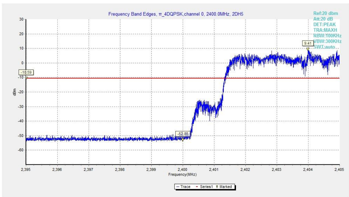
Fig.15. Frequency Band Edges: \pi/4 DQPSK, Channel 0, Hopping On
