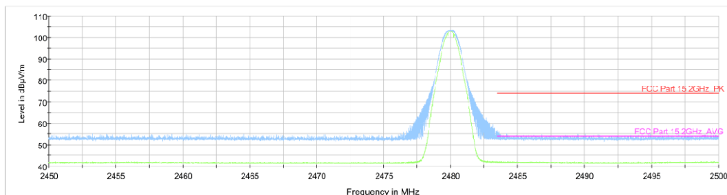
Fig.23. Frequency Band Edges: GFSK, Channel 78, Hopping Off, ch11, 2.45 GHz - 2.50GHz
