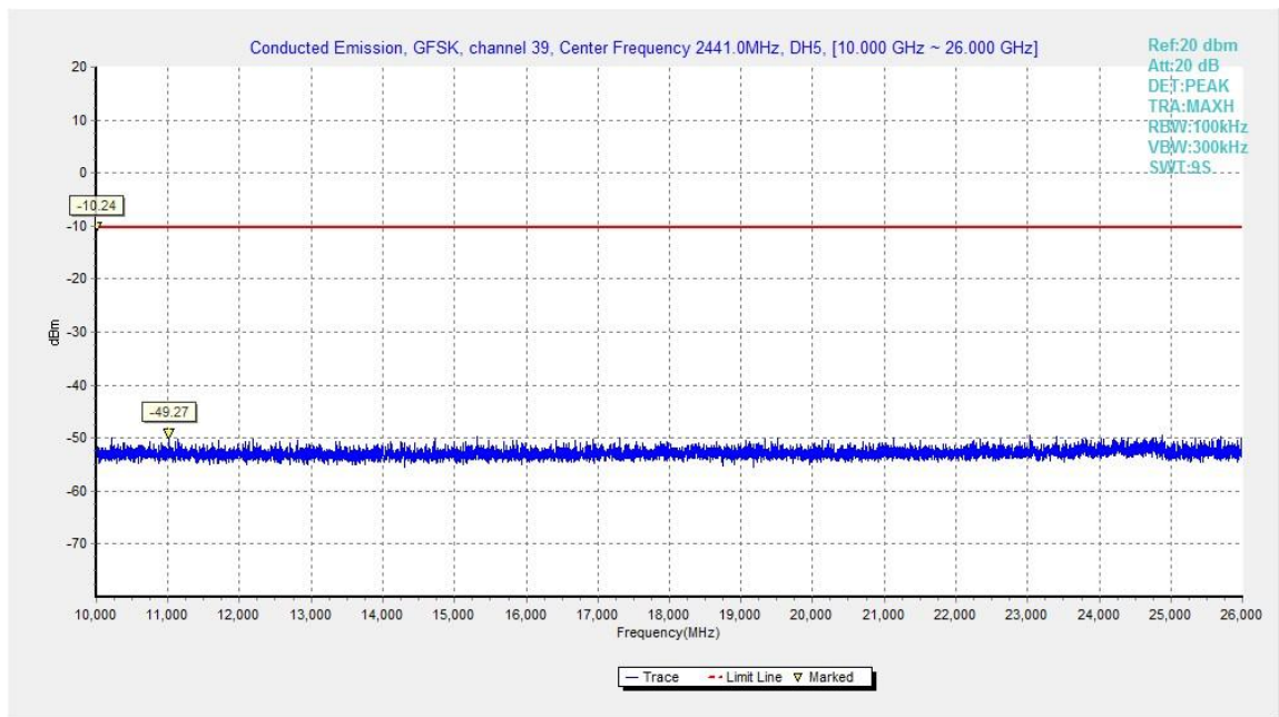
Fig.37. Conducted spurious emission: GFSK, Channel 39, 10GHz – 26GHz
