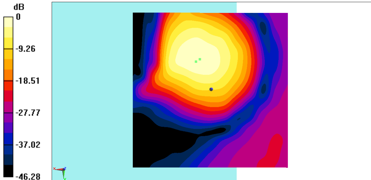
Fig B.4 T-Coil WIF12.4G
