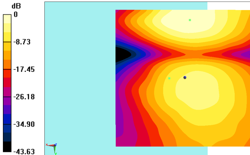
Fig B.1 T-Coil LTEBand41
