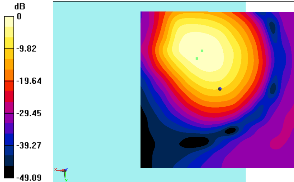
Fig B.2 T-Coil LTEB41
