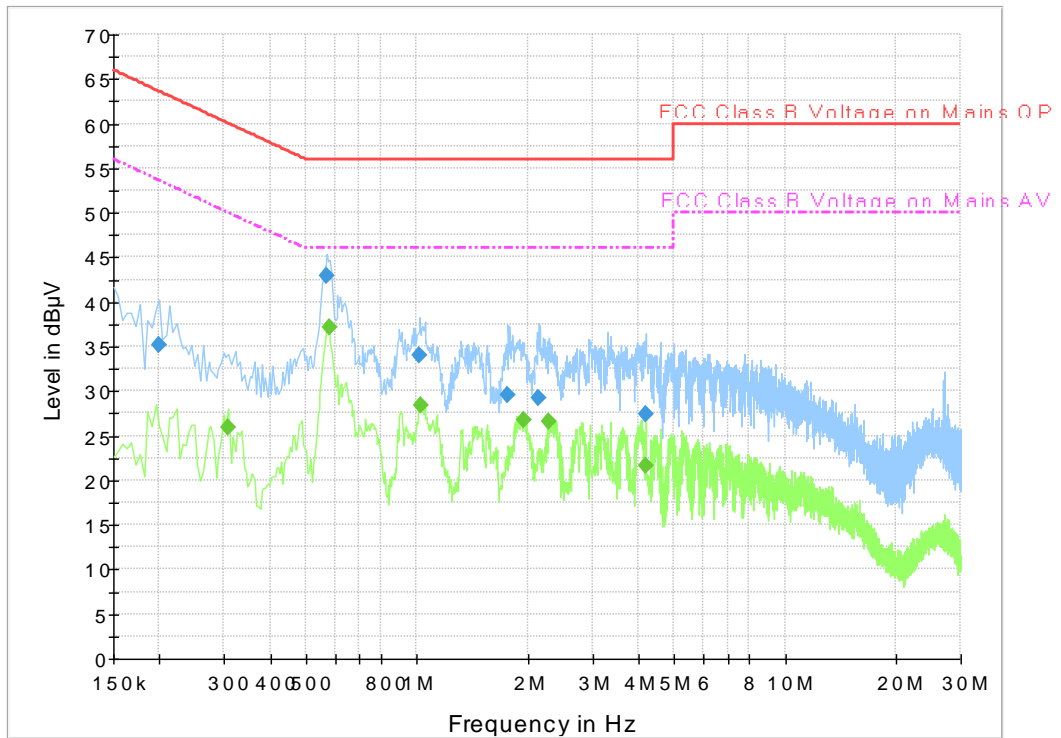
Fig. 22 AC Power line Conducted Emission-802.11a
