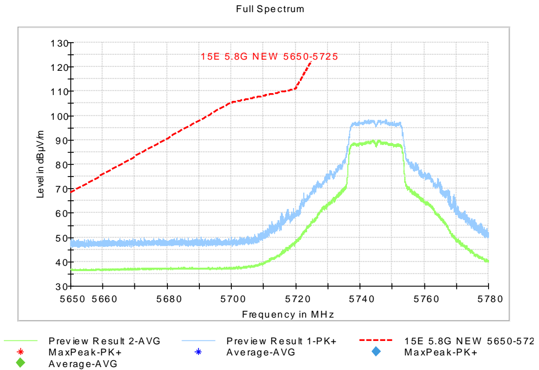
Fig. 10 Band Edges (802.11a Ch149, 5745MHz)
