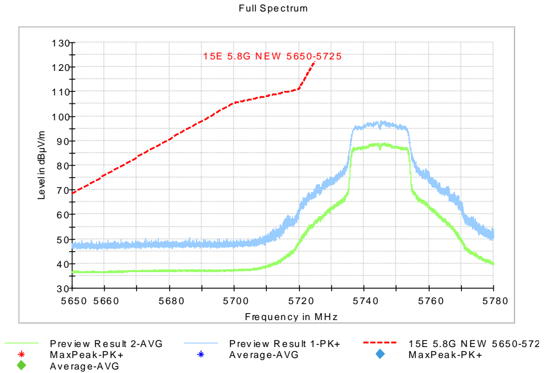
Fig. 12 Band Edges (802.11n-HT20 Ch149, 5745MHz)
