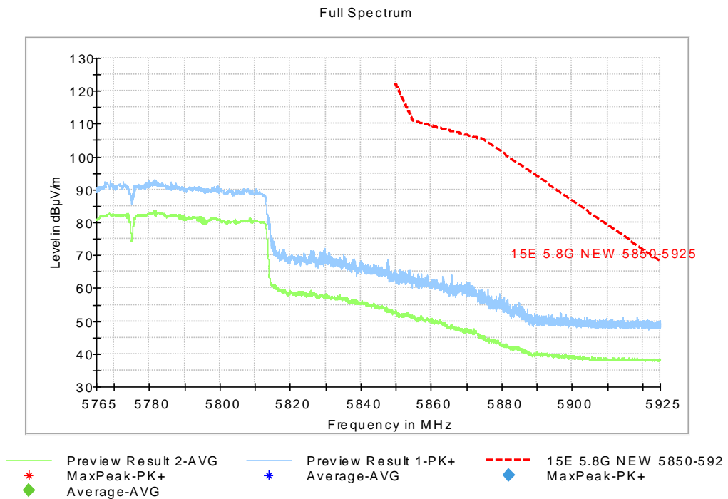
Fig. 21 Band Edges (802.11ac-HT80 Ch155, 5775MHz)
