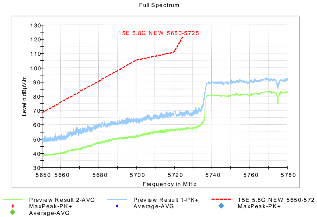
Fig. 20 Band Edges (802.11ac-HT80 Ch155, 5775MHz)
