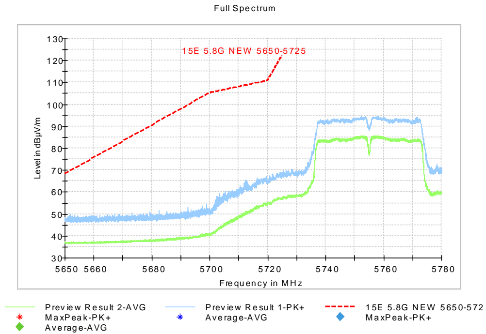
Fig. 18 Band Edges (802.11ac-HT40 Ch151, 5755MHz)
