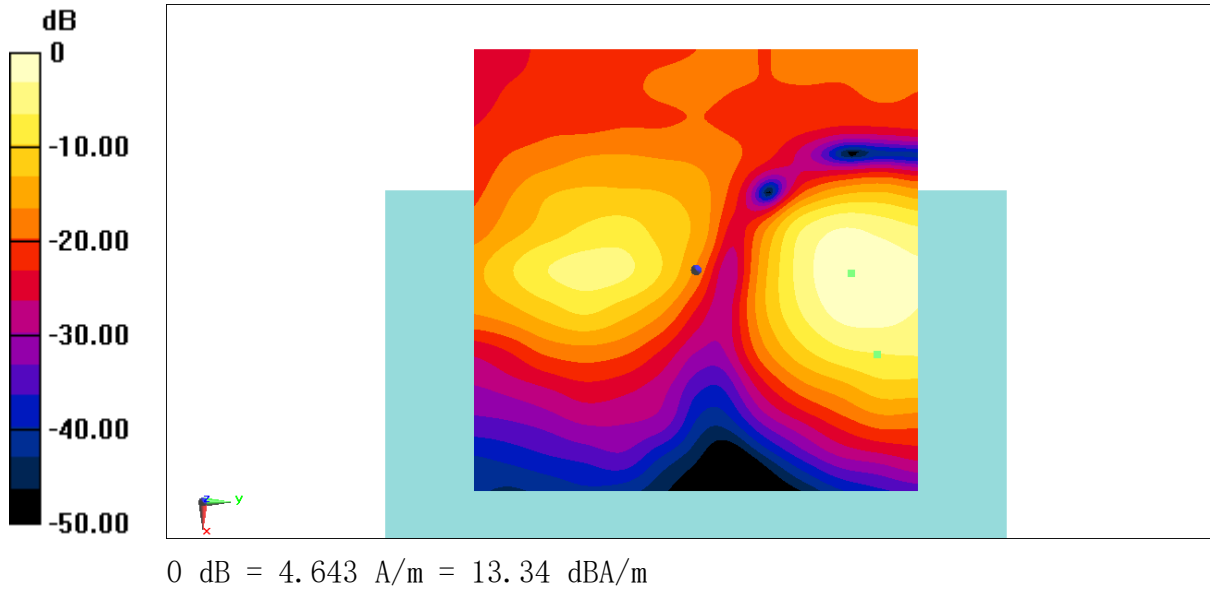
Fig B.14 T-Coil WiFi-2.4G
