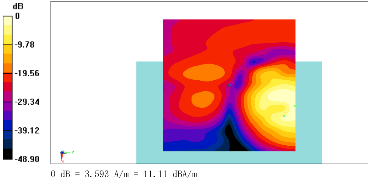
Fig B.16 T-Coil WiFi-5G
