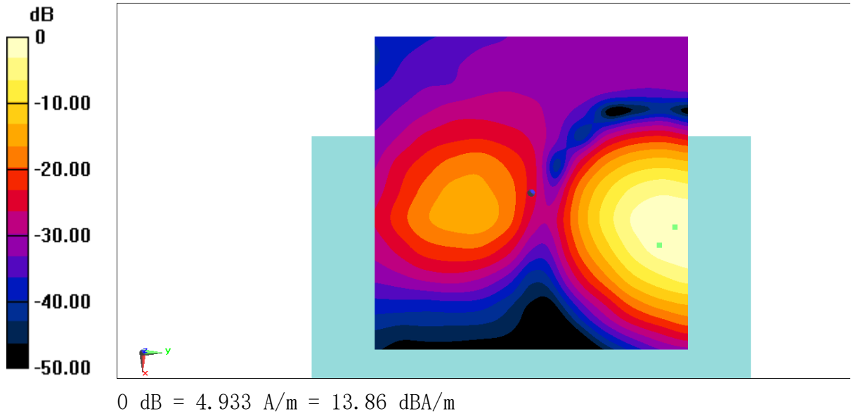
Fig B.4 T-Coil LTE B12
