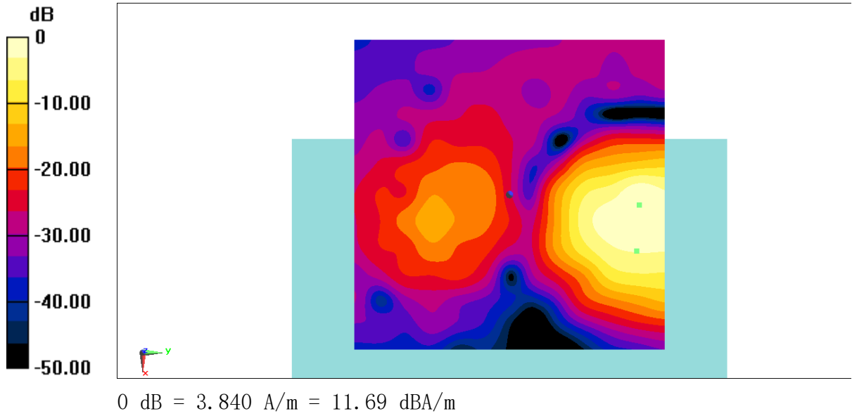
Fig B.6 T-Coil WiFi-2.4G
