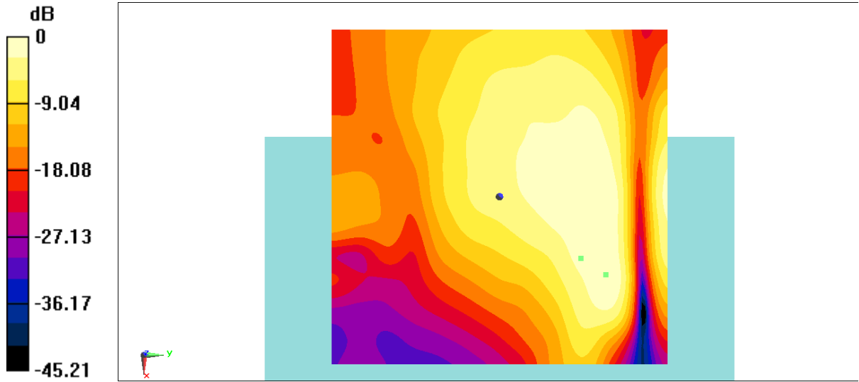
Fig B.13 T-Coil WiFi-2.4G
