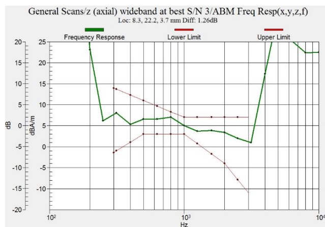
Figure C.6 Frequency Response of LTE B66 - OTT VoIP
