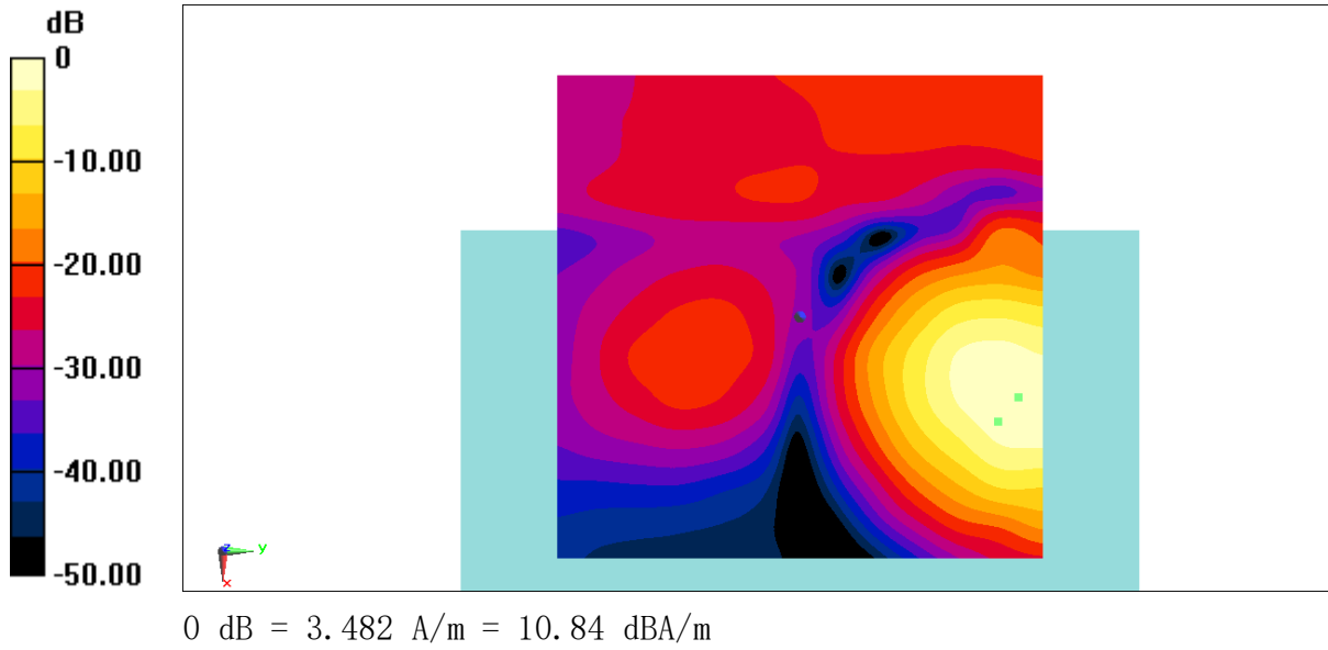
Fig B.12 T-Coil LTE B66
