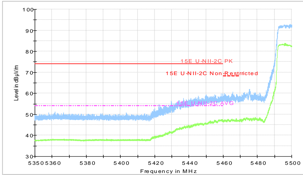
Fig.52 Band Edges (802.11ac-HT80, 5530MHz)
