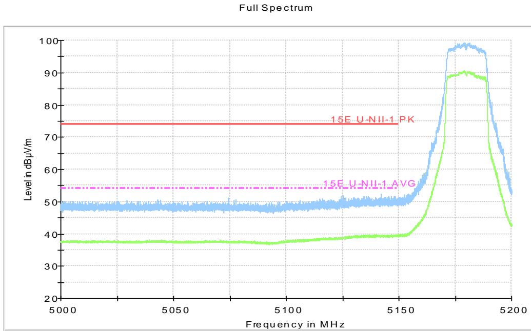
Fig.42 Band Edges (802.11ac-HT20, 5180MHz)
