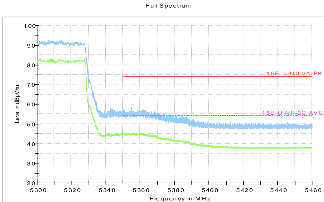
Fig.51 Band Edges (802.11ac-HT80, 5290MHz)
