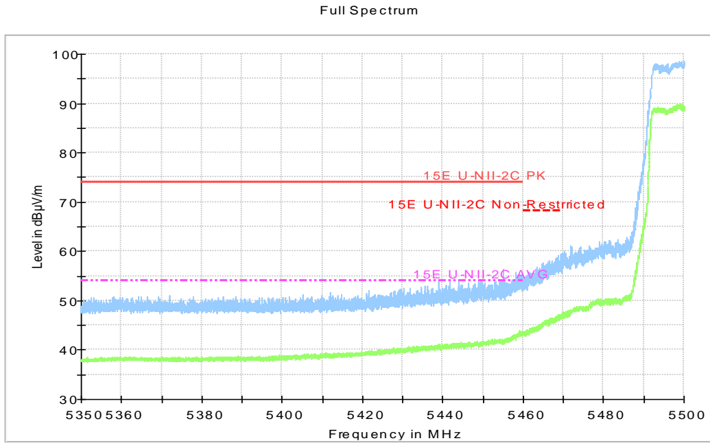
Fig.40 Band Edges (802.11n-HT40, 5510MHz)
