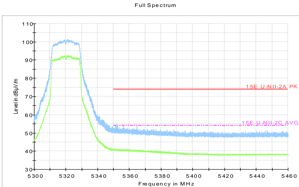
Fig.43 Band Edges (802.11ac-HT20, 5320MHz)
