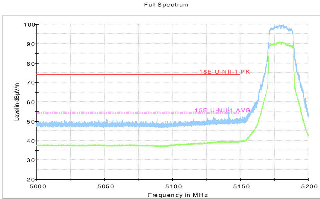
Fig.34 Band Edges (802.11n-HT20, 5180MHz)
