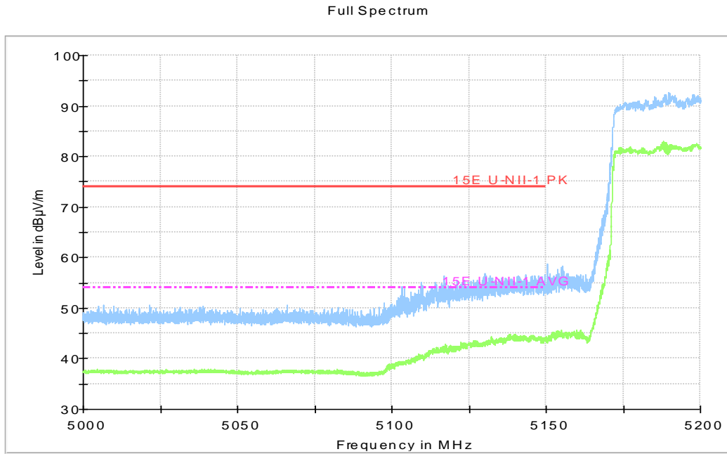
Fig.50 Band Edges (802.11ac-HT80, 5210MHz)
