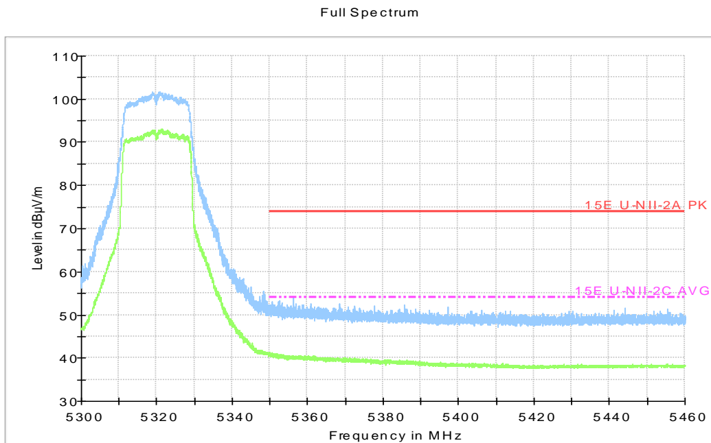
Fig.35 Band Edges (802.11n-HT20, 5320MHz)
