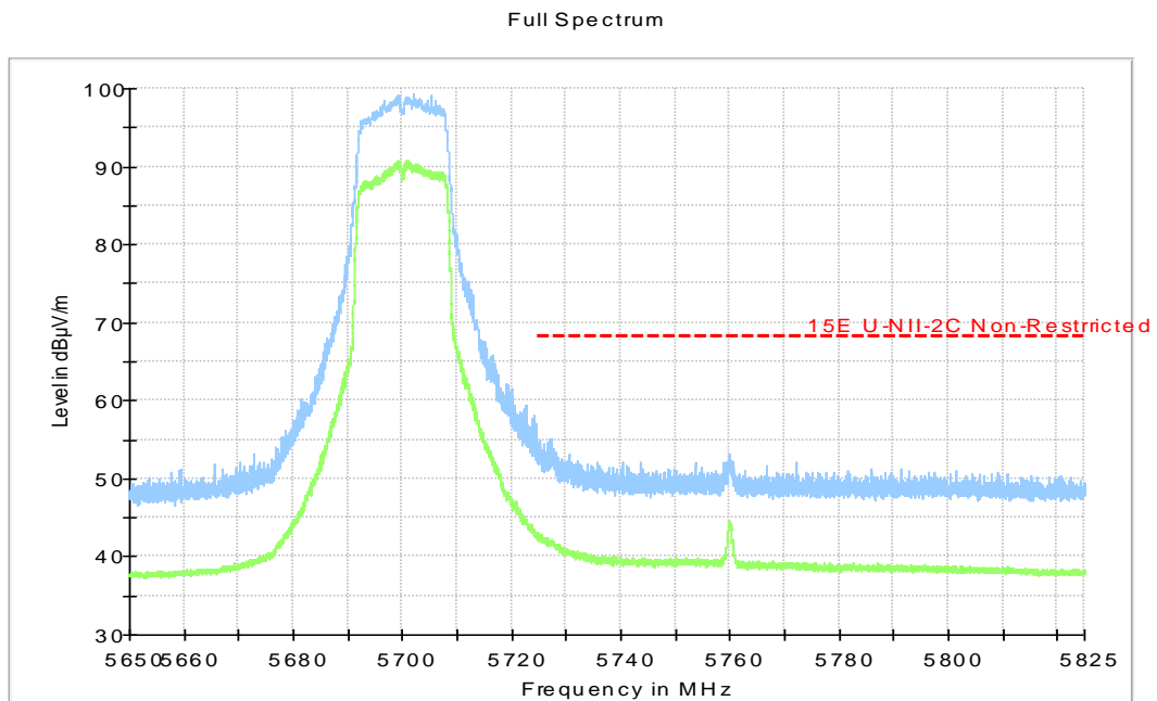
Fig.33 Band Edges (802.11a, 5700MHz)
