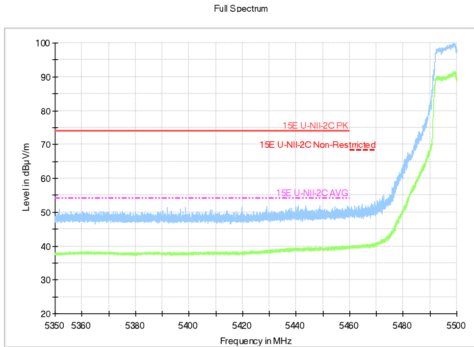
Fig.36 Band Edges (802.11a, 5500MHz)
