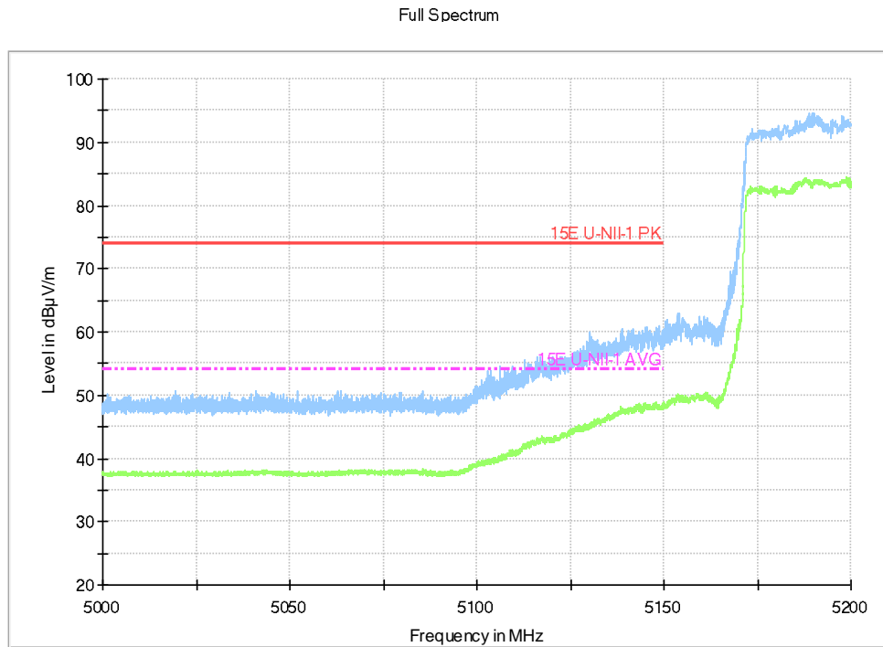
Fig.54 Band Edges (802.11ac-HT80, 5210MHz)
