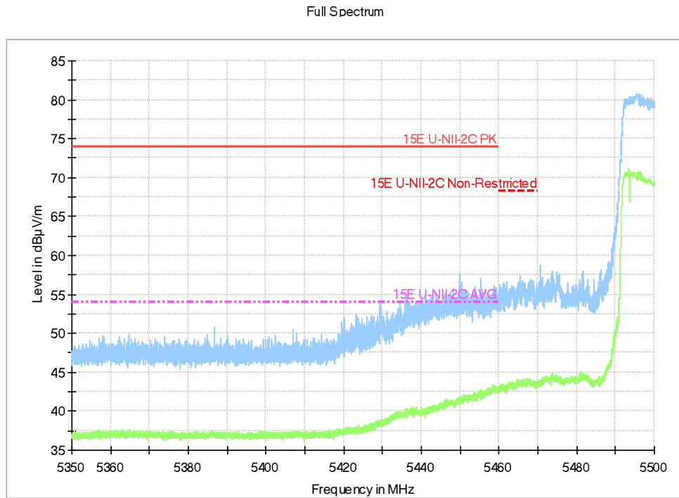
Fig.56 Band Edges (802.11ac-HT80, 5530MHz)
