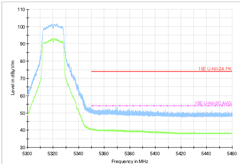
Fig.39 Band Edges (802.11n-HT20, 5320MHz)
