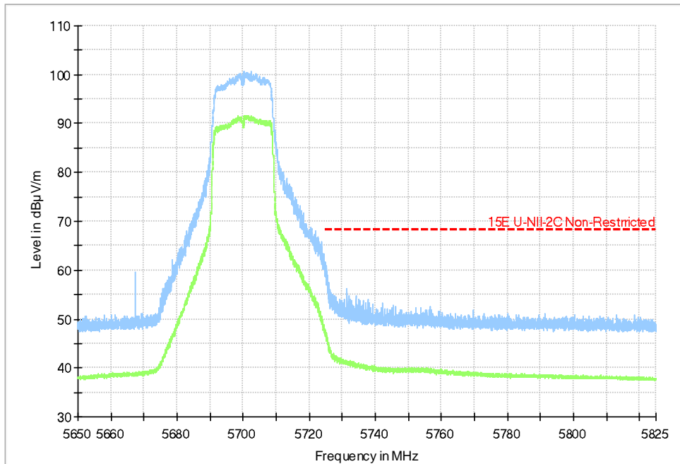
Fig.41 Band Edges (802.11n-HT20, 5700MHz)
