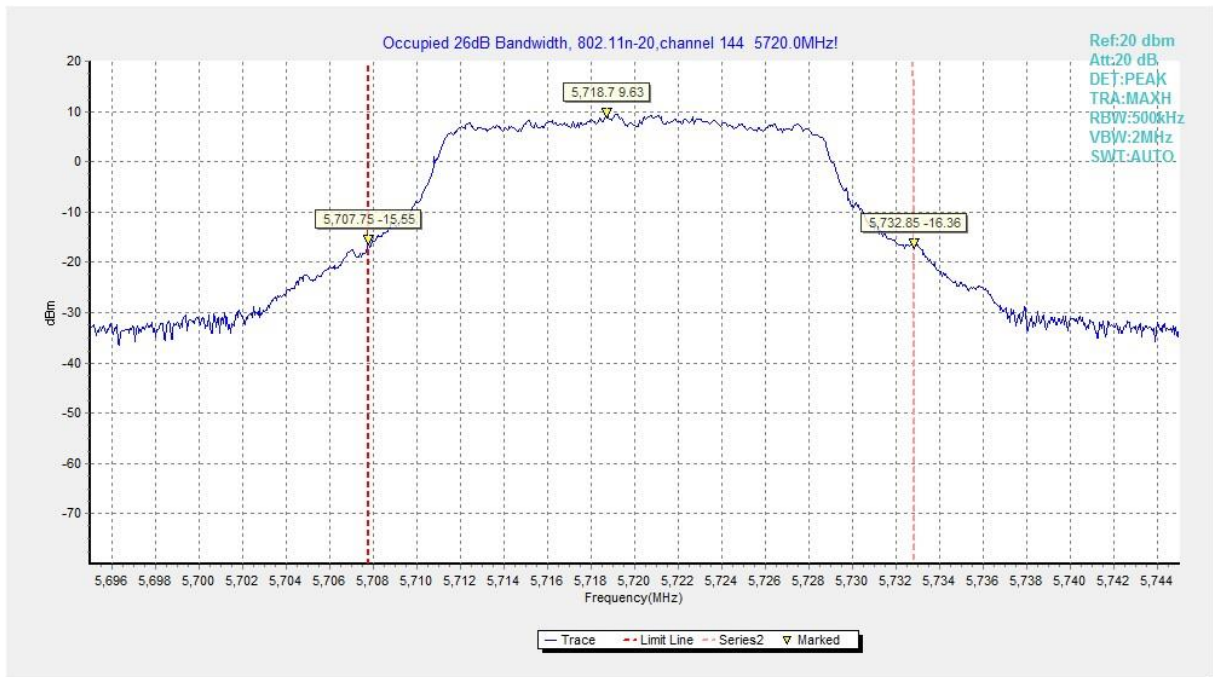
Fig.20 Occupied 26dB Bandwidth (802.11n-20, 5720MHz)
