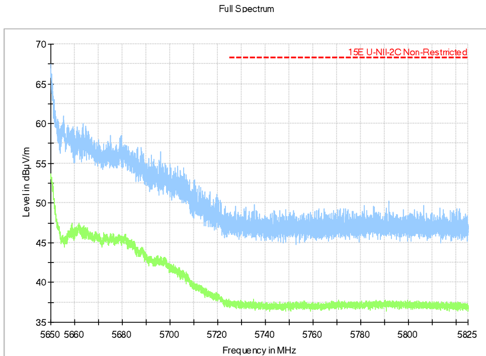
Fig.57 Band Edges (802.11ac-HT80, 5610MHz)
