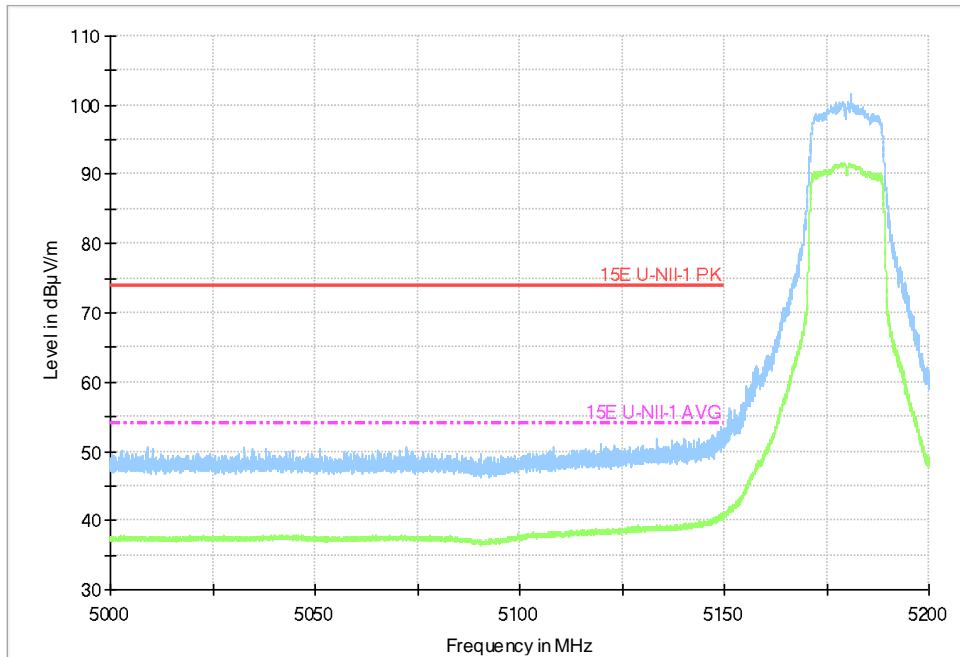
Fig.38 Band Edges (802.11n-HT20, 5180MHz)
