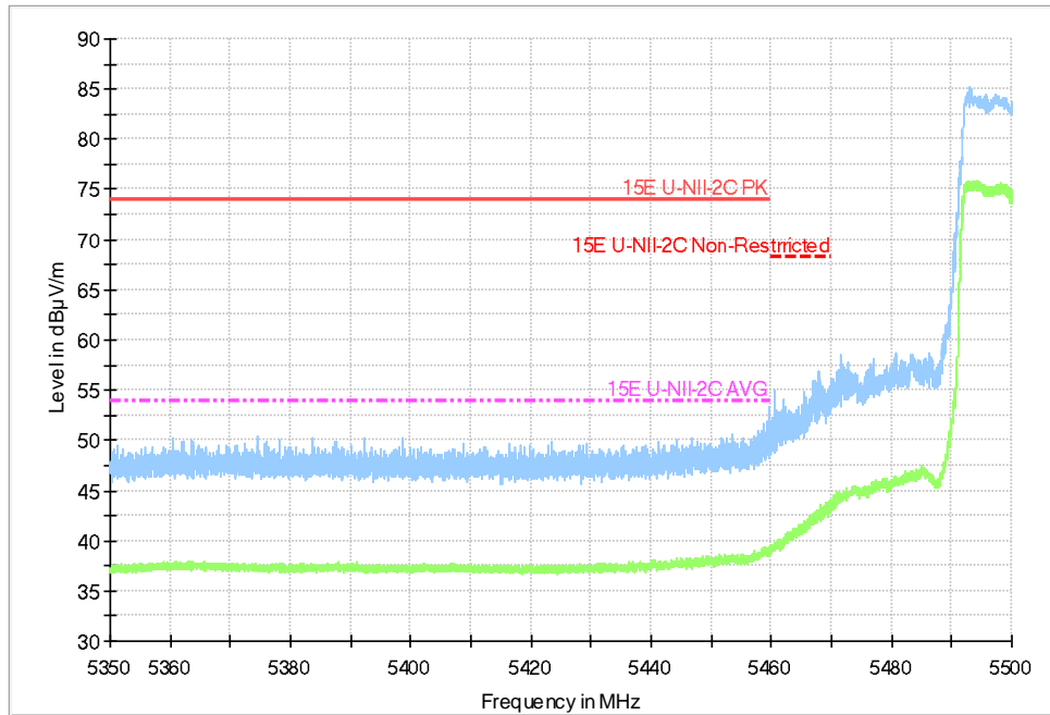
Fig.52 Band Edges (802.11ac-HT40, 5510MHz)
