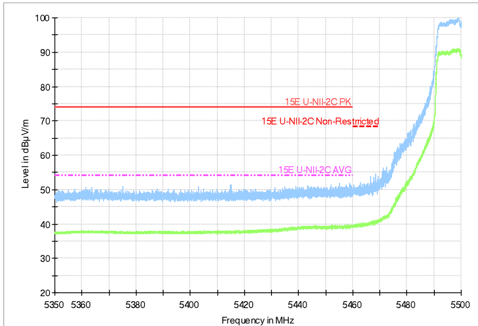
Fig.40 Band Edges (802.11n-HT20, 5500MHz)
