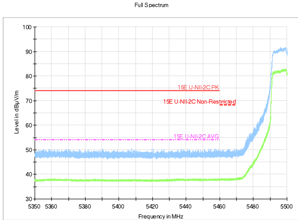
Fig.44 Band Edges (802.11ac-HT20, 5500MHz)
