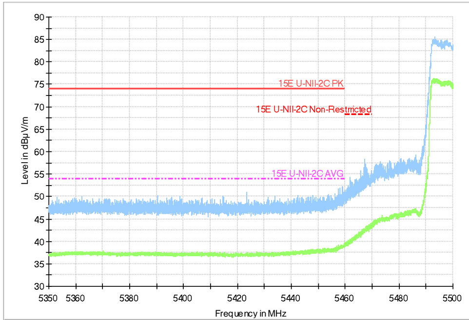
Fig.48 Band Edges (802.11n-HT40, 5510MHz)
