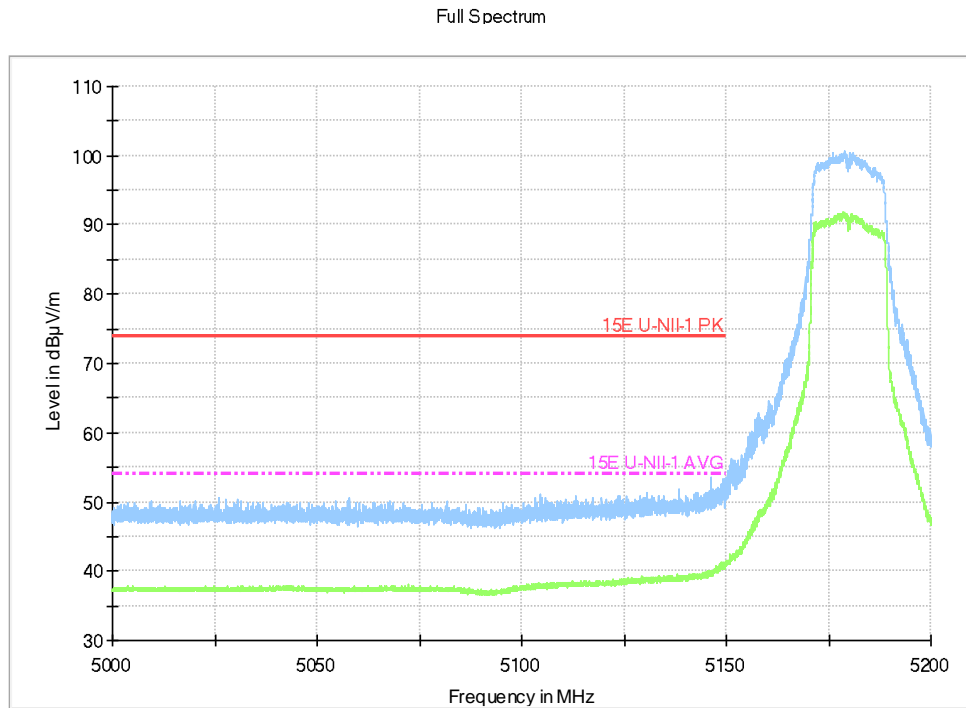
Fig.42 Band Edges (802.11ac-HT20, 5180MHz)
