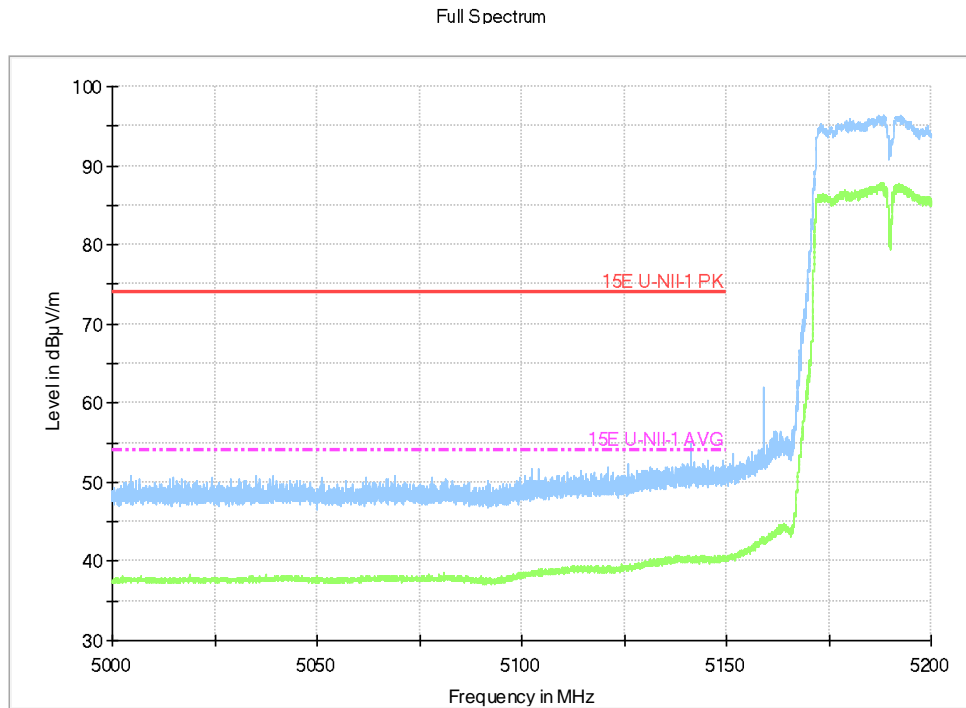
Fig.50 Band Edges (802.11ac-HT40, 5190MHz)
