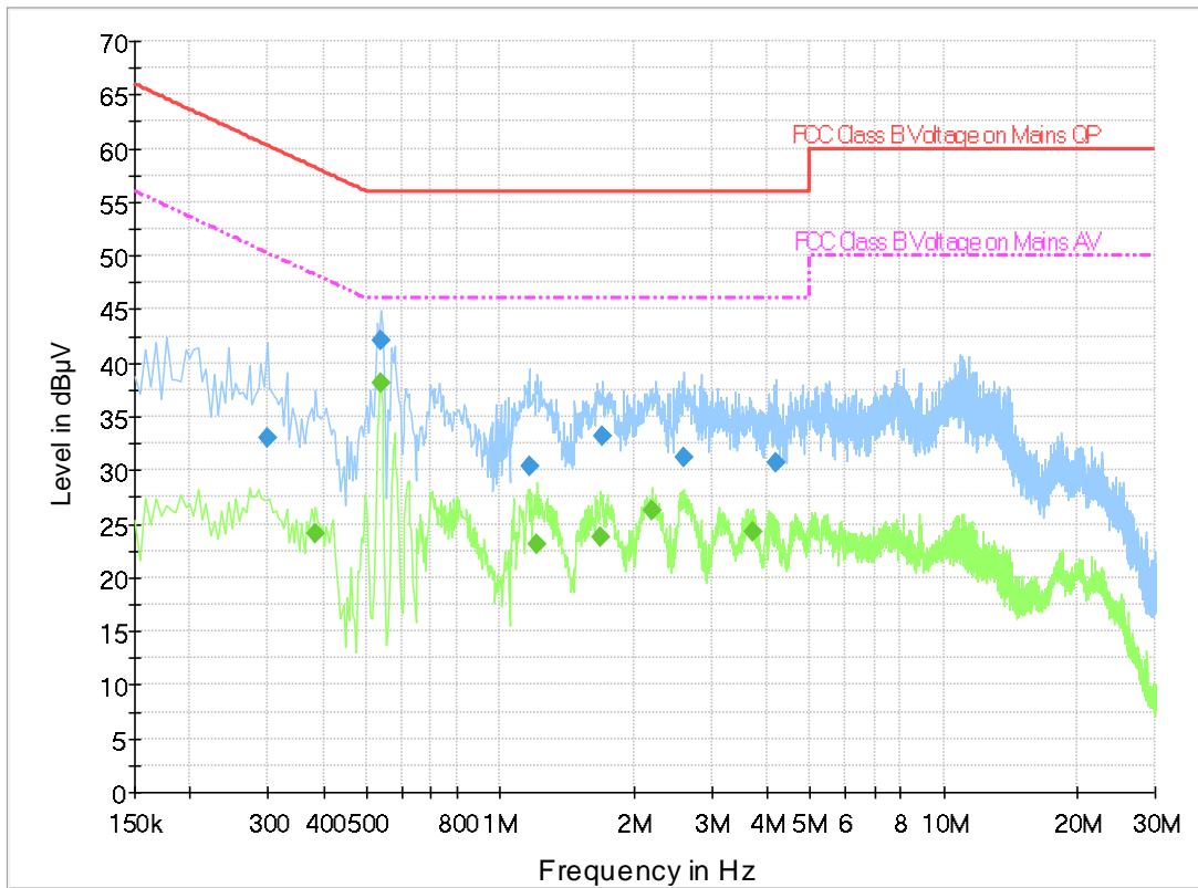
Fig.B.7.2 AC Powerline Conducted Emission-Idle
