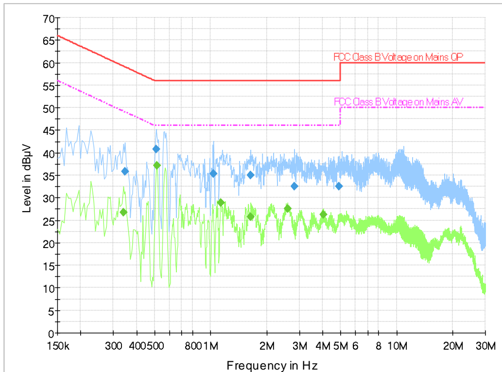
Fig.B.7.1 AC Powerline Conducted Emission-Traffic
