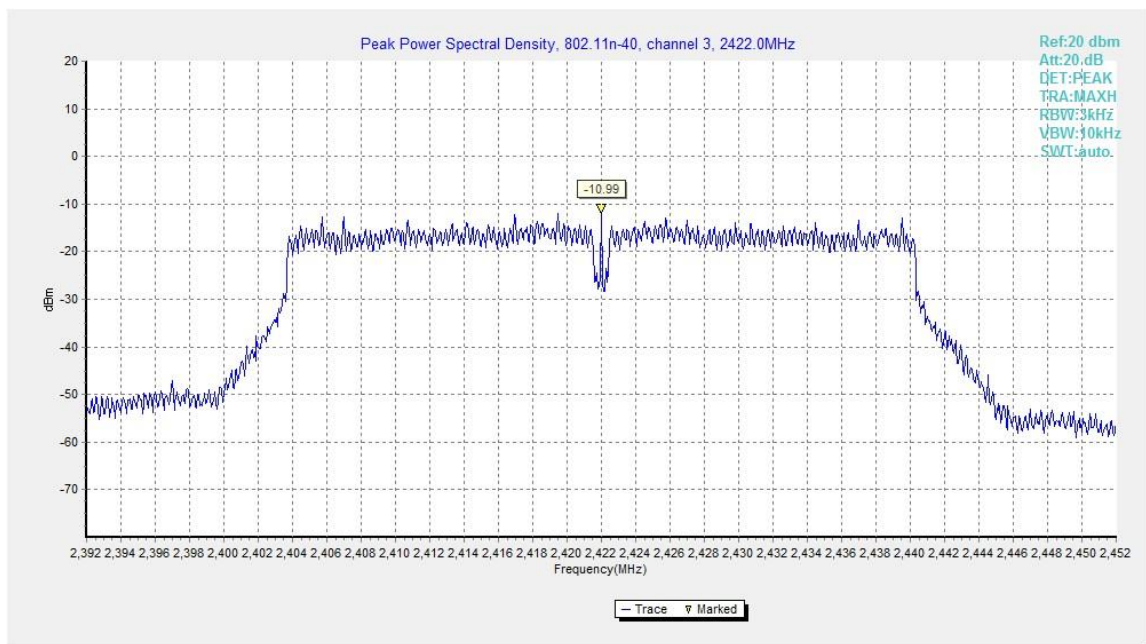
Fig.B.3.10 Power Spectral Density (802.11n-HT40, Ch 3)
