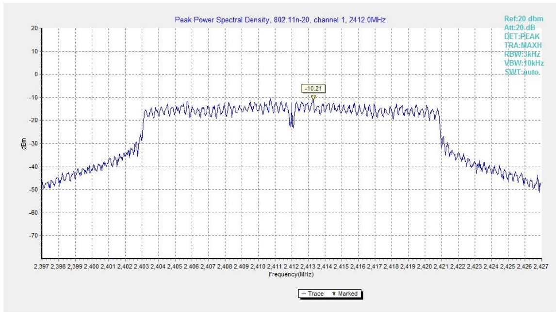
Fig.B.3.7 Power Spectral Density (802.11n-HT20, Ch 1)
