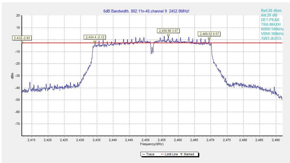
Fig.B.4.12 Occupied 6dB Bandwidth (802.11n-HT40, Ch 9)
