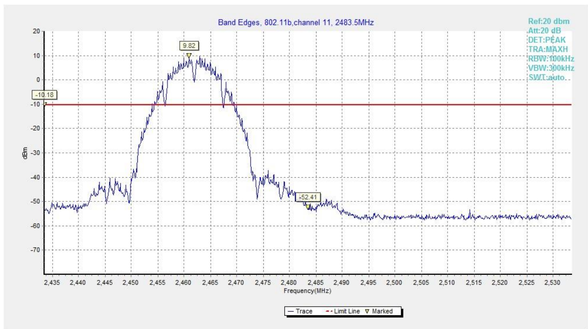
Fig.B.5.2 Band Edges (802.11b, Ch 11)
