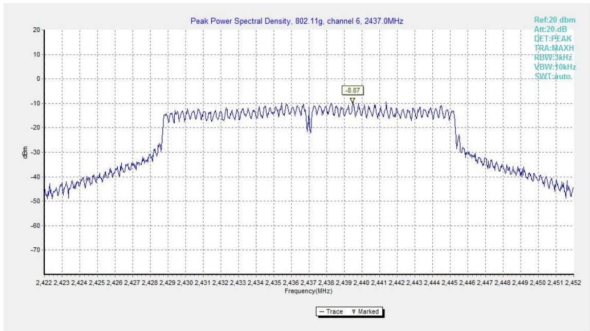
Fig.B.3.5 Power Spectral Density (802.11g, Ch 6)
