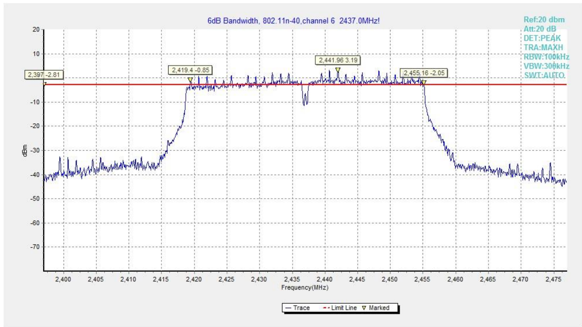
Fig.B.4.11 Occupied 6dB Bandwidth (802.11n-HT40, Ch 6)
