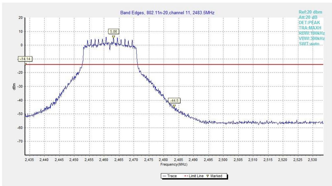
Fig.B.5.6 Band Edges (802.11n-HT20, Ch 11)
