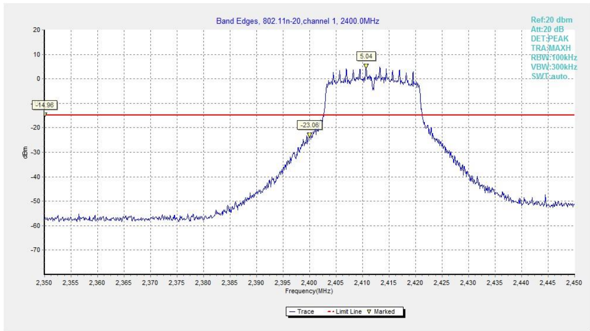
Fig.B.5.5 Band Edges (802.11n-HT20, Ch 1)
