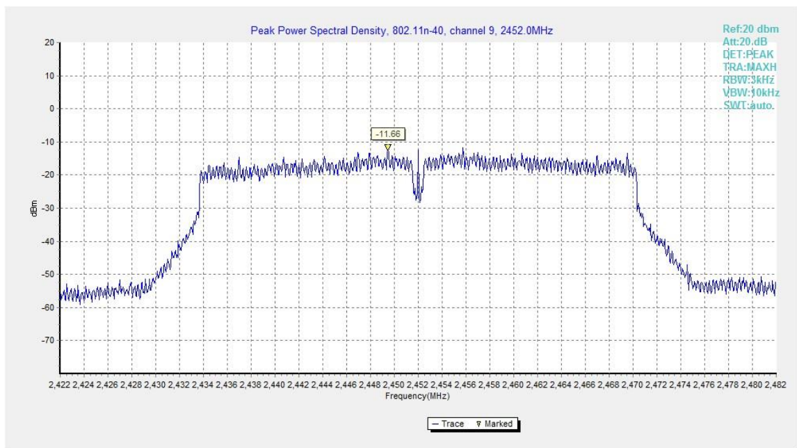
Fig.B.3.12 Power Spectral Density (802.11n-HT40, Ch 9)
