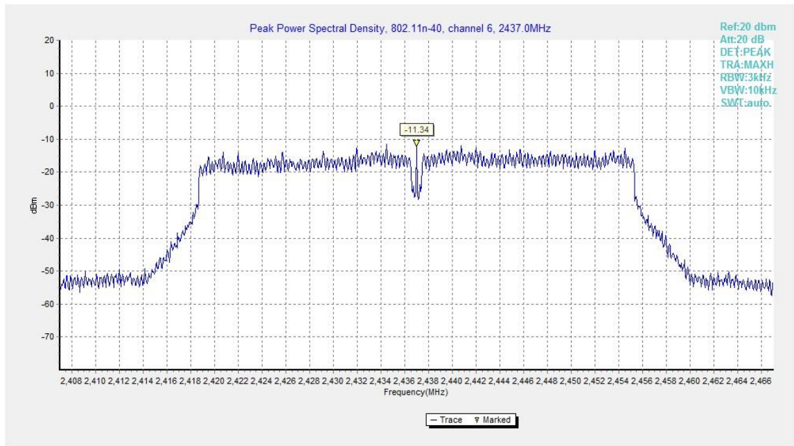
Fig.B.3.11 Power Spectral Density (802.11n-HT40, Ch 6)
