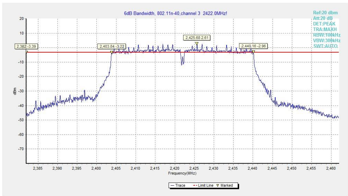
Fig.B.4.10 Occupied 6dB Bandwidth (802.11n-40MHz, Ch 3)
