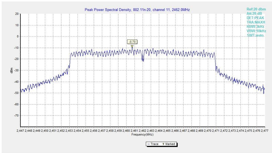
Fig.B.3.9 Power Spectral Density (802.11n-HT20, Ch 11)
