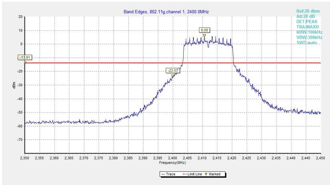
Fig.B.5.3 Band Edges (802.11g, Ch 1)
