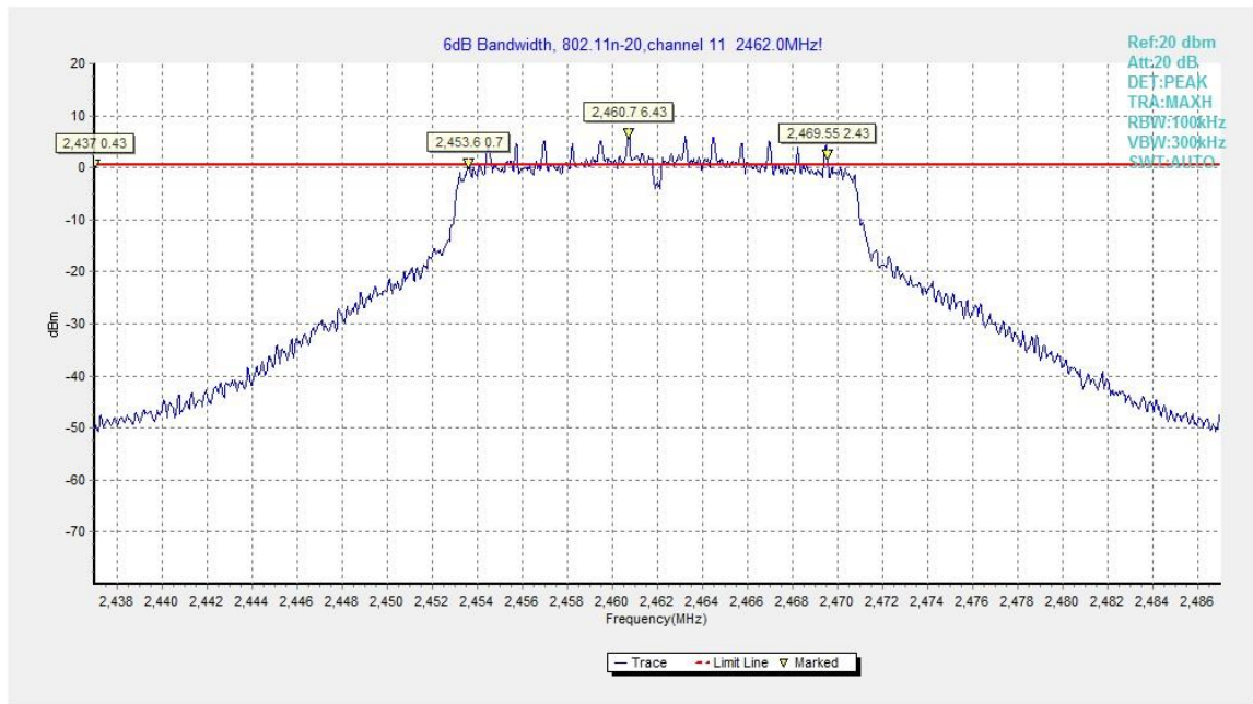
Fig.B.4.9 Occupied 6dB Bandwidth (802.11n-HT20, Ch 11)
