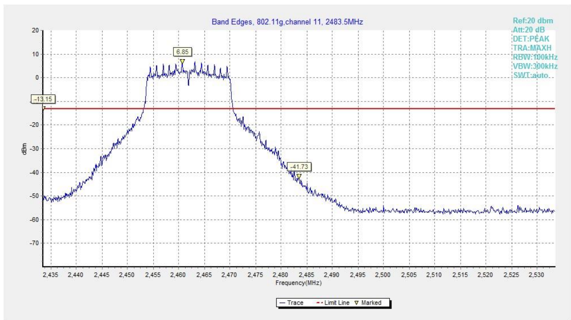
Fig.B.5.4 Band Edges (802.11g, Ch 11)
