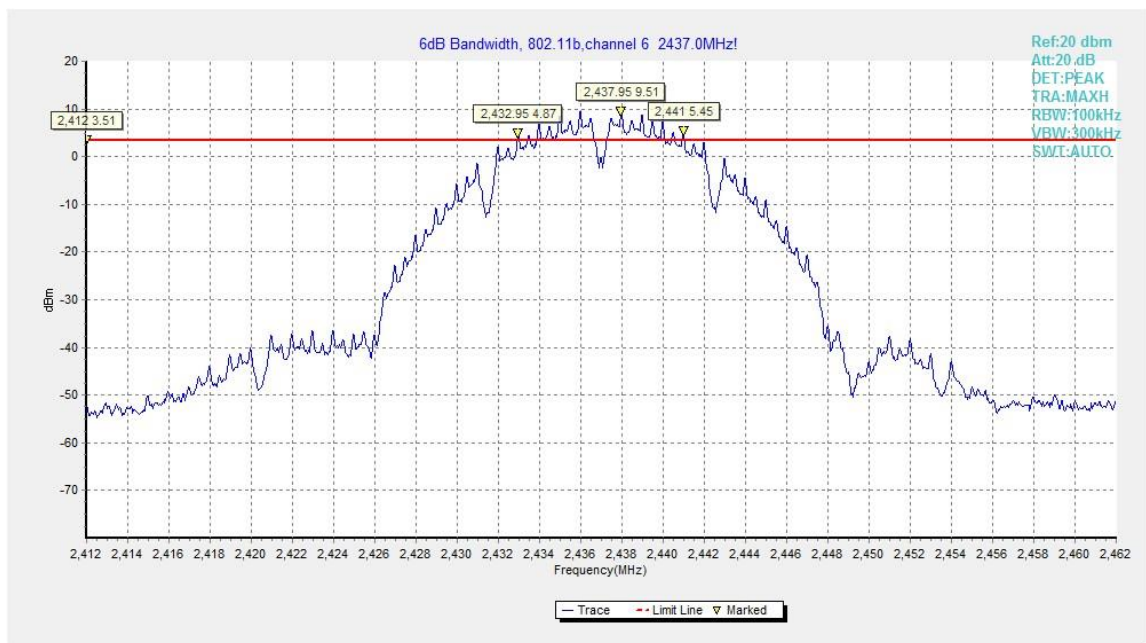
Fig.B.4.2 Occupied 6dB Bandwidth (802.11b, Ch 6)
