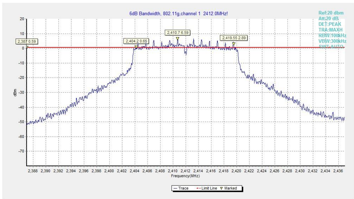
Fig.B.4.4 Occupied 6dB Bandwidth (802.11g, Ch 1)
