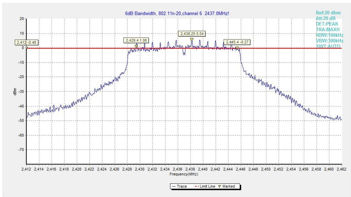
Fig.B.4.8 Occupied 6dB Bandwidth (802.11n-HT20, Ch 6)
