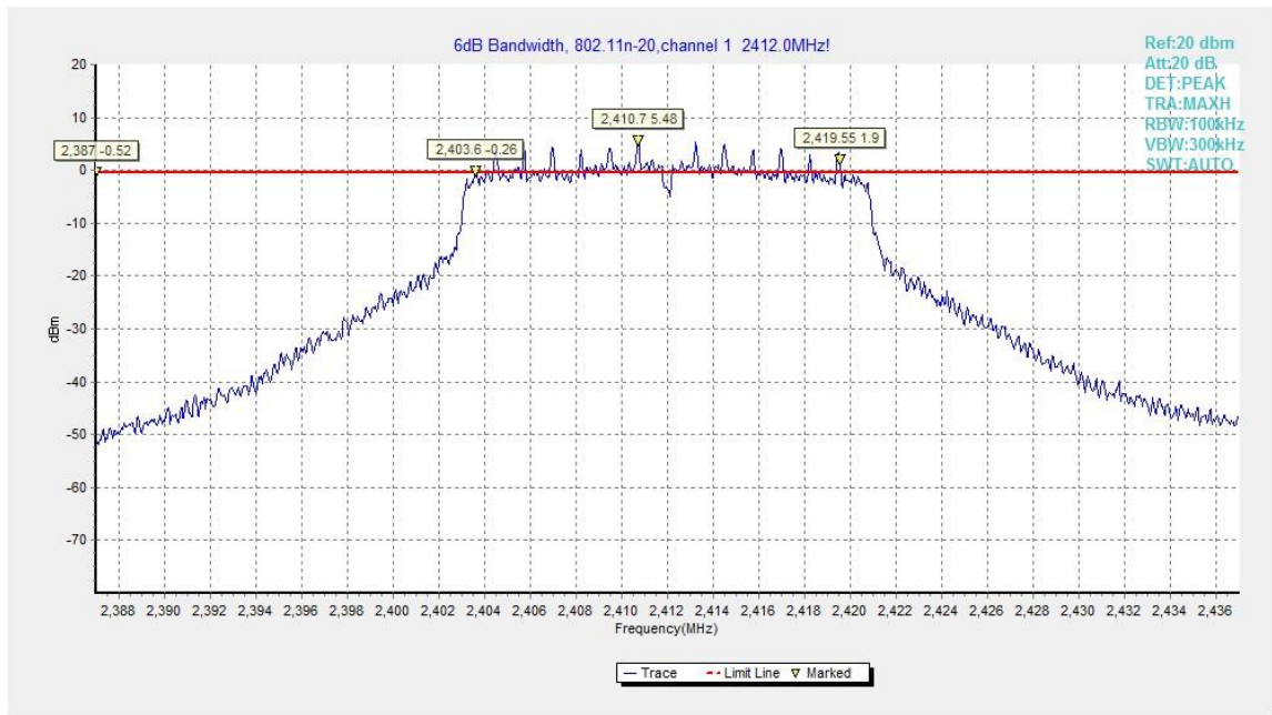
Fig.B.4.7 Occupied 6dB Bandwidth (802.11n-20MHz, Ch 1)
