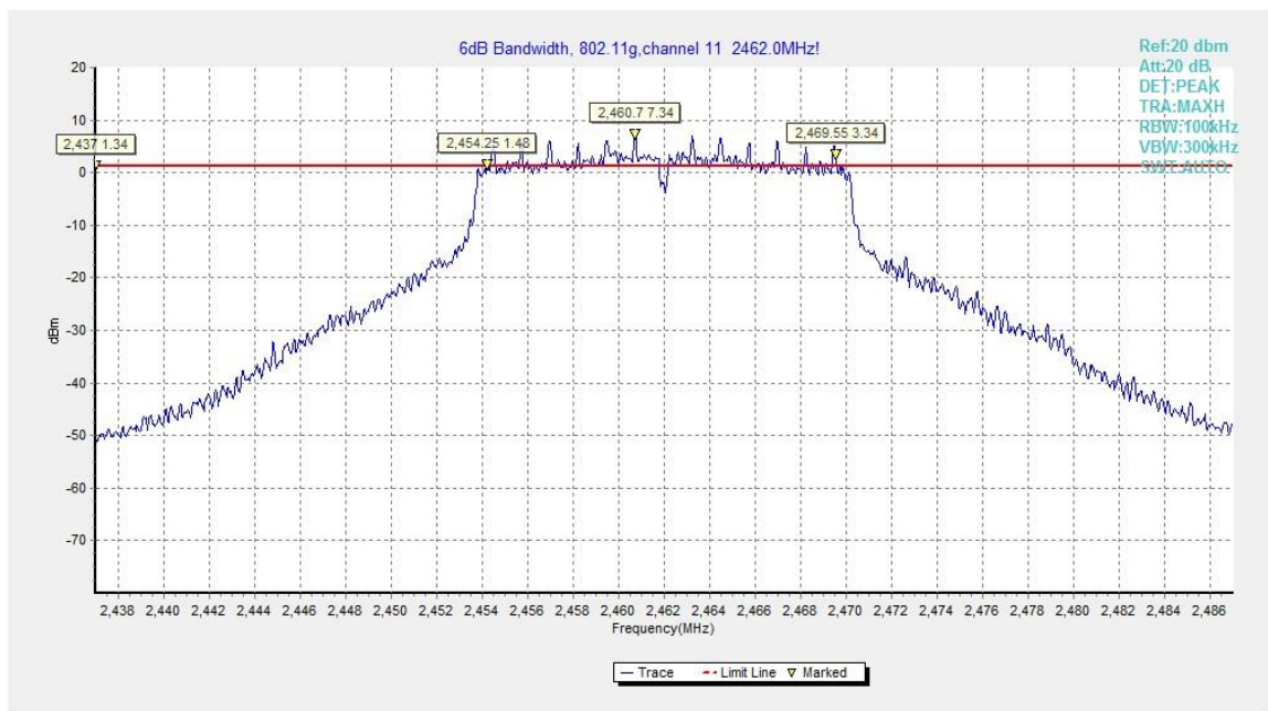
Fig.B.4.6 Occupied 6dB Bandwidth (802.11g, Ch 11)
