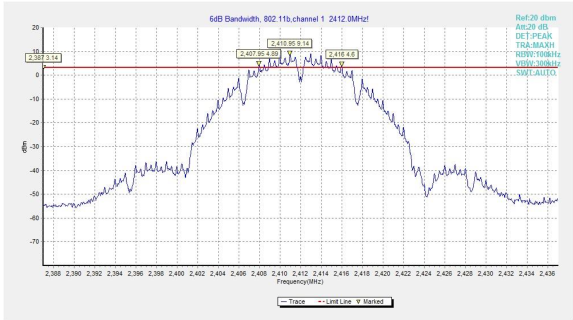
Fig.B.4.1 Occupied 6dB Bandwidth(802.11b,Ch 1)
