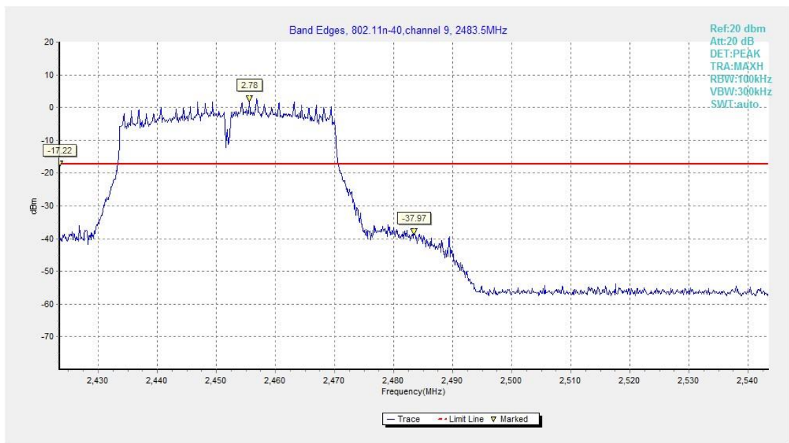
Fig.B.5.8 Band Edges (802.11n-HT40, Ch 9)
