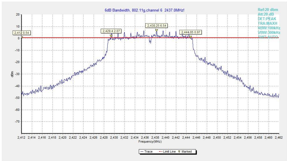
Fig.B.4.5 Occupied 6dB Bandwidth (802.11g, Ch 6)
