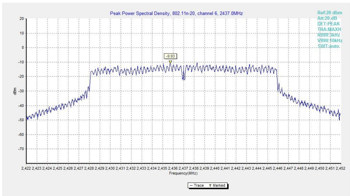
Fig.B.3.8 Power Spectral Density (802.11n-HT20, Ch 6)
