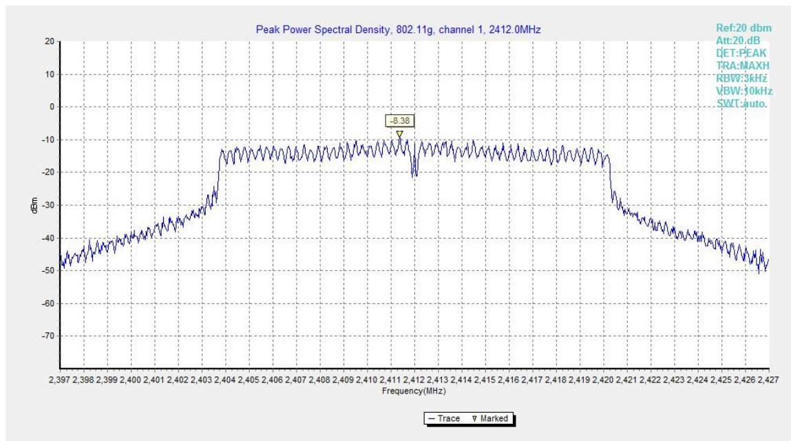
Fig.B.3.4 Power Spectral Density (802.11g, Ch 1)
