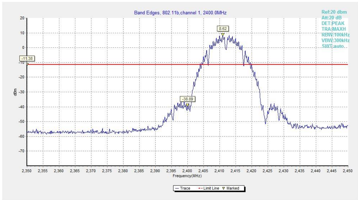
Fig.B.5.1 Band Edges (802.11b, Ch 1)
