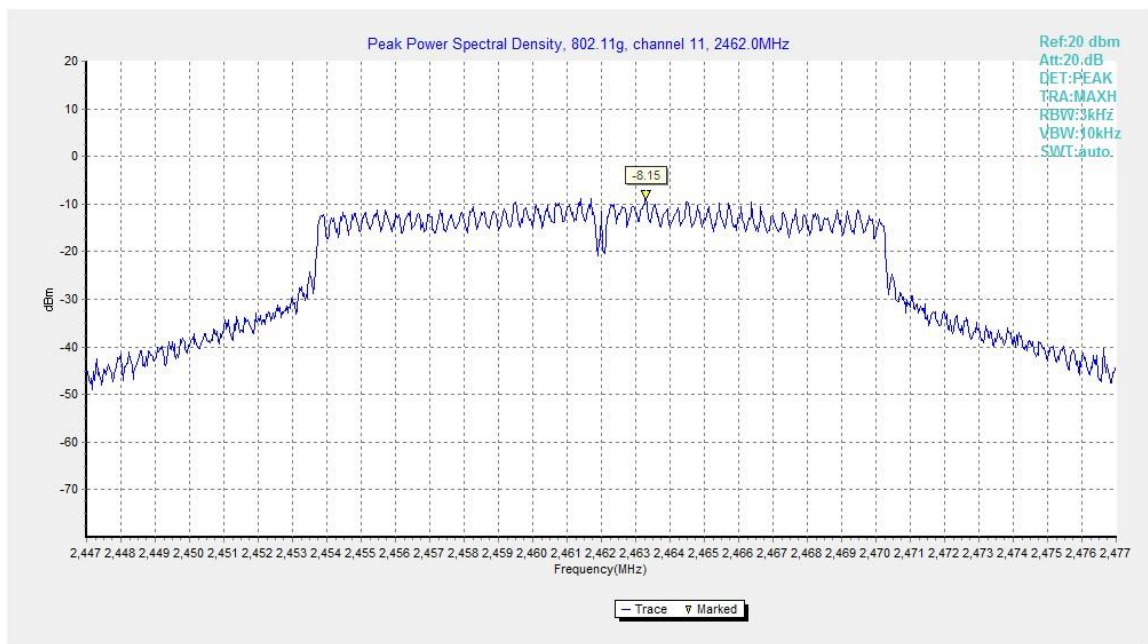
Fig.B.3.6 Power Spectral Density (802.11g, Ch 11)
