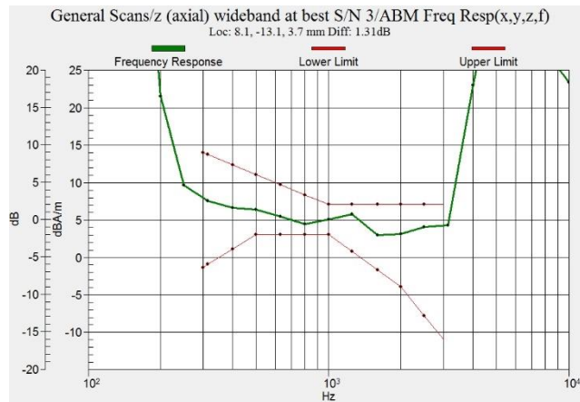
Figure C.8 Frequency Response of LTE B41 - OTT VoIP
