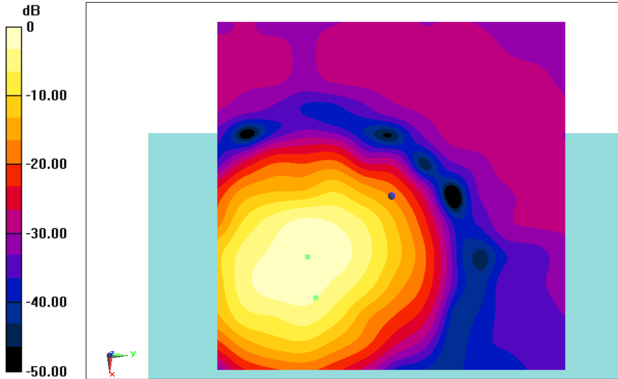
Fig B.6 T-Coil LTE B41
