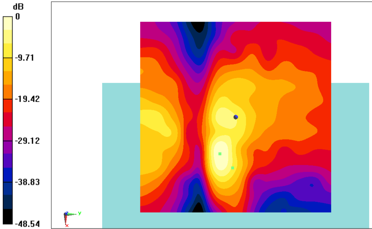
Fig B.3 T-Coil LTE B12
