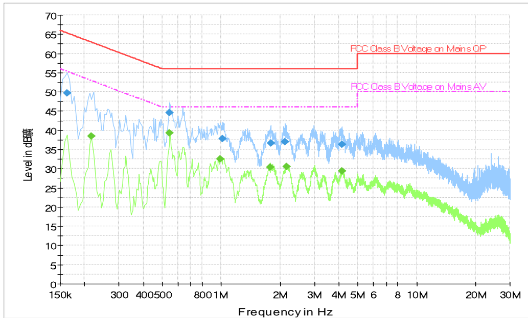
Fig.A.7.4 AC Powerline Conducted Emission- 802.11b, charger UC13US(PUAN)
