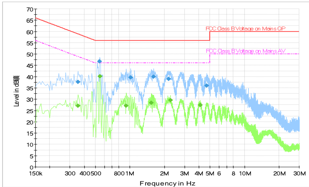
Fig.A.7.1 AC Powerline Conducted Emission- 802.11b, charger QC13US(BYD)
