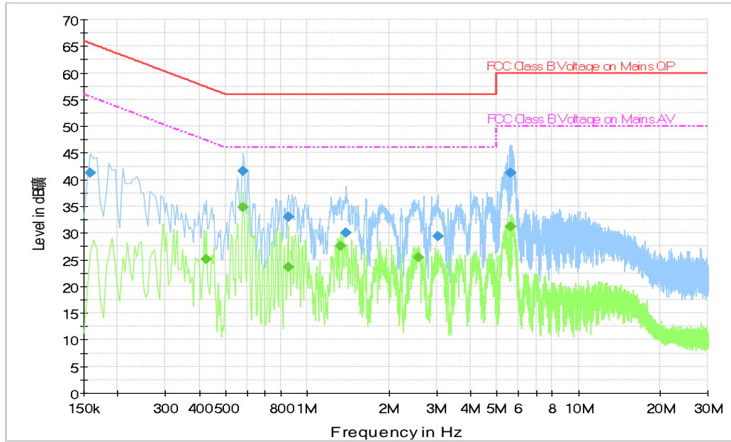
Fig.A.7.3 AC Powerline Conducted Emission- 802.11b, charger QC13US(PUAN)
