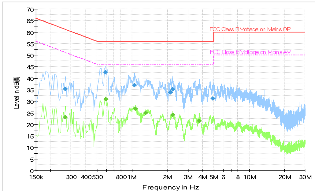
Fig.A.7.5 AC Powerline Conducted Emission- 802.11b, charger UC13US(Chen Yang)
