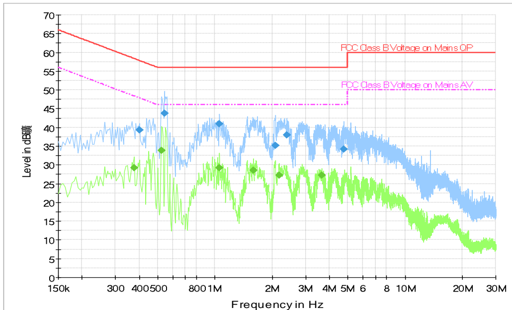
Fig.A.7.2 AC Powerline Conducted Emission-Idle, charger QC13US(BYD)
