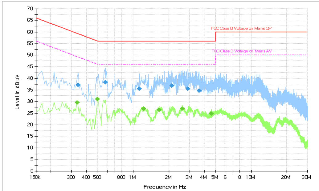
Fig.B.11.1 AC Powerline Conducted Emission- bluetooth, charger QC13US(BYD)
