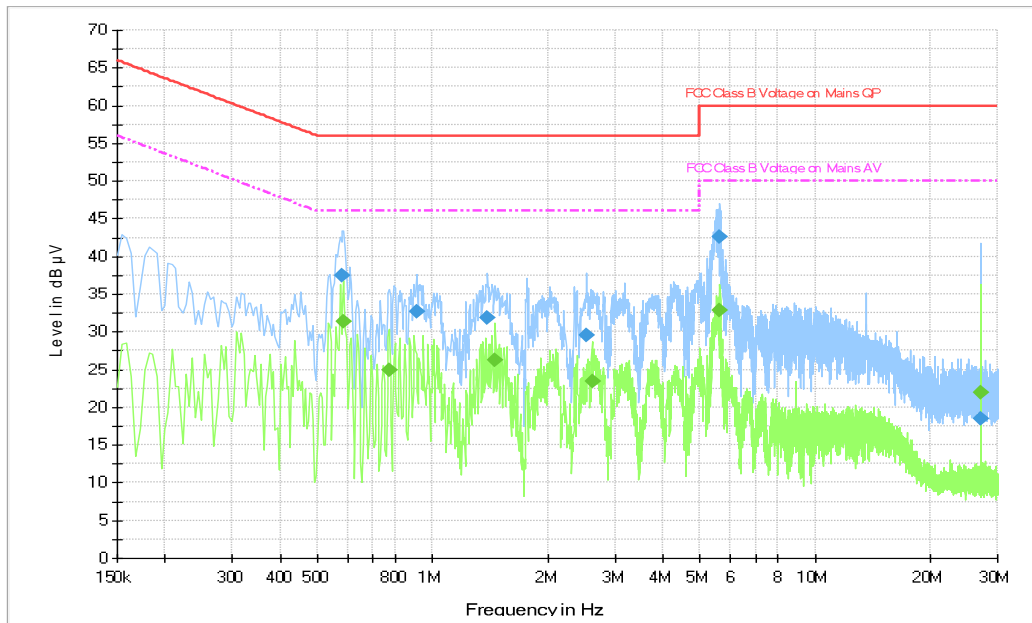
Fig.B.11.3 AC Powerline Conducted Emission- bluetooth, charger QC13US(PUAN)
