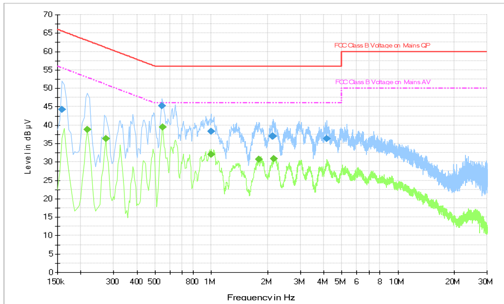
Fig.B.11.4 AC Powerline Conducted Emission- bluetooth, charger UC13US(PUAN)
