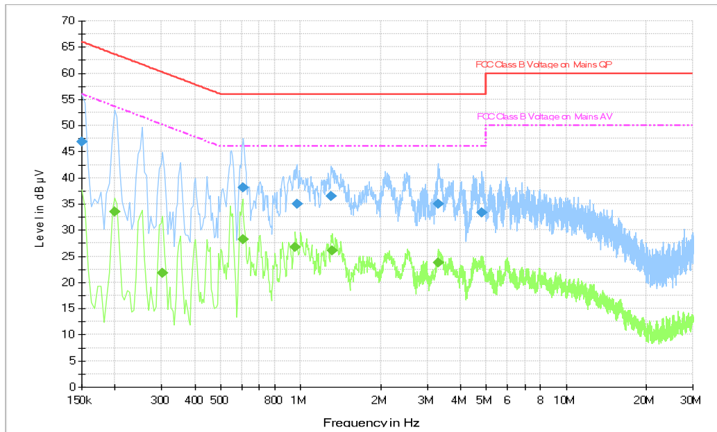
Fig.B.11.5 AC Powerline Conducted Emission- bluetooth, charger UC13US(Chen Yang)
