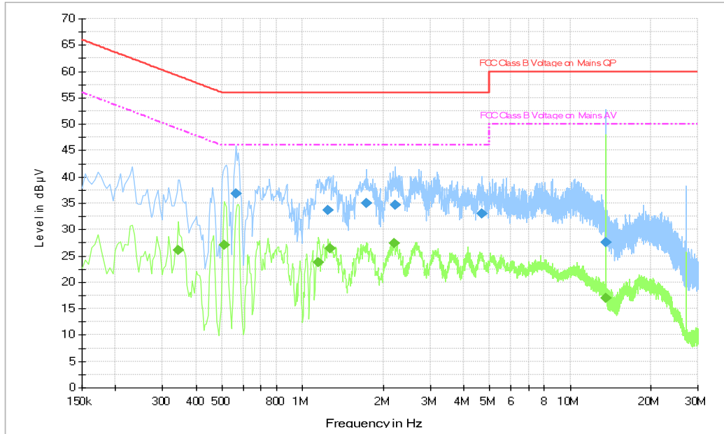
Fig.B.11.2 AC Powerline Conducted Emission-Idle, charger QC13US(BYD)
