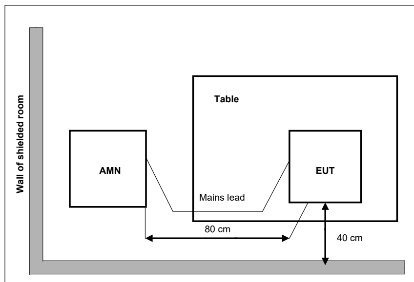
Figure B-10: Measurement Setup
