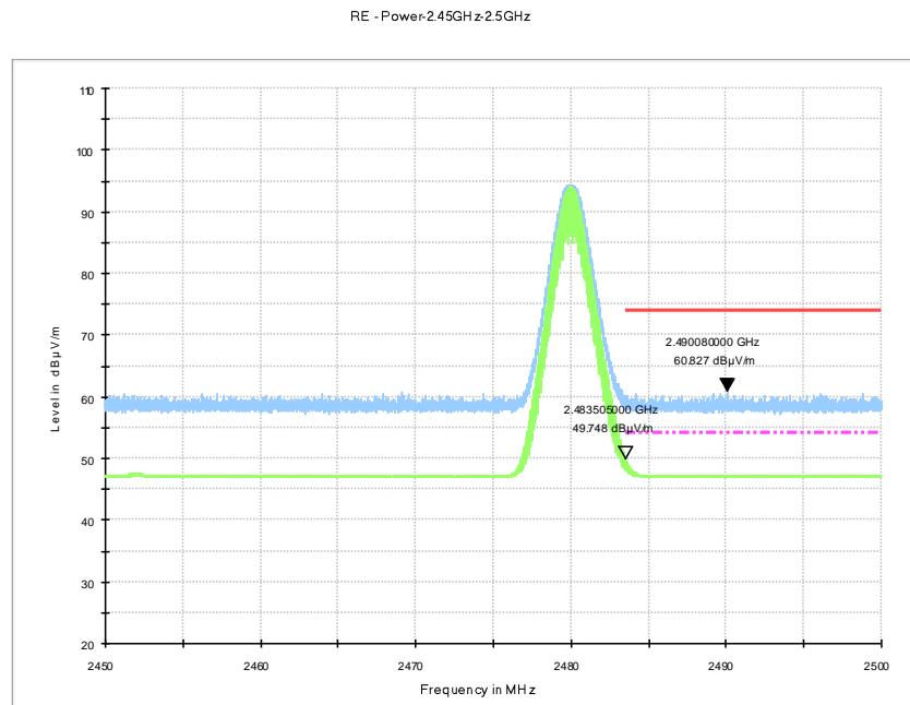
Fig.14. Frequency Band Edges: GFSK, Channel 78, ch11, 2.45 GHz - 2.50GHz
