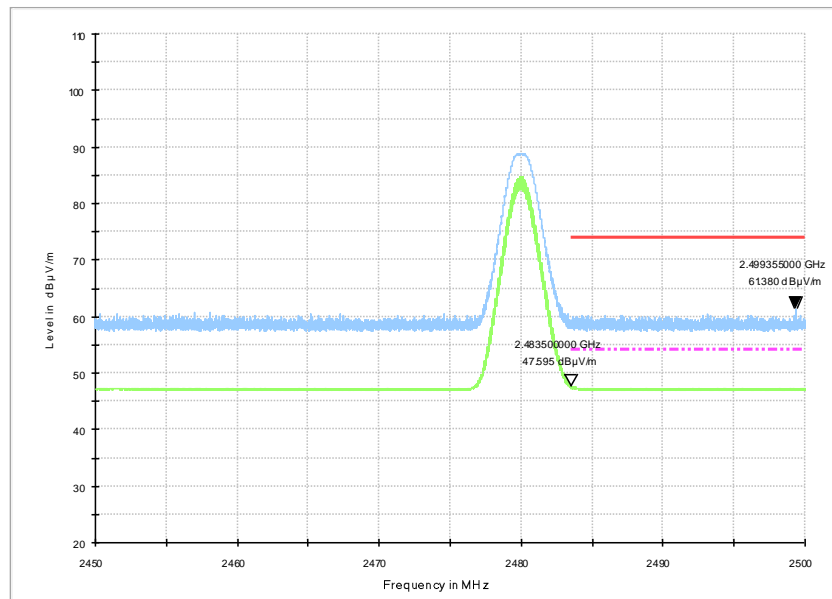
Fig.4. Frequency Band Edges: GFSK, 2480 MHz, 2.45 GHz - 2.50GHz
