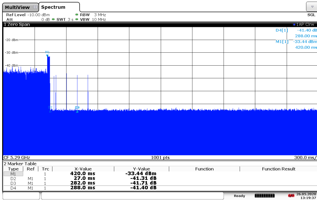
Fig.A.5 channel closing transmission time
