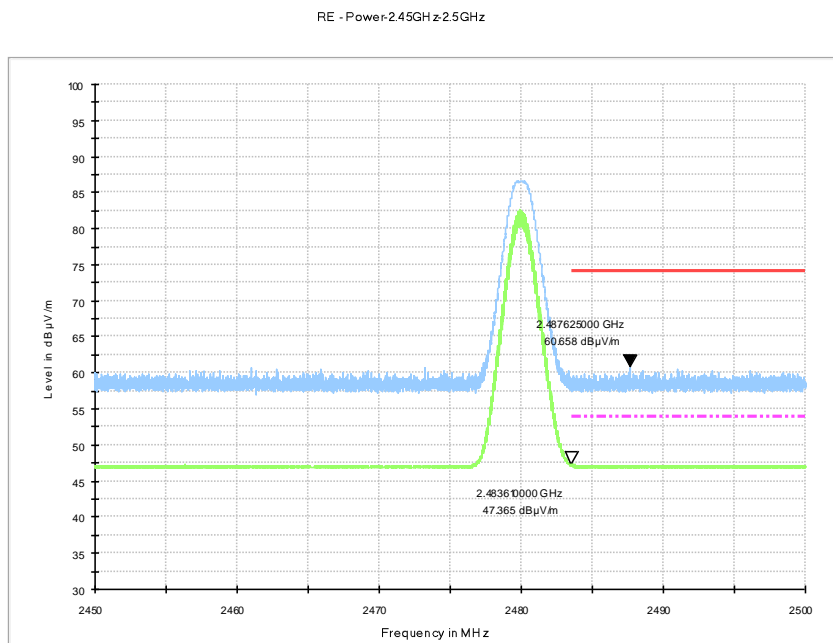
Fig.4. Frequency Band Edges: GFSK, 2480 MHz, 2.45 GHz - 2.50GHz
