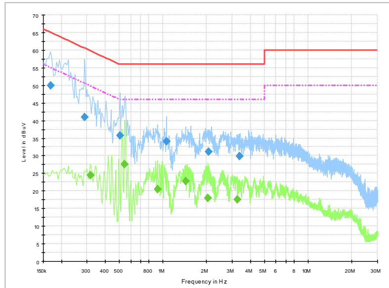
Fig.A.9.1 AC Powerline Conducted Emission-traffic
