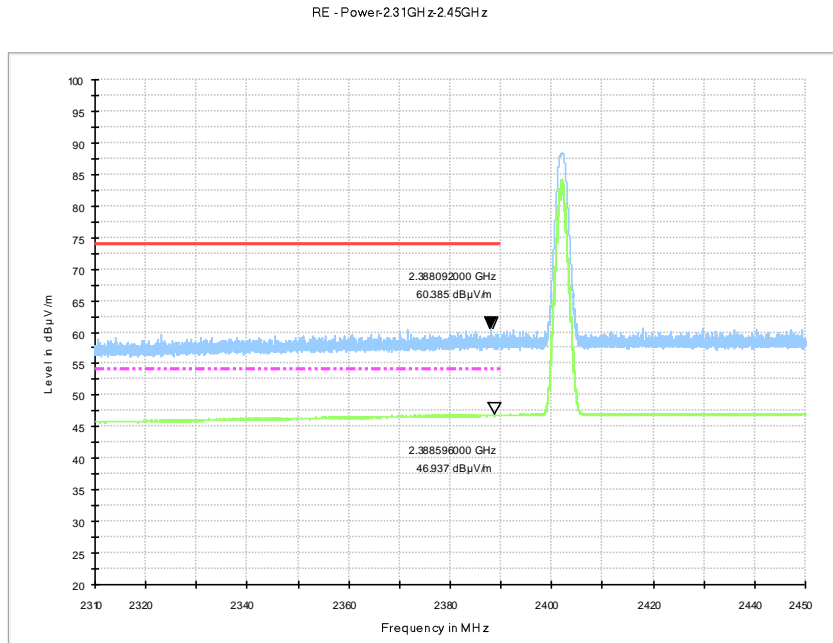
Fig.3. Frequency Band Edges: GFSK, 2402 MHz, 2.31 GHz – 2.45GHz
