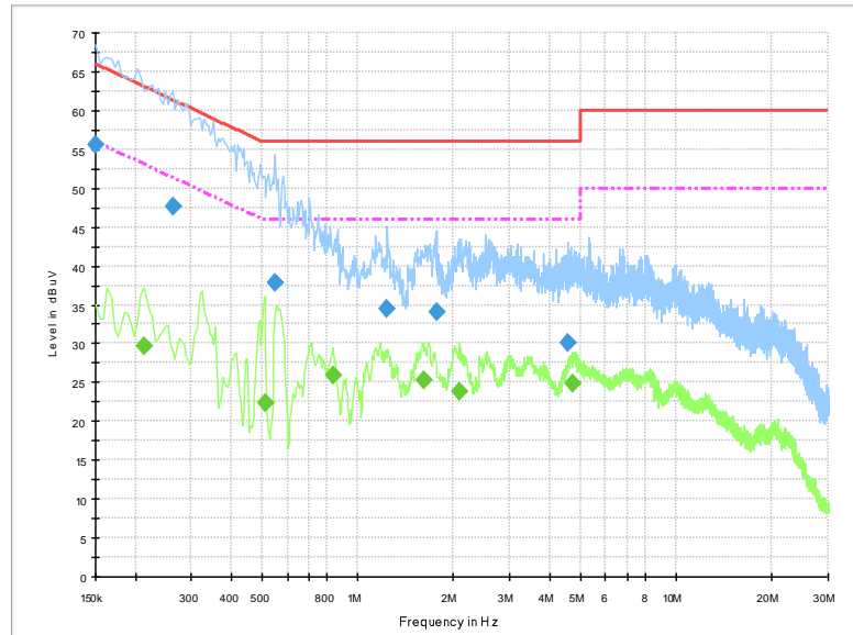
Fig.A.11.1 AC Powerline Conducted Emission-traffic
