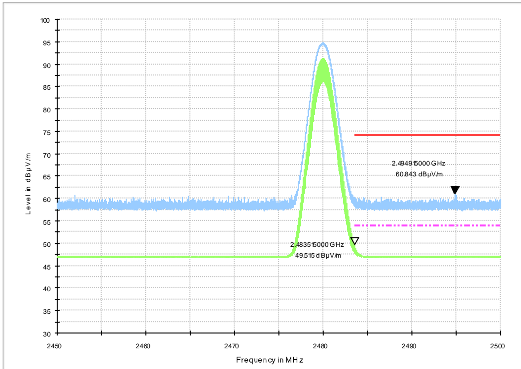
Fig.18. Frequency Band Edges: 8DPSK, Channel 78, 2.45 GHz - 2.50GHz
