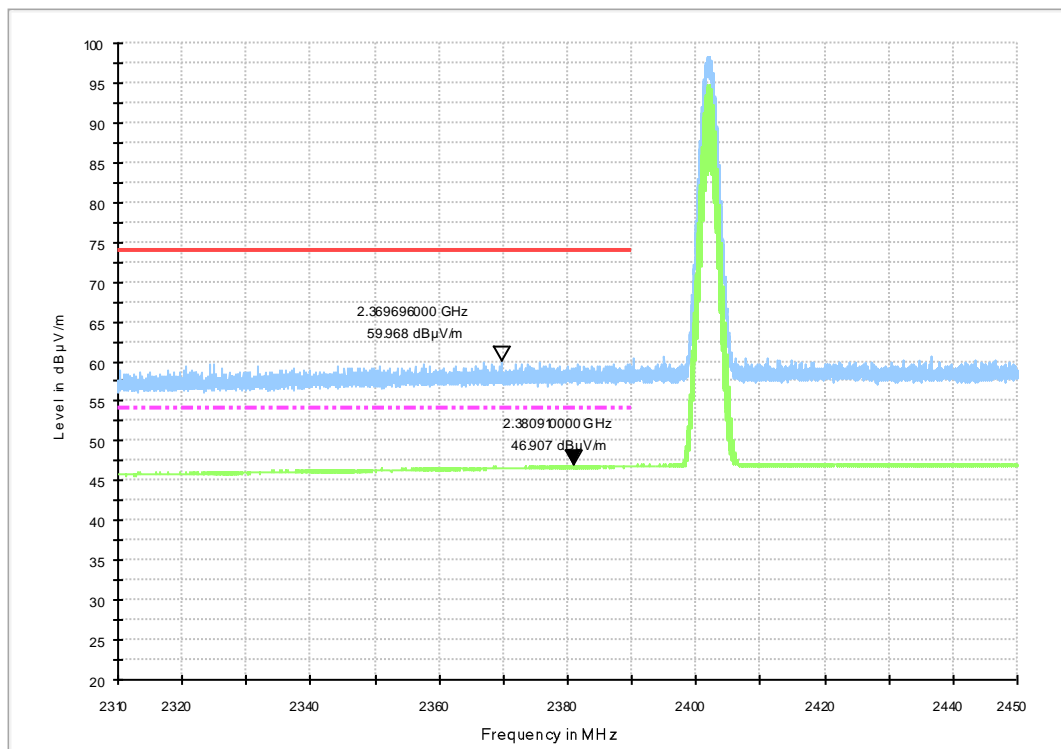
Fig.17. Frequency Band Edges: 8DPSK, Channel 0, 2.31 GHz - 2.45GHz
