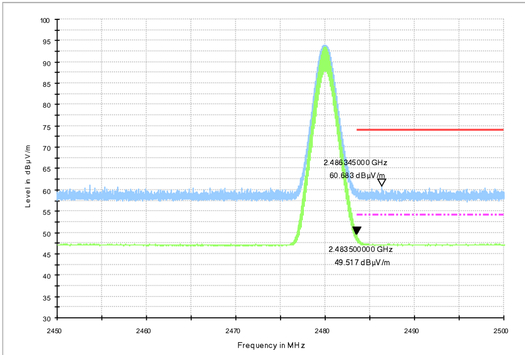
Fig.14. Frequency Band Edges: GFSK, Channel 78, ch11, 2.45 GHz - 2.50GHz
