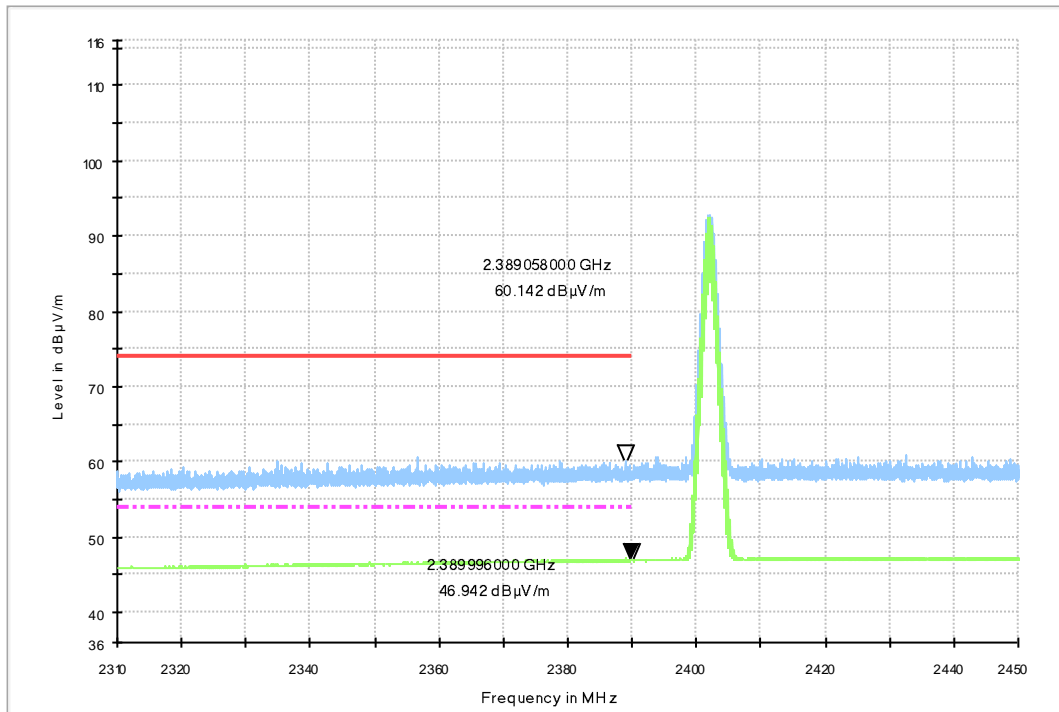
Fig.13. Frequency Band Edges: GFSK, Channel 0, 2.31 GHz – 2.45GHz
