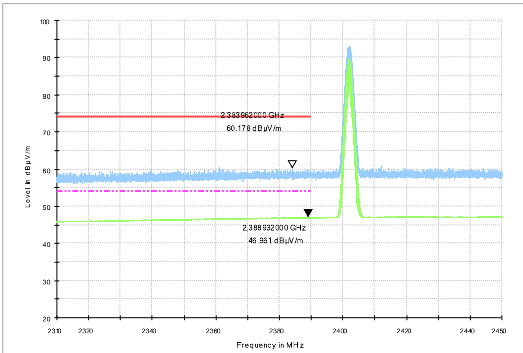
Fig.15. Frequency Band Edges: \pi/4 DQPSK, Channel 0, 2.31 GHz - 2.45GHz
