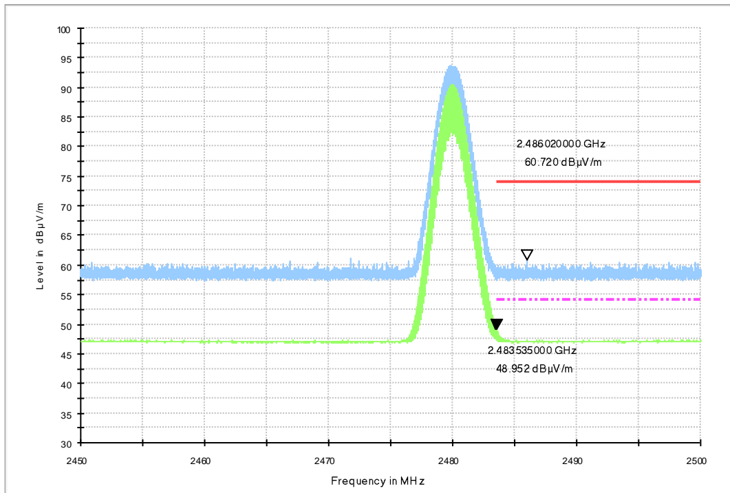
Fig.16. Frequency Band Edges: \pi/4 DQPSK, Channel 78, 2.45 GHz - 2.50GHz
