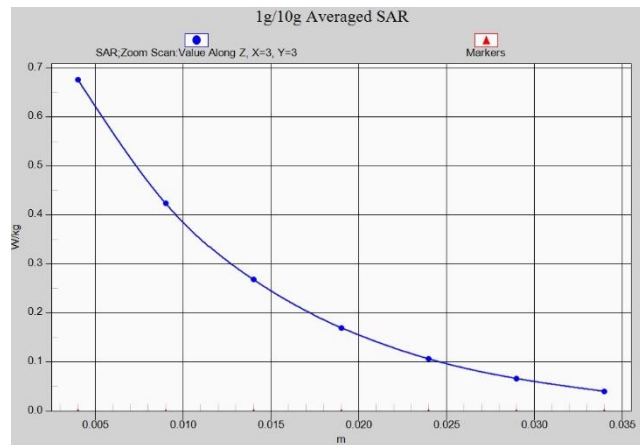
Fig. 1-40 Z-Scan at power reference point (LTE Band66)
