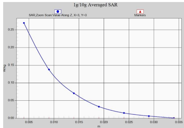
Fig. 1-37 Z-Scan at power reference point (LTE Band41)
