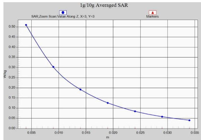
Fig. 1-58 Z-Scan at power reference point (n71)
