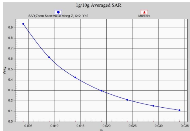
Fig. 1-42 Z-Scan at power reference point (LTE Band71)
