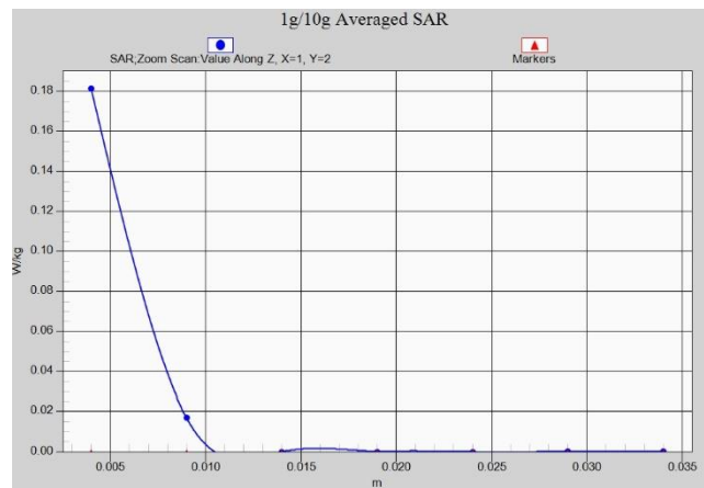
Fig. 1-45 Z-Scan at power reference point (wifi5G)
