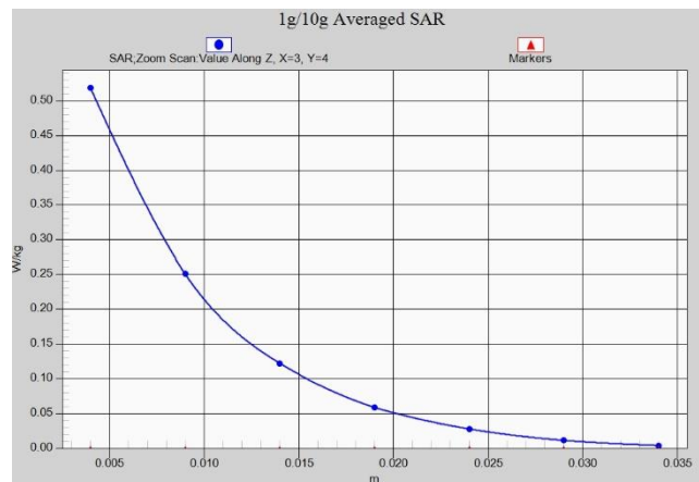
Fig. 1-36 Z-Scan at power reference point (LTE Band41)
