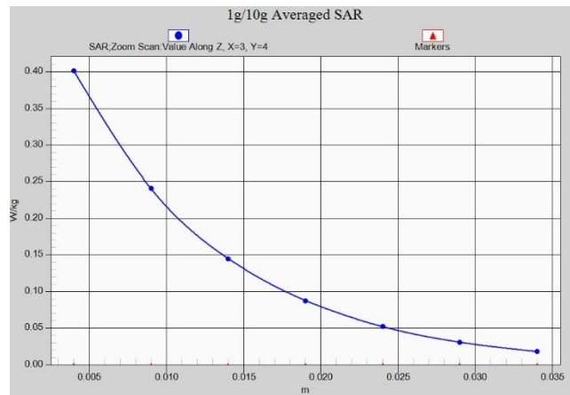
Fig. 1-49 Z-Scan at power reference point (n2)
