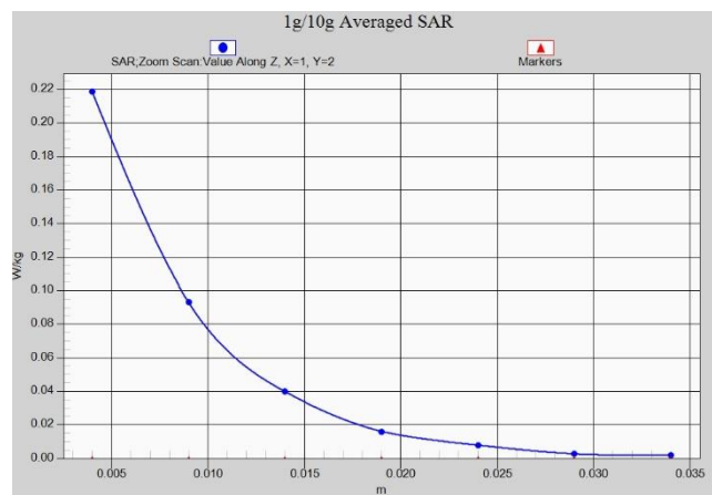
Fig. 1-35 Z-Scan at power reference point (LTE Band41)
