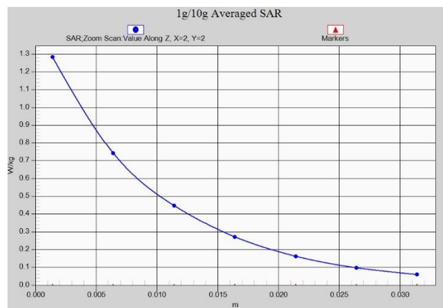
Fig. 1-29 Z-Scan at power reference point (LTE Band25)
