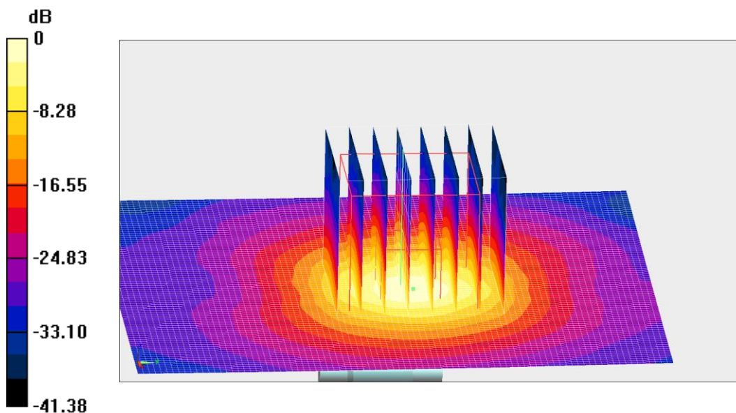
Fig.B.16 validation 5750 MHz 100mW
