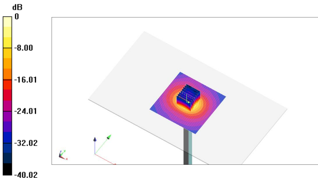
Fig.B.14 validation 5250 MHz 100mW
