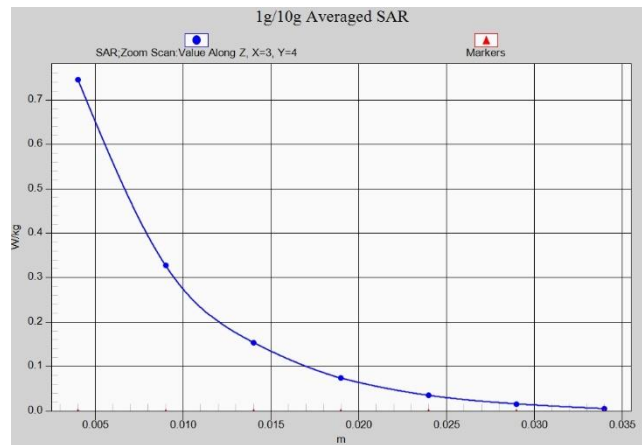
Fig. 1-43 Z-Scan at power reference point (wifi2450)
