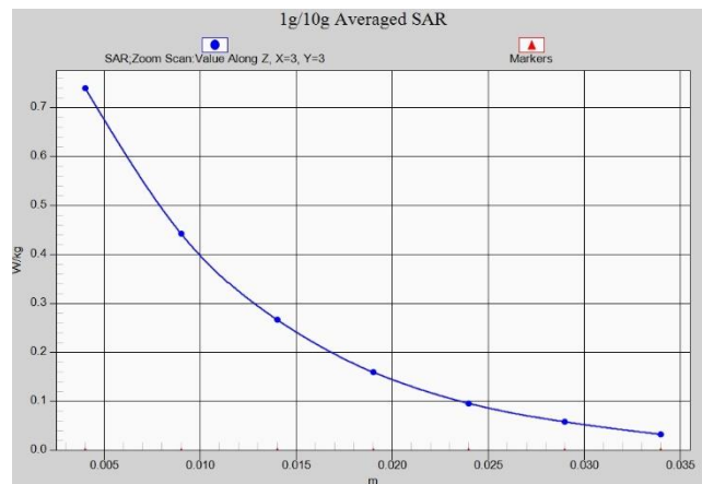
Fig. 1-51 Z-Scan at power reference point (n25)
