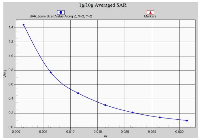
Fig. 1-31 Z-Scan at power reference point (LTE Band26)
