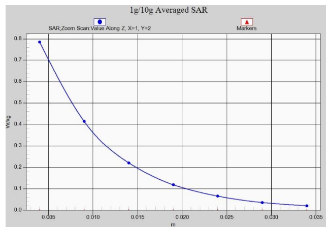
Fig. 1-47 Z-Scan at power reference point (n2)
