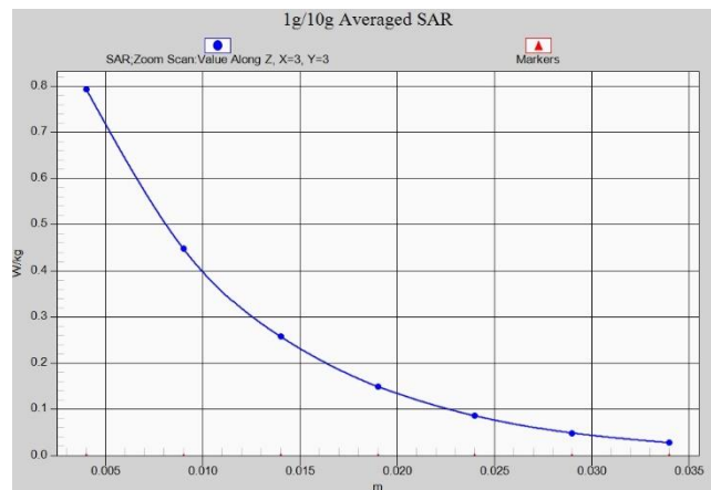
Fig. 1-48 Z-Scan at power reference point (n2)
