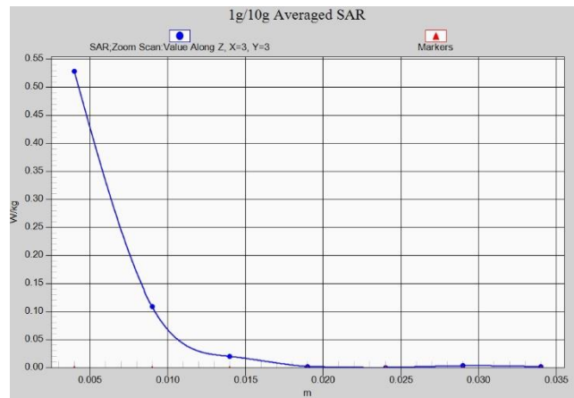
Fig. 1-46 Z-Scan at power reference point (wifi5G)
