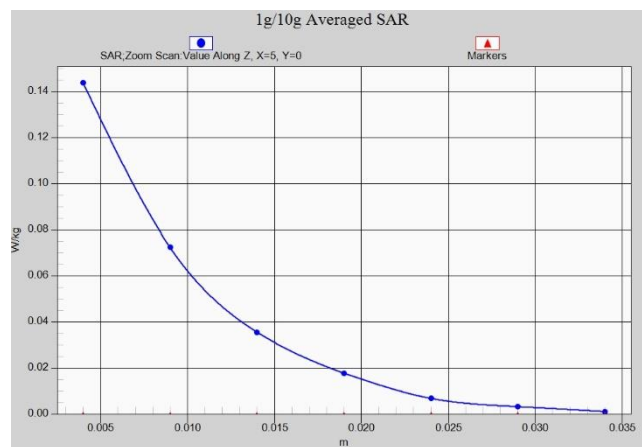
Fig. 1-44 Z-Scan at power reference point (wifi2450)
