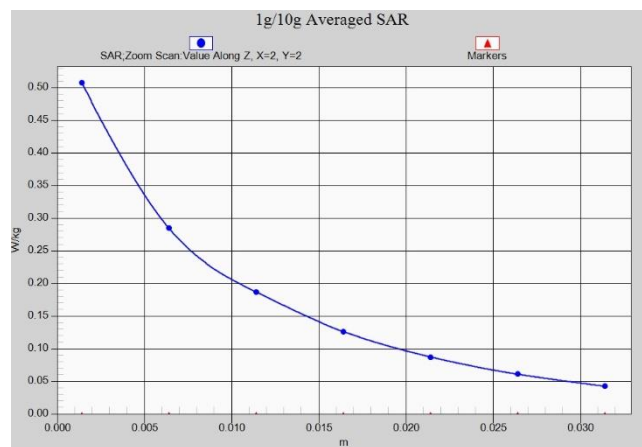
Fig. 1-26 Z-Scan at power reference point (LTE Band13)
