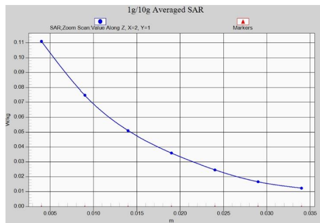
Fig. 1-50 Z-Scan at power reference point (n25)
