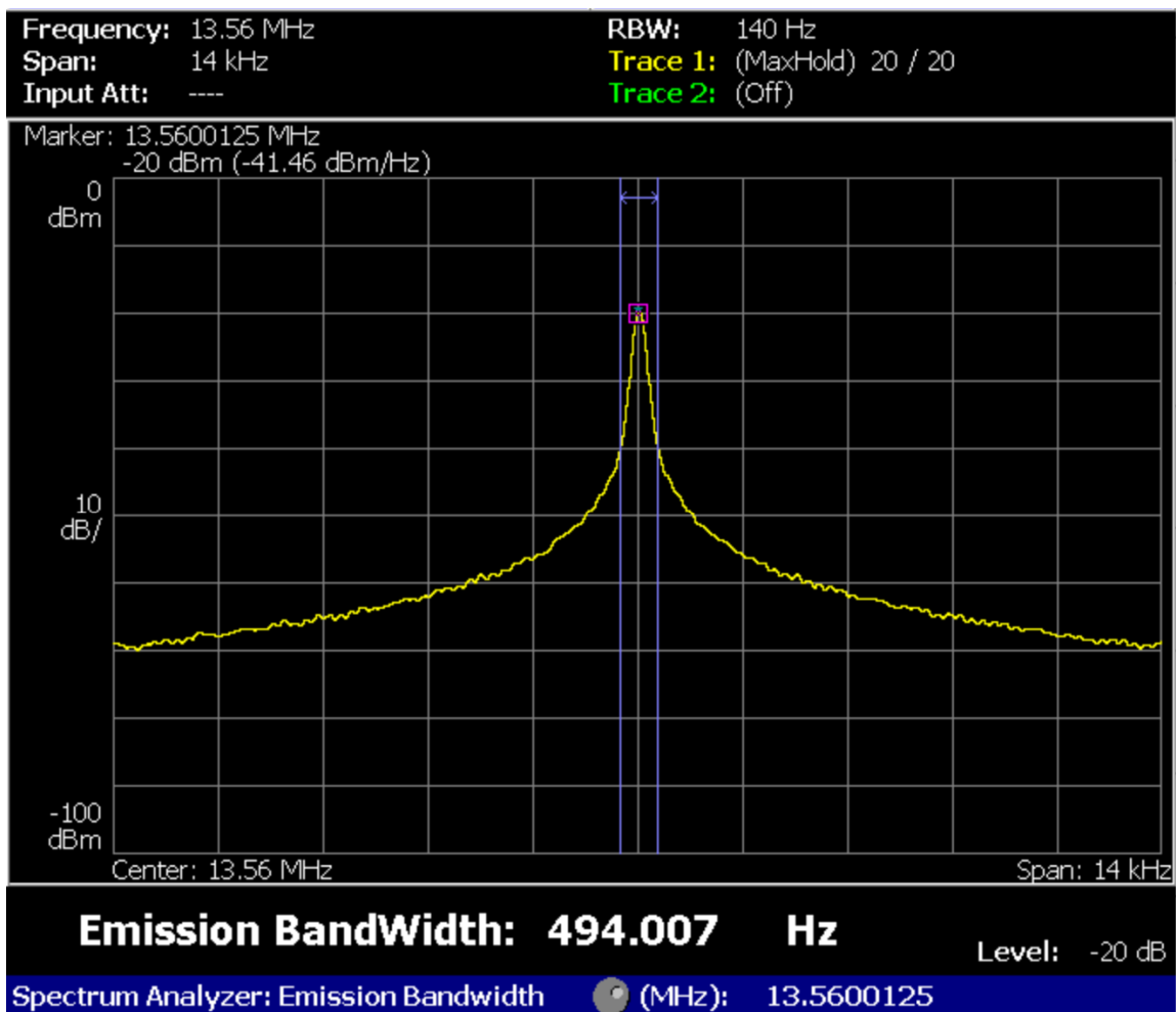
Figure B-9: Measurement results for 20dB Bandwidth
