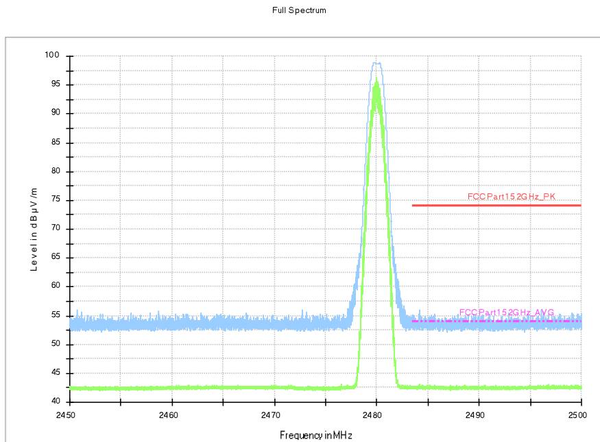
Fig.4. Frequency Band Edges: GFSK, Channel 39, 2.45 GHz - 2.50GHz
