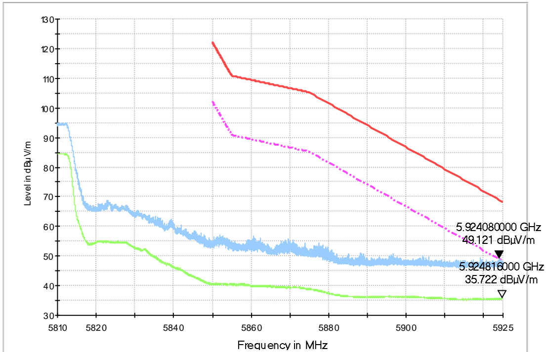
Fig. 90 Band Edges (802.11n-HT40, 5795MHz)
