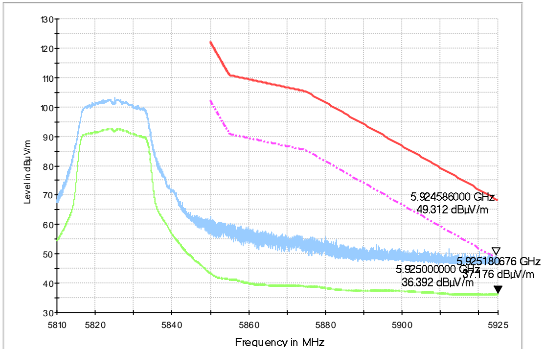
Fig. 88 Band Edges (802.11ac-HT20, 5825MHz)
