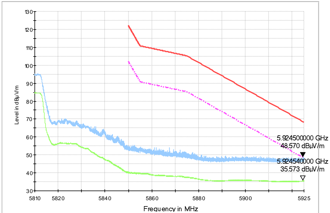
Fig. 92 Band Edges (802.11ac-HT40, 5795MHz)
