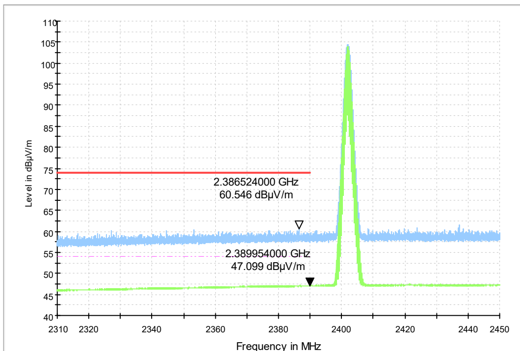
RE - Power-2.31GHz-2.45GHz
