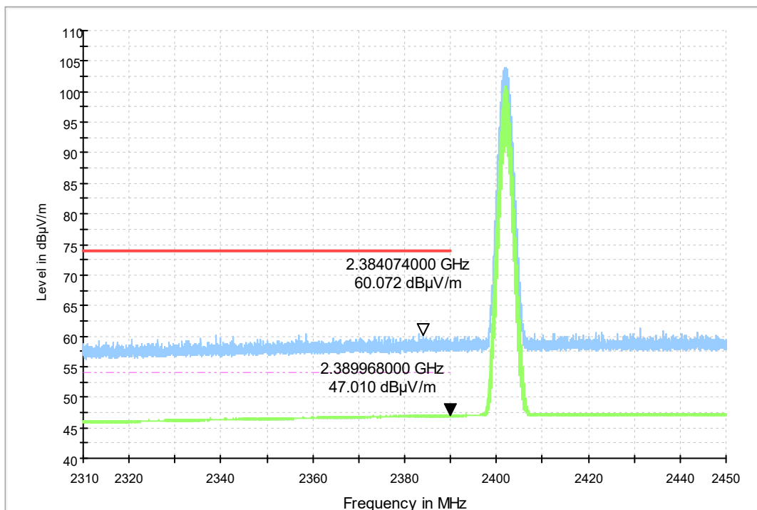
RE - Power-2.31GHz-2.45GHz
