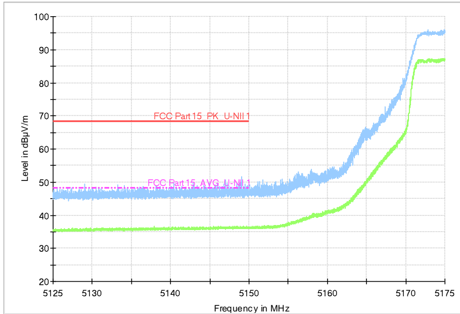
Fig.58 Band Edges (802.11n-HT20, 5180MHz)
