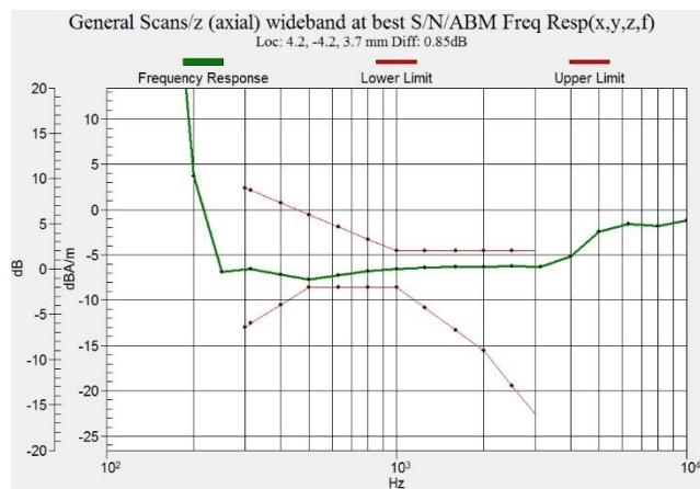
Figure C.2 Frequency Response of WCDMA 850
