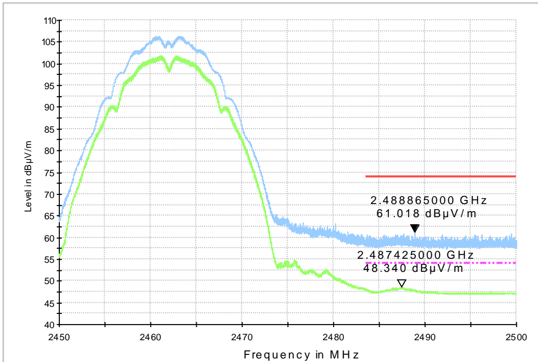
Fig.A.5.10 Transmitter Spurious Emission - Radiated Band edge: 802.11b, ch11, 2.45 GHz - 2.50GHz
