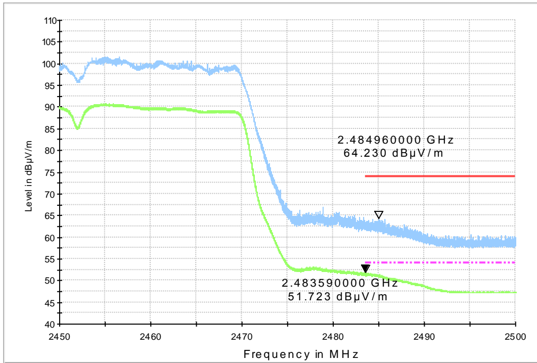
Fig.A.5.16 Transmitter Spurious Emission - Radiated Band edge: 802.11n-HT40, ch9, 2.45 GHz - 2.50GHz
