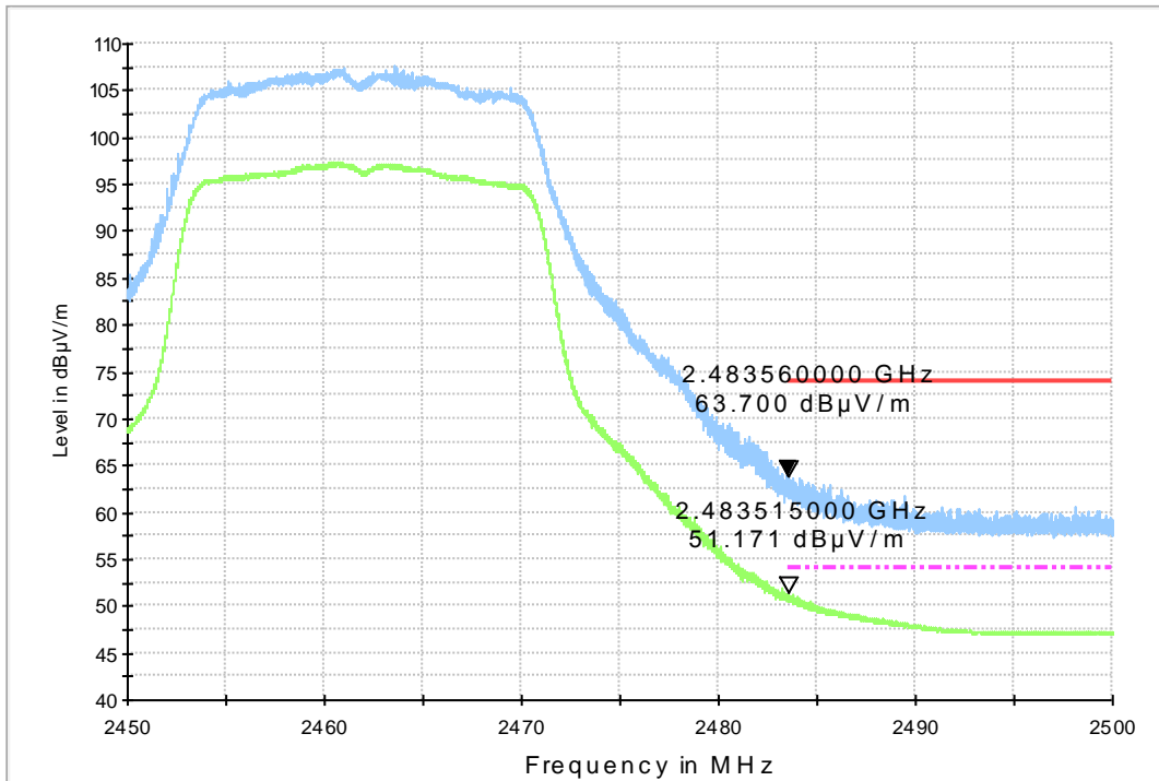
Fig.A.5.14 Transmitter Spurious Emission - Radiated Band edge: 802.11n-HT20, ch11, 2.45 GHz - 2.50GHz
