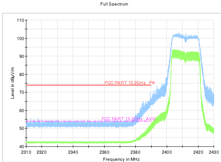
Fig.A.6.2.1 Transmitter Spurious Emission - Radiated (Power): 802.11n-HT20, ch1, 2.31 GHz - 2.43GHz
