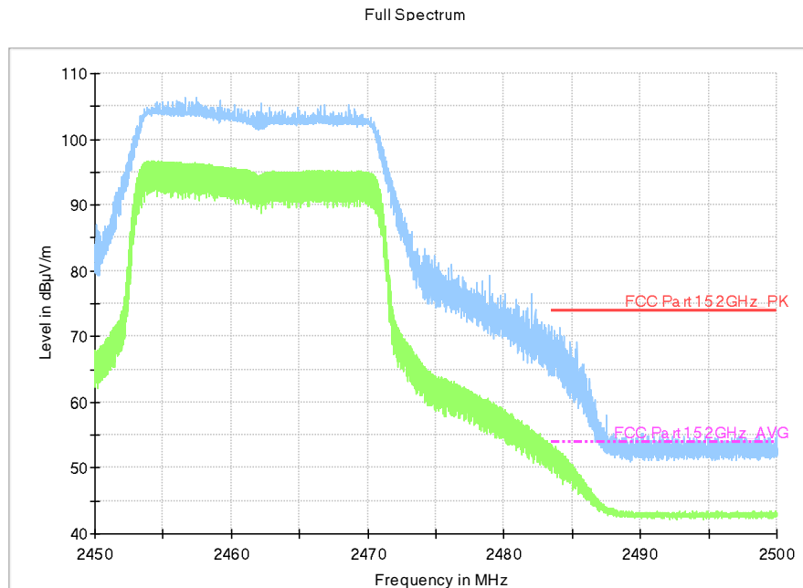
Fig.A.6.2.2 Transmitter Spurious Emission - Radiated (Power): 802.11n-HT20, ch11, 2.45 GHz - 2.50GHz
