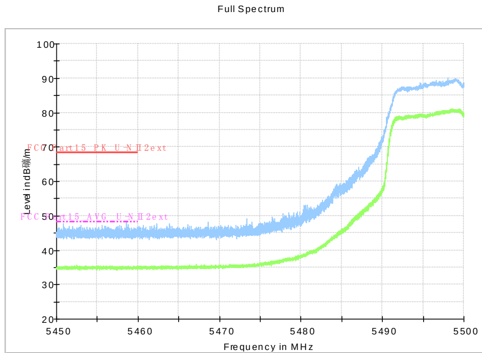
Fig.66 Band Edges (802.11ac-HT20, 5500MHz)
