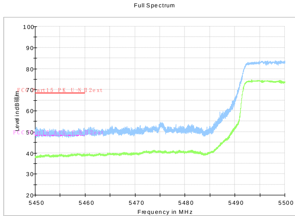
Fig.84 Band Edges (802.11ac-HT80, 5530MHz)
