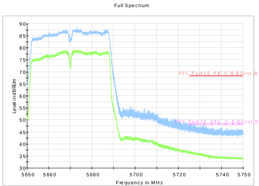
Fig.73 Band Edges (802.11n-HT40, 5670MHz)
