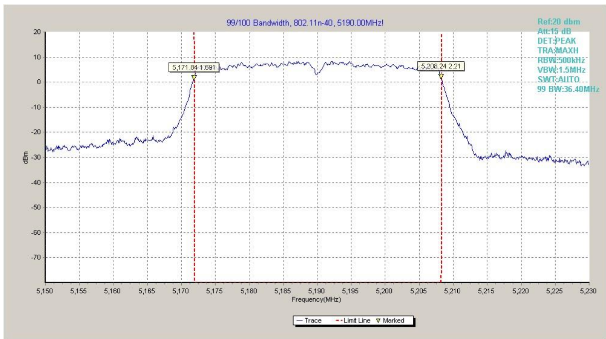
Fig.98 99% Occupied bandwidth (802.11n-HT40, 5190MHz)
