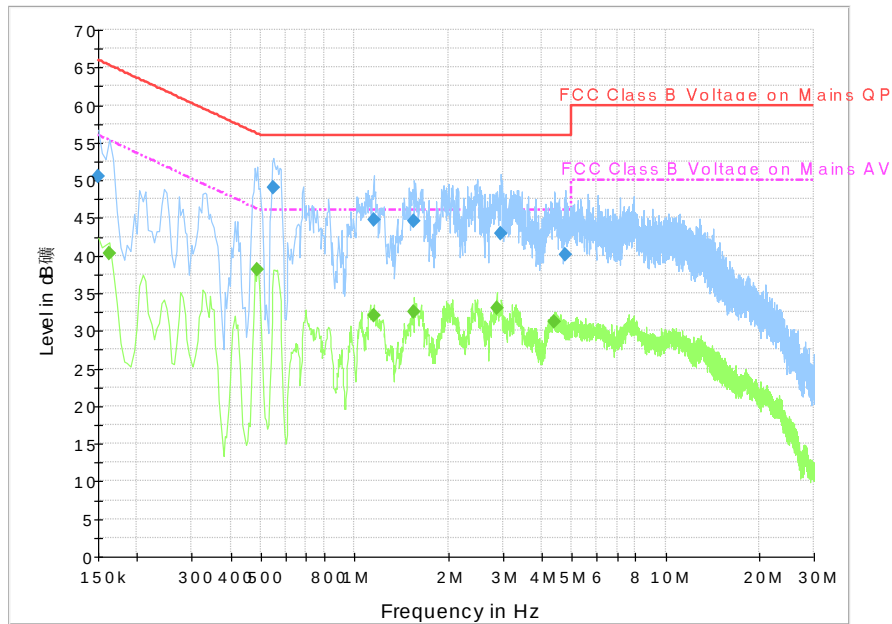
Fig.88 Conducted Emission(802.11a, IDLE)
