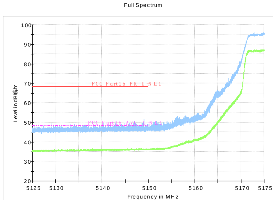
Fig.58 Band Edges (802.11n-HT20, 5180MHz)
