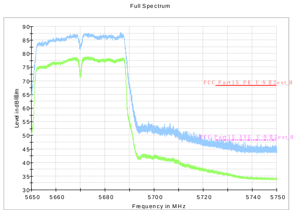
Fig.79 Band Edges (802.11ac-HT40, 5670MHz)
