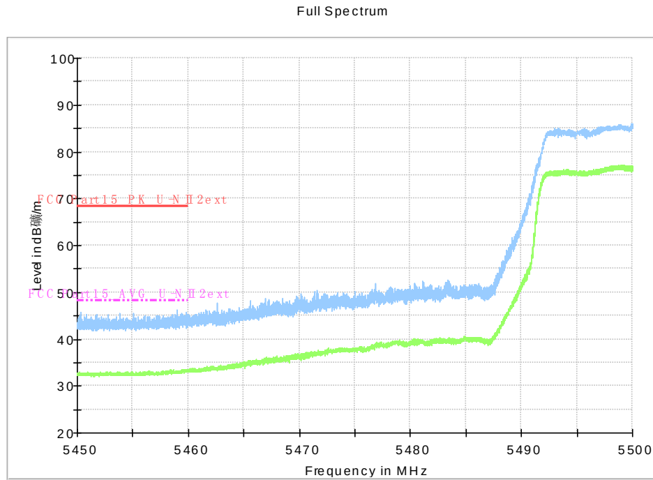
Fig.72 Band Edges (802.11n-HT40, 5510MHz)
