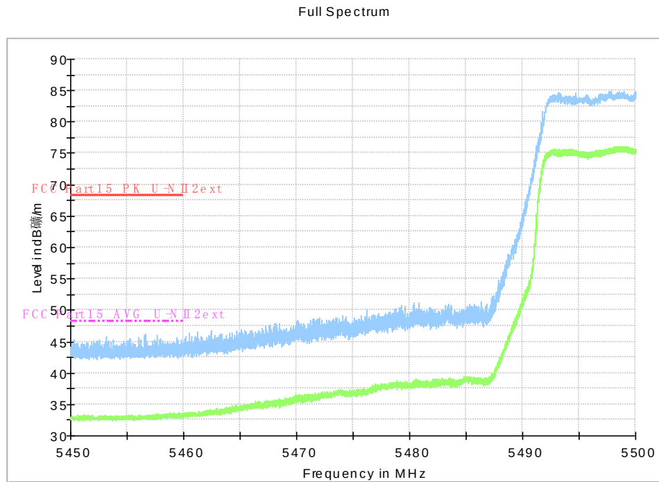
Fig.78 Band Edges (802.11ac-HT40, 5510MHz)
