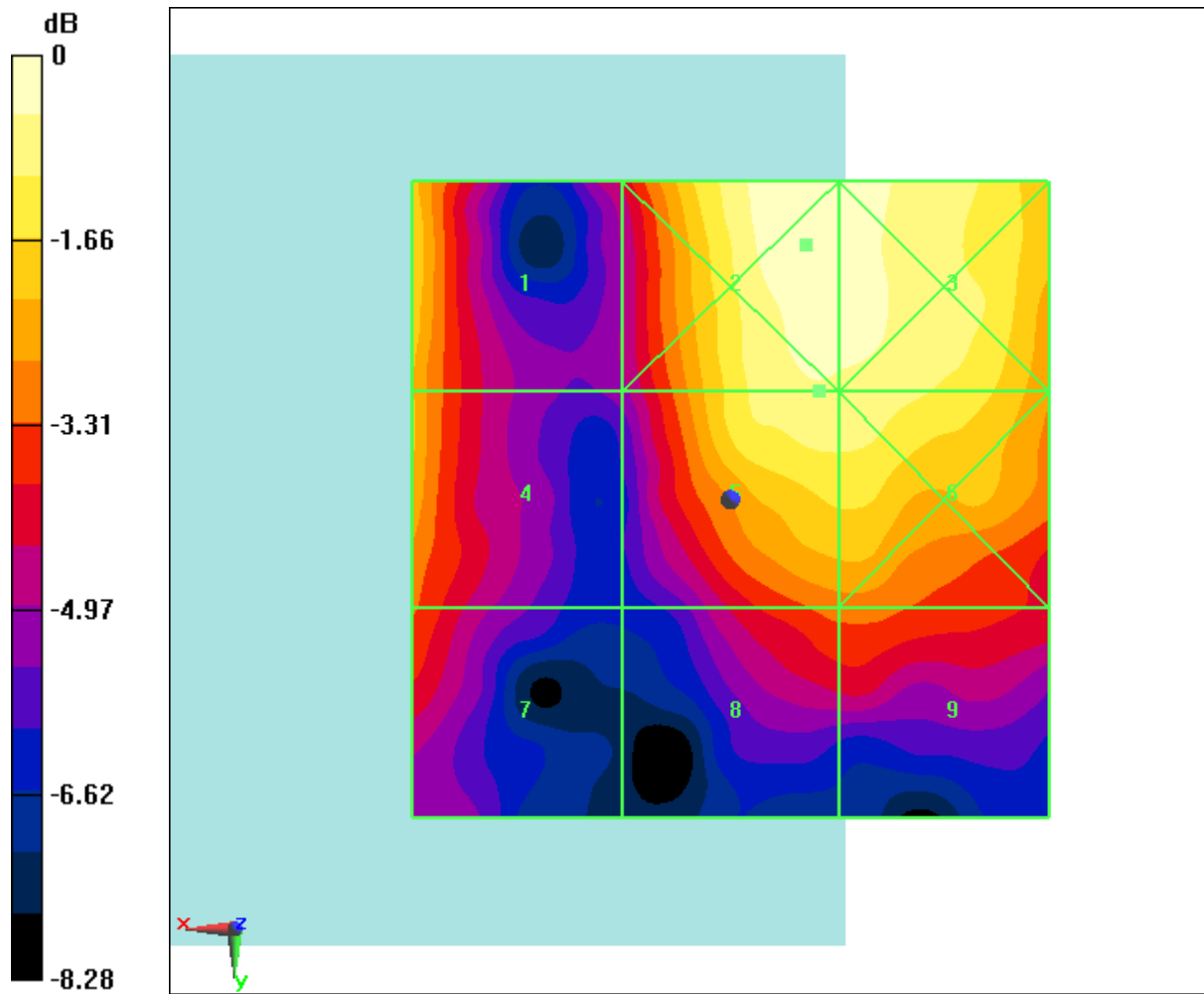
Fig B.7 HAC RF E-Field LTE Band41 QPSK CH41490
