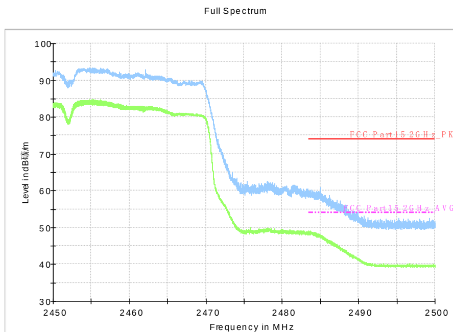
Fig.A.6.2.8 Transmitter Spurious Emission - Radiated (Power): 802.11n-HT740, ch9, 2.45 GHz - 2.50GHz
