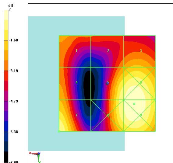
Fig B.16 HAC RF E-Field LTE Band41 Power Class 2 QPSK CH41490
