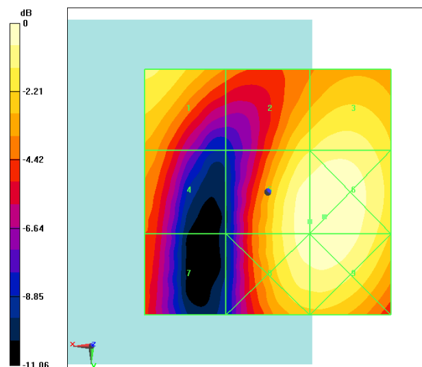
Fig B.27 HAC RF E-Field LTE Band41 Power Class 3 QPSK CH41055
