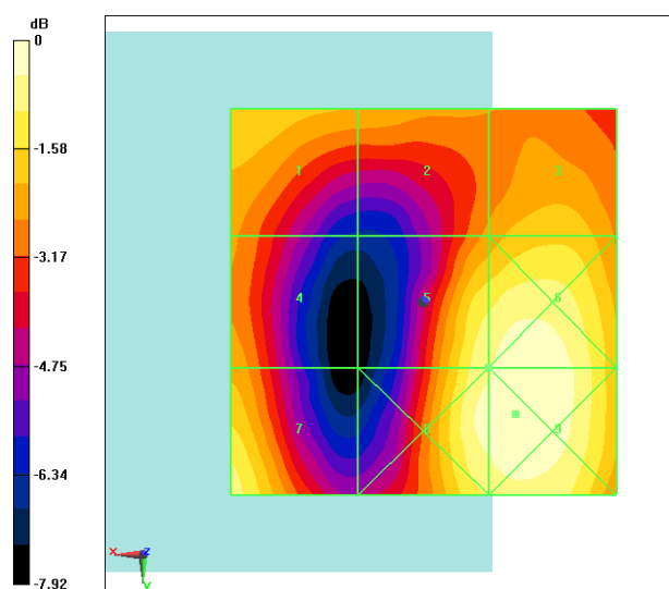
Fig B.32 HAC RF E-Field LTE Band41 Power Class 3 16QAM CH41055
