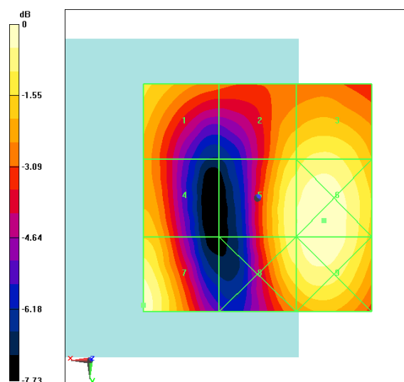
Fig B.18 HAC RF E-Field LTE Band41 Power Class 2 QPSK CH40620
