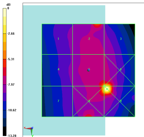
Fig B.14 HAC RF E-Field CDMA BC10 Middle
