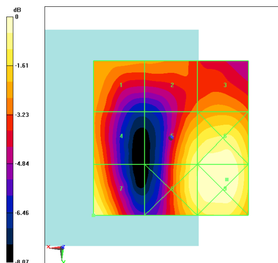
Fig B.21 HAC RF E-Field LTE Band41 Power Class 2 16QAM CH41490
