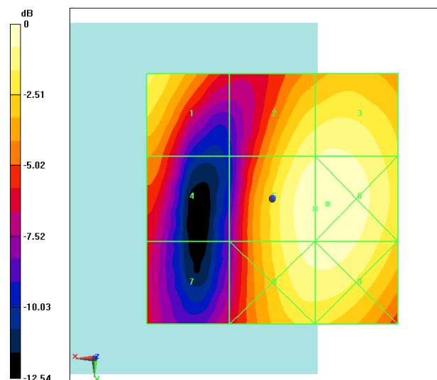
Fig B.29 HAC RF E-Field LTE Band41 Power Class 3 QPSK CH40185
