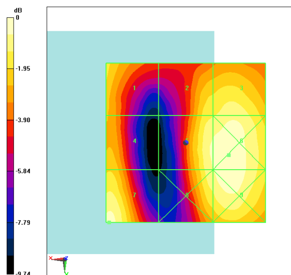
Fig B.24 HAC RF E-Field LTE Band41 Power Class 2 16QAM CH40185
