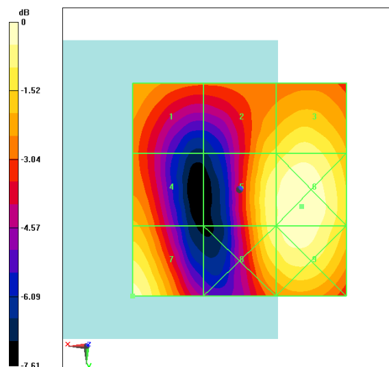
Fig B.17 HAC RF E-Field LTE Band41 Power Class 2 QPSK CH41055
