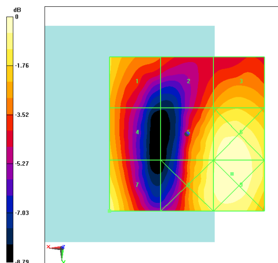
Fig B.34 HAC RF E-Field LTE Band41 Power Class 3 16QAM CH40185
