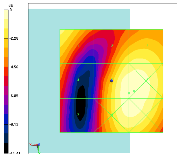
Fig B.28 HAC RF E-Field LTE Band41 Power Class 3 QPSK CH40620
