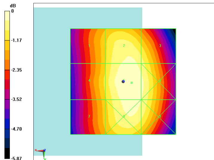
Fig B.1 HAC RF E-Field GSM 850 High
