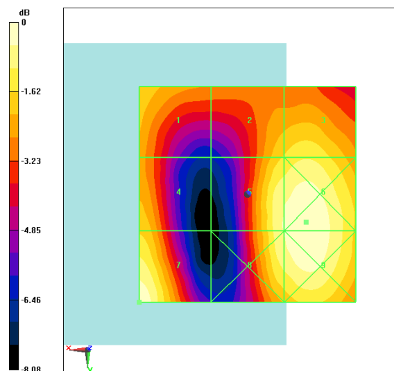
Fig B.23 HAC RF E-Field LTE Band41 Power Class 2 16QAM CH40620
