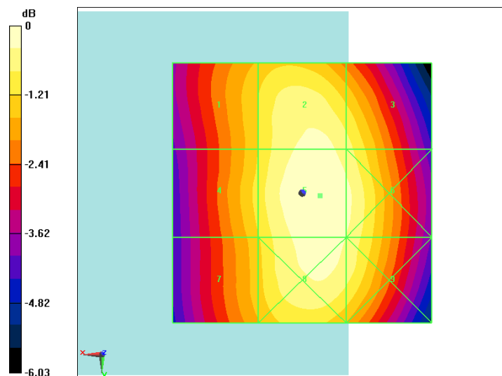
Fig B.2 HAC RF E-Field GSM 850 Middle
