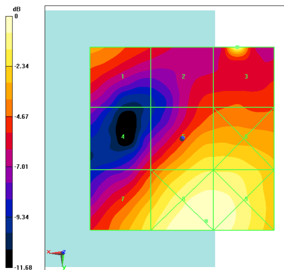
Fig B.12 HAC RF E-Field CDMA BC1 Low
