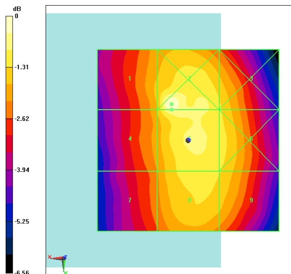
Fig B.13 HAC RF E-Field CDMA BC10 High
