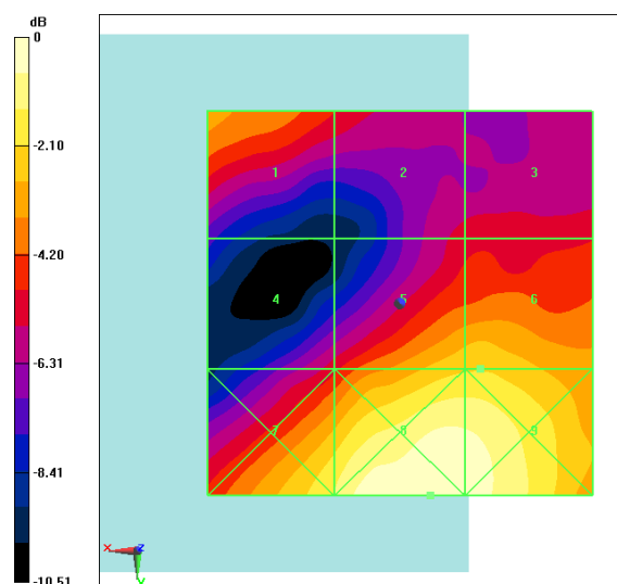
Fig B.11 HAC RF E-Field CDMA BC1 Middle
