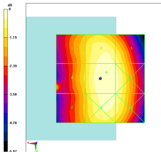
Fig B.15 HAC RF E-Field CDMA BC10 Low
