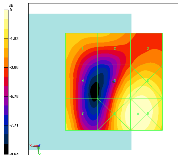
Fig B.31 HAC RF E-Field LTE Band41 Power Class 3 16QAM CH41490
