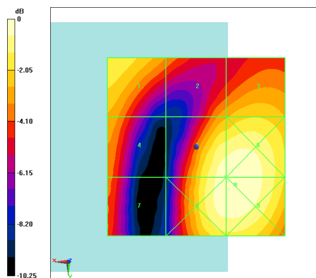
Fig B.26 HAC RF E-Field LTE Band41 Power Class 3 QPSK CH41490
