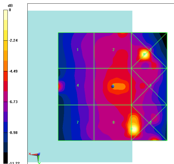
Fig B.7 HAC RF E-Field CDMA BC0 High
