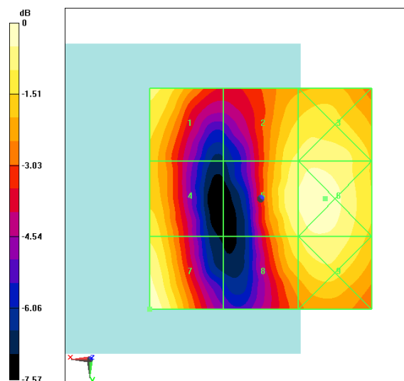
Fig B.35 HAC RF E-Field LTE Band41 Power Class 3 16QAM CH3975
