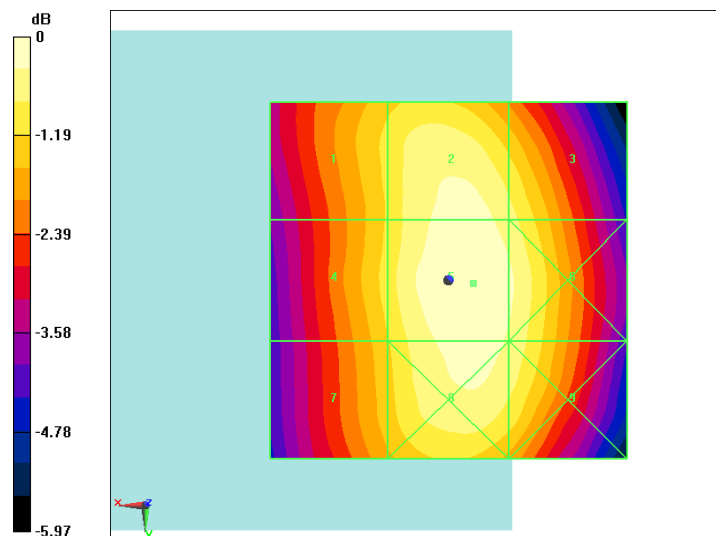
Fig B.3 HAC RF E-Field GSM 850 Low
