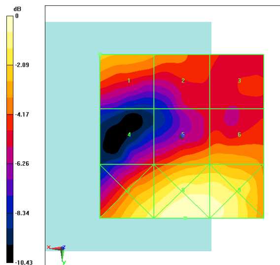
Fig B.10 HAC RF E-Field CDMA BC1 High
