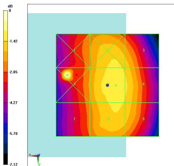
Fig B.8 HAC RF E-Field CDMA BC0 Middle
