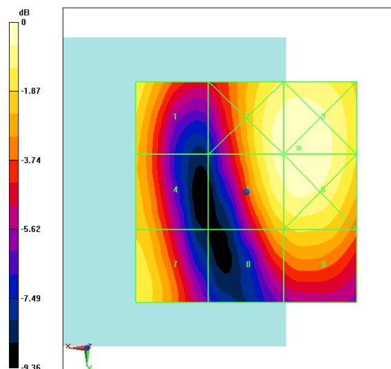
Fig B.20 HAC RF E-Field LTE Band41 Power Class 2 QPSK CH39750
