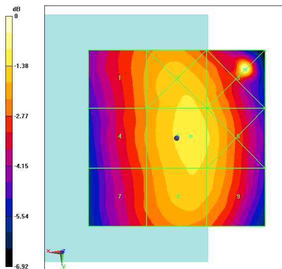
Fig B.9 HAC RF E-Field CDMA BC0 Low
