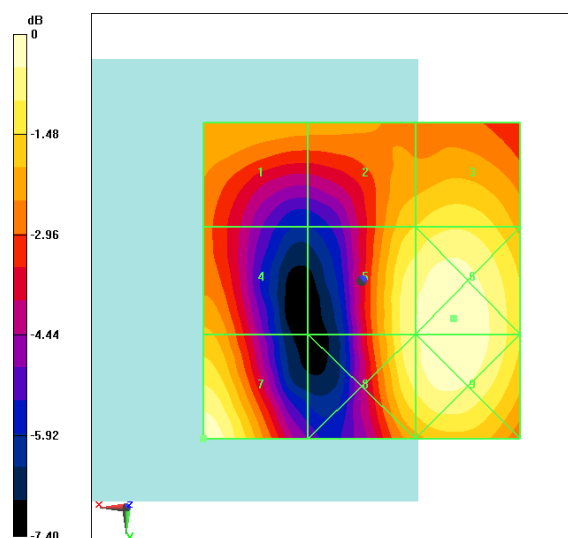
Fig B.22 HAC RF E-Field LTE Band41 Power Class 2 16QAM CH41055
