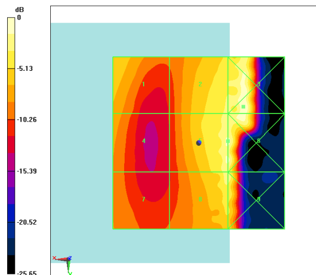
Fig B.30 HAC RF E-Field LTE Band41 Power Class 3 QPSK CH39750
