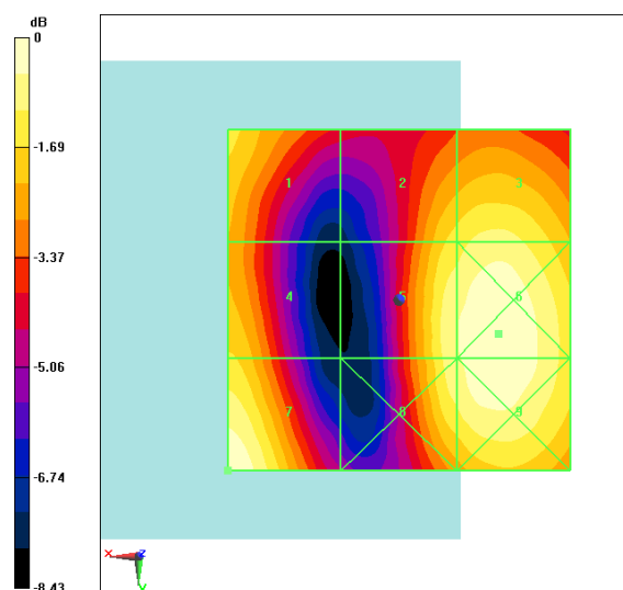
Fig B.25 HAC RF E-Field LTE Band41 Power Class 2 16QAM CH39750
