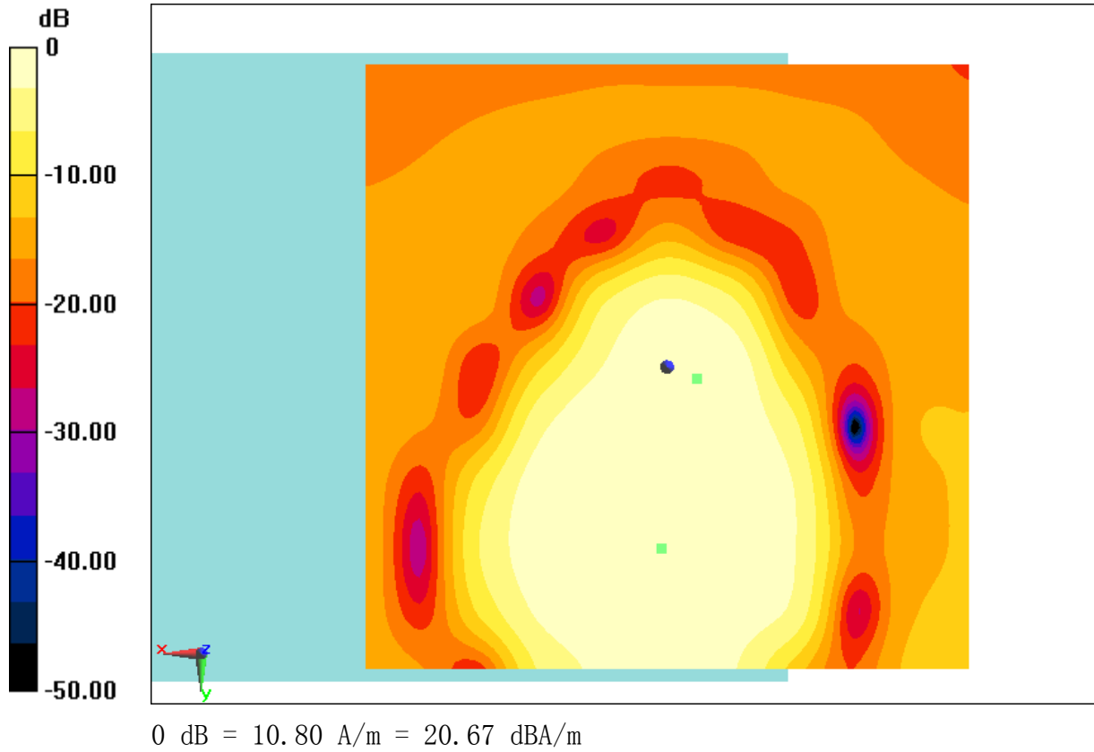
Fig B.18 T-Coil LTE B12
