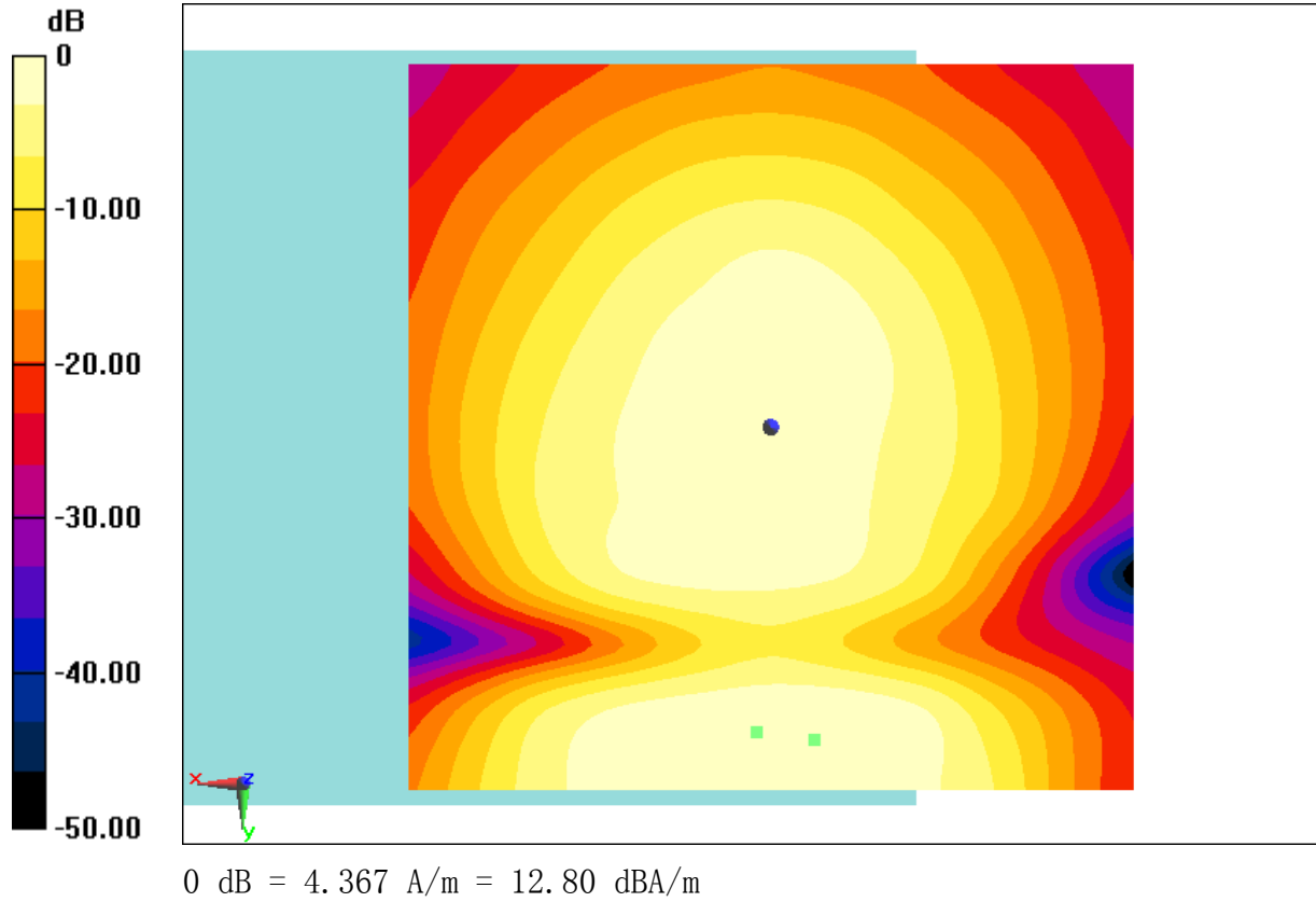
Fig B.17 T-Coil LTE B12
