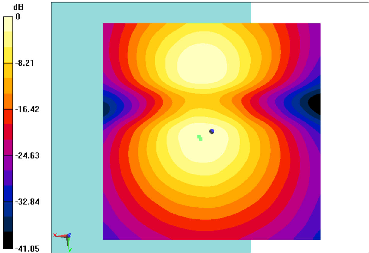
Fig B.19 T-Coil Wifi -2.4G
