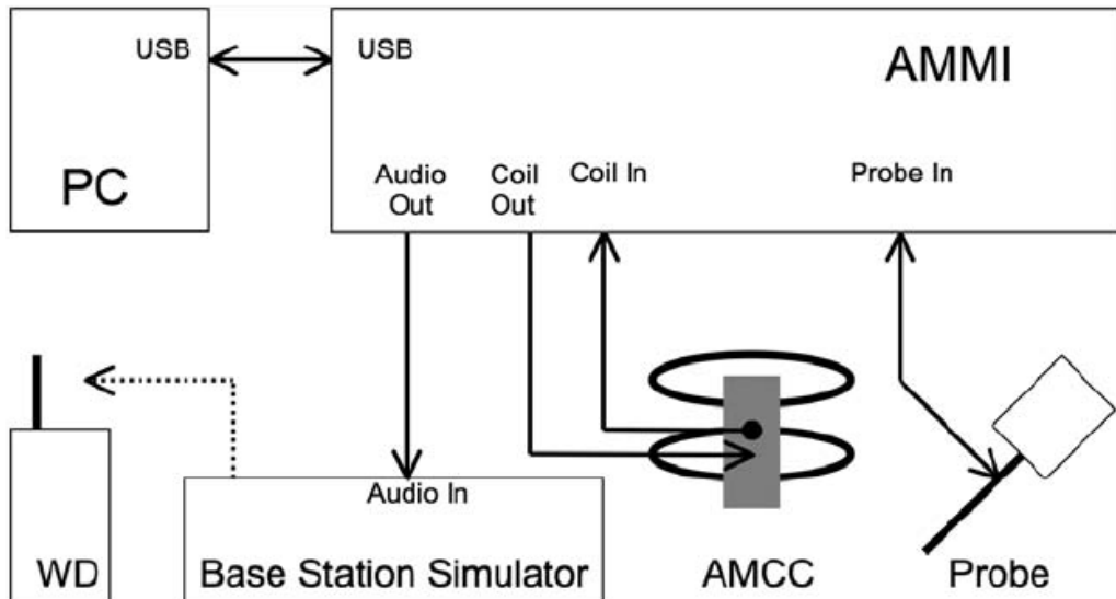
Figure 5.2T-Coil setup with HAC Test Arch and AMCC
