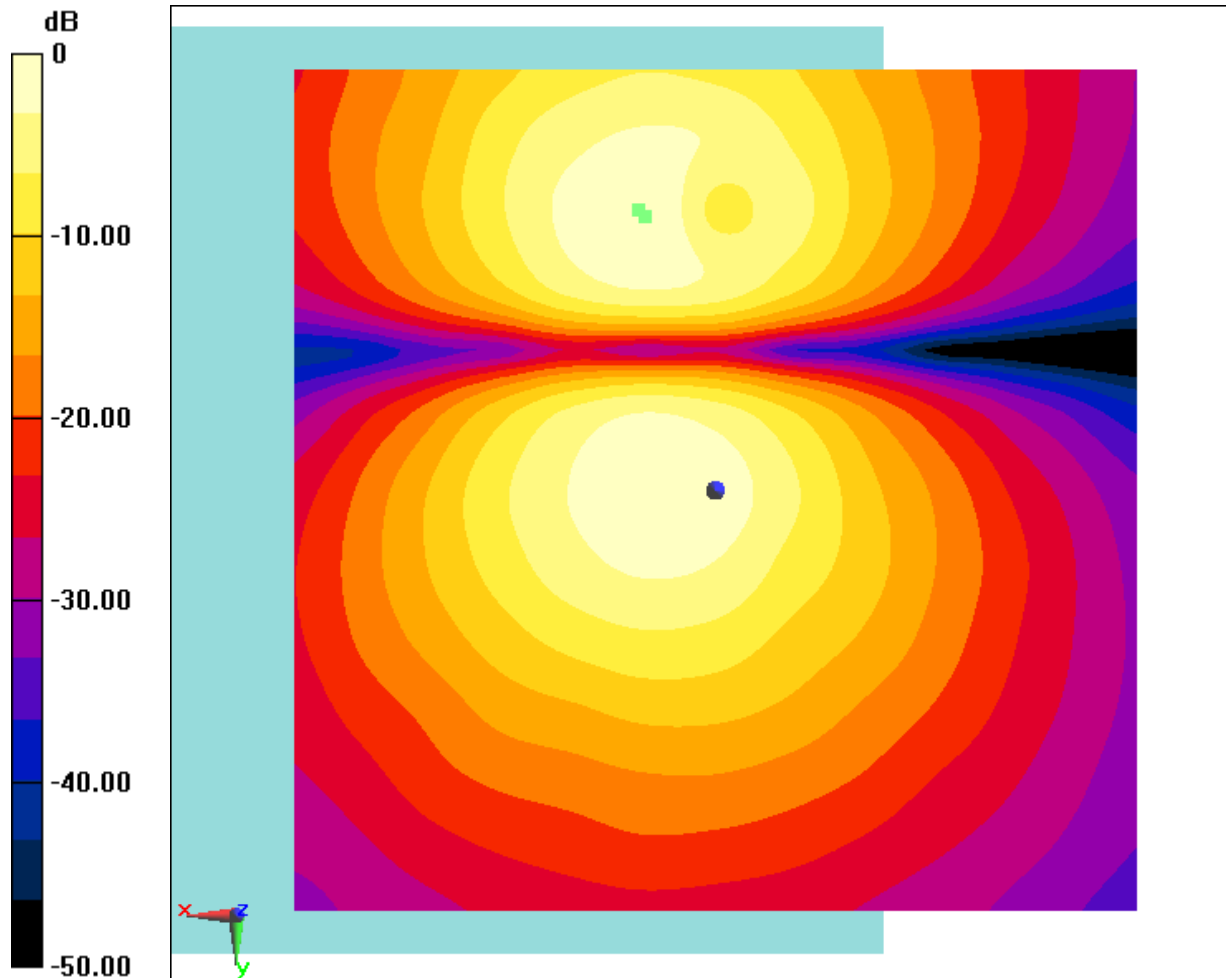
Fig B.11 T-Coil LTE B2
