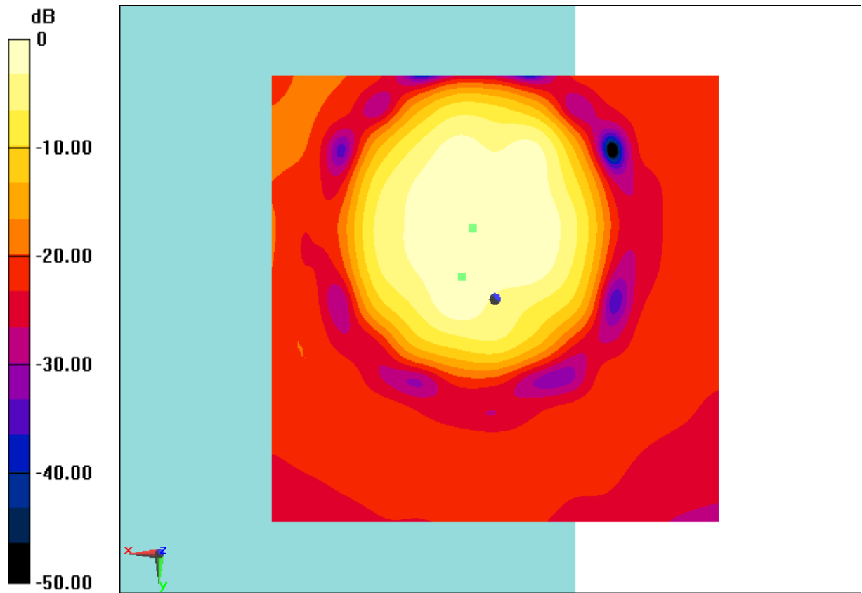
Fig B.20 T-Coil Wifi -2.4G
