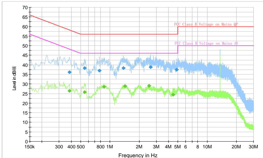
Figure A-5: Test result of EUT8 at test set. NFC01
