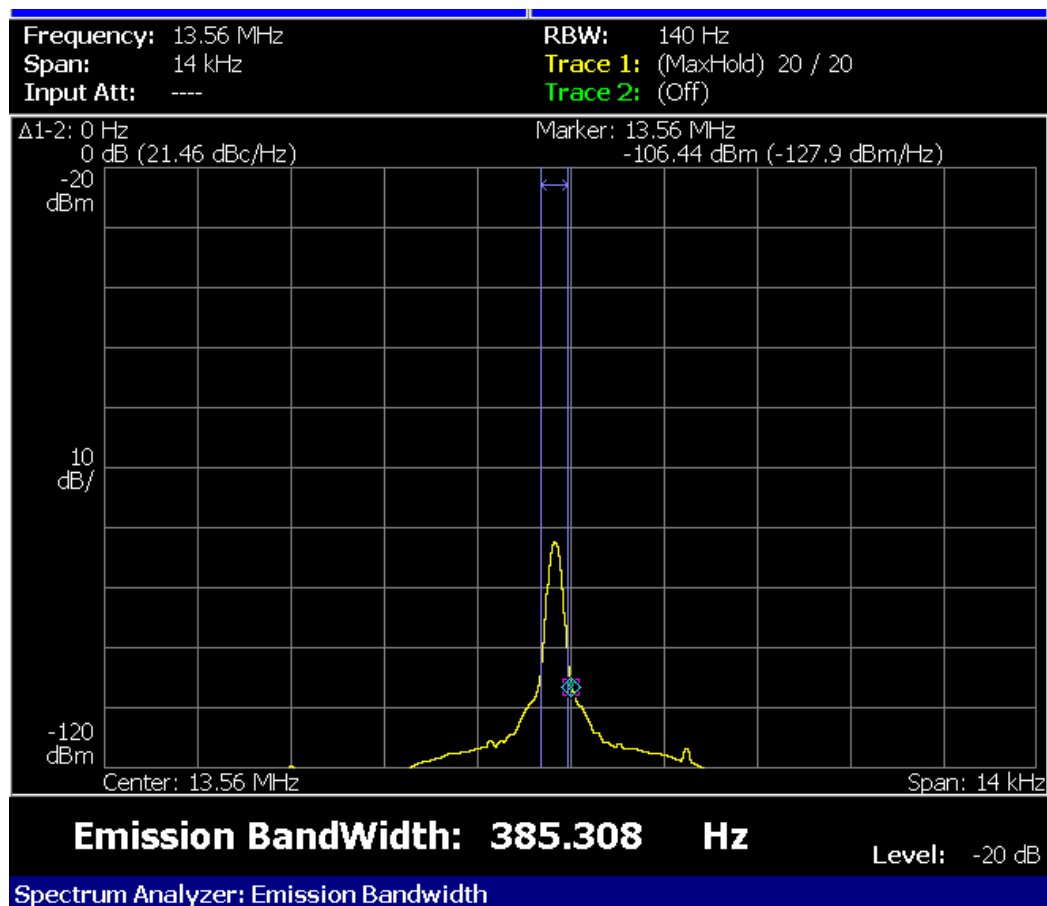
Figure A-4: Test result of EUT42 at test set. NFC02
