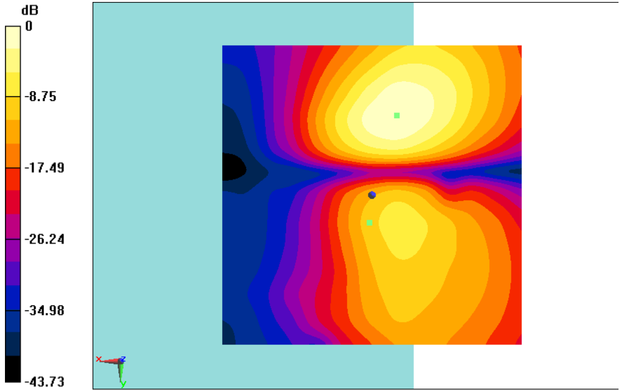
Fig B.13 T-coil LTE Band4
