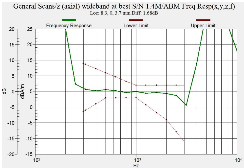
Figure C.7 Frequency Response of LTE B4
