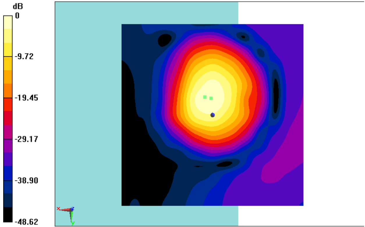
Fig B.20 T-coil LTE Band26
