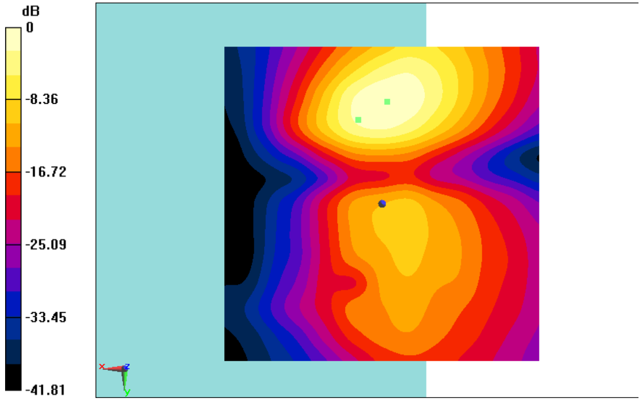
Fig B.19 T-coil LTE Band26
