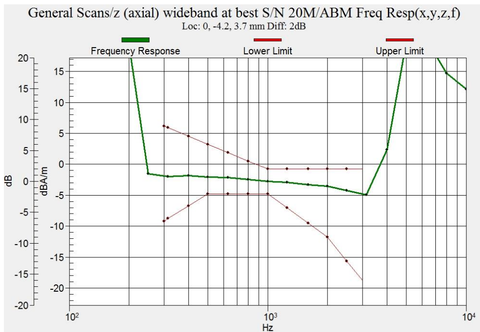
Figure C.10 Frequency Response of LTE B26
