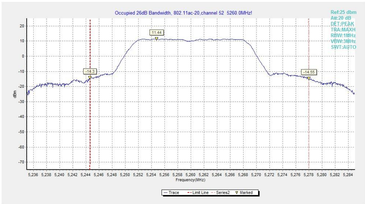
Fig. 22 Occupied 26dB Bandwidth (802.11ac-HT20, 5260MHz)
