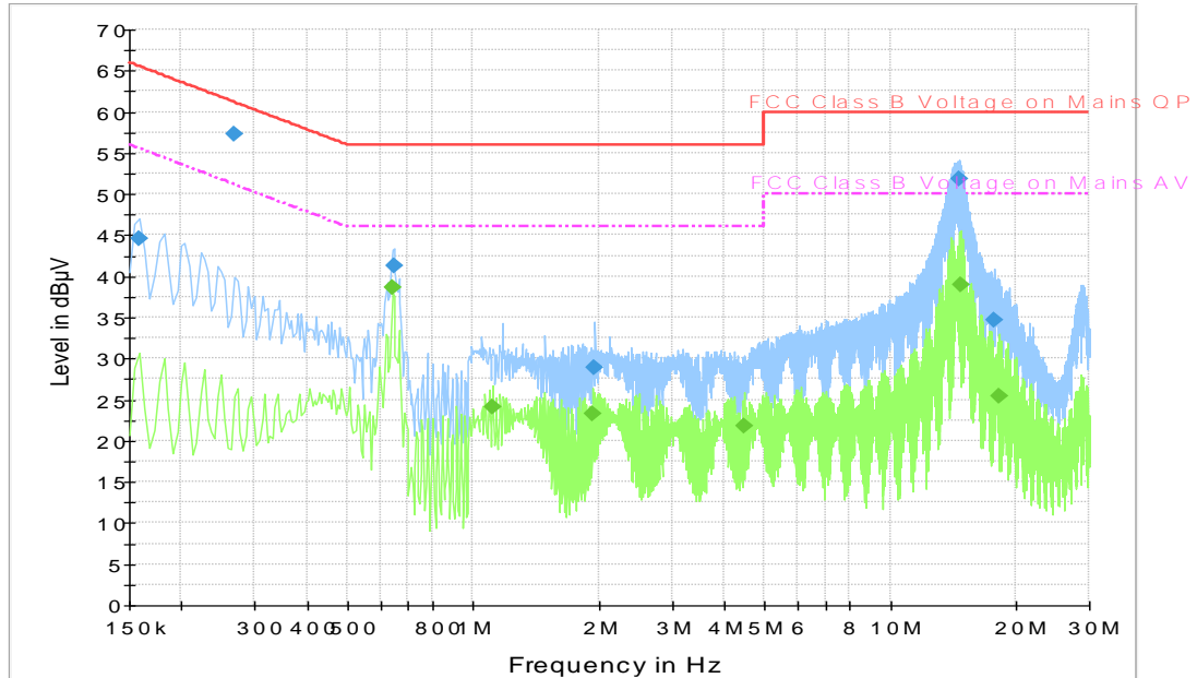
Figure A.14 Conducted Emission
