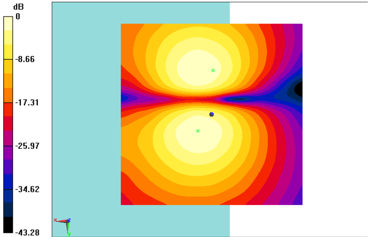
Fig B.21 T-Coil LTE B26
