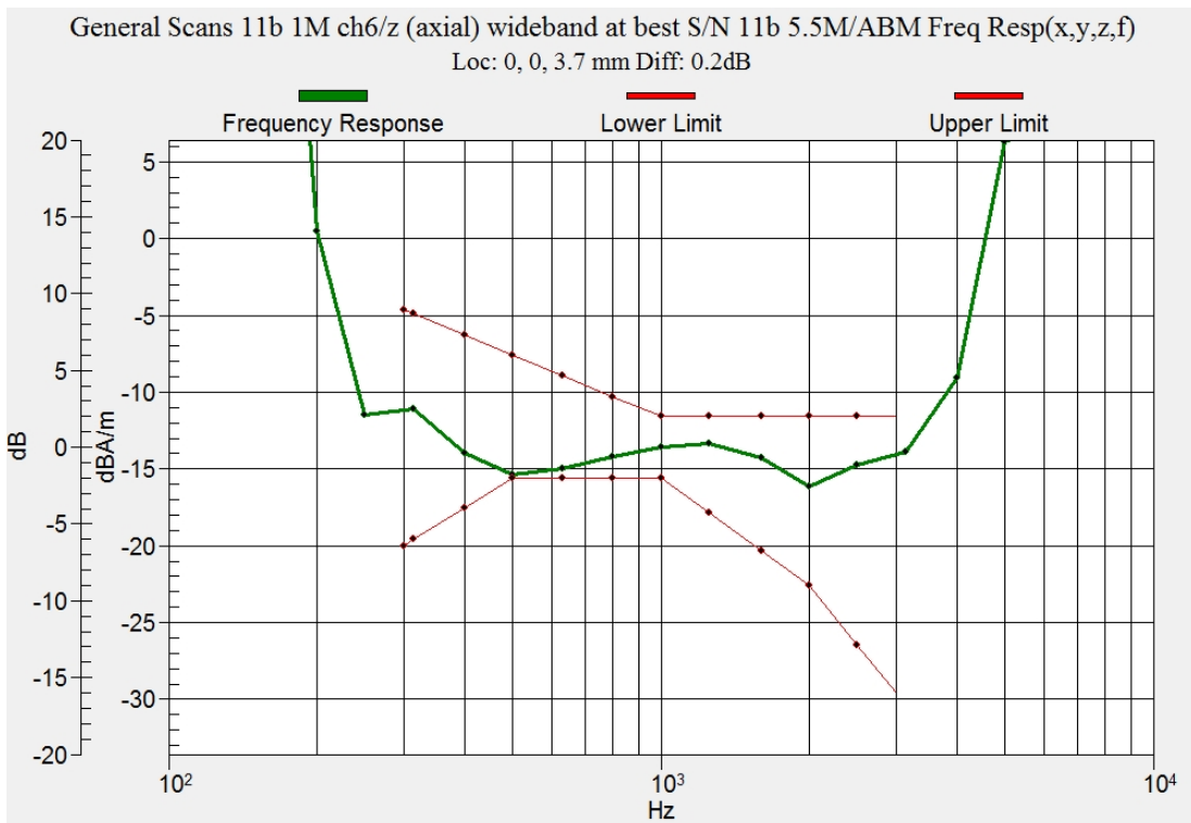
Figure C.13 Frequency Response of WiFi-2.4G
