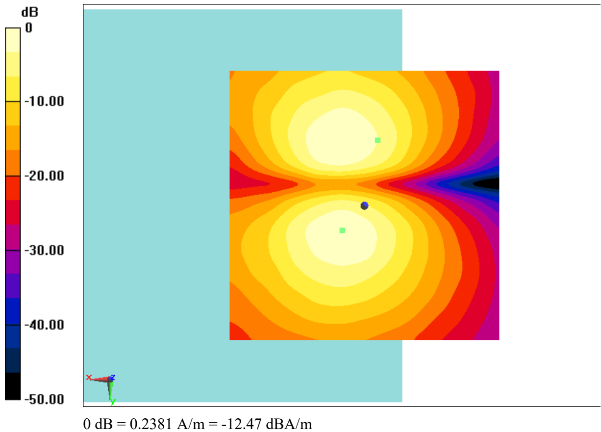
Fig B.23 T-Coil LTE B41
