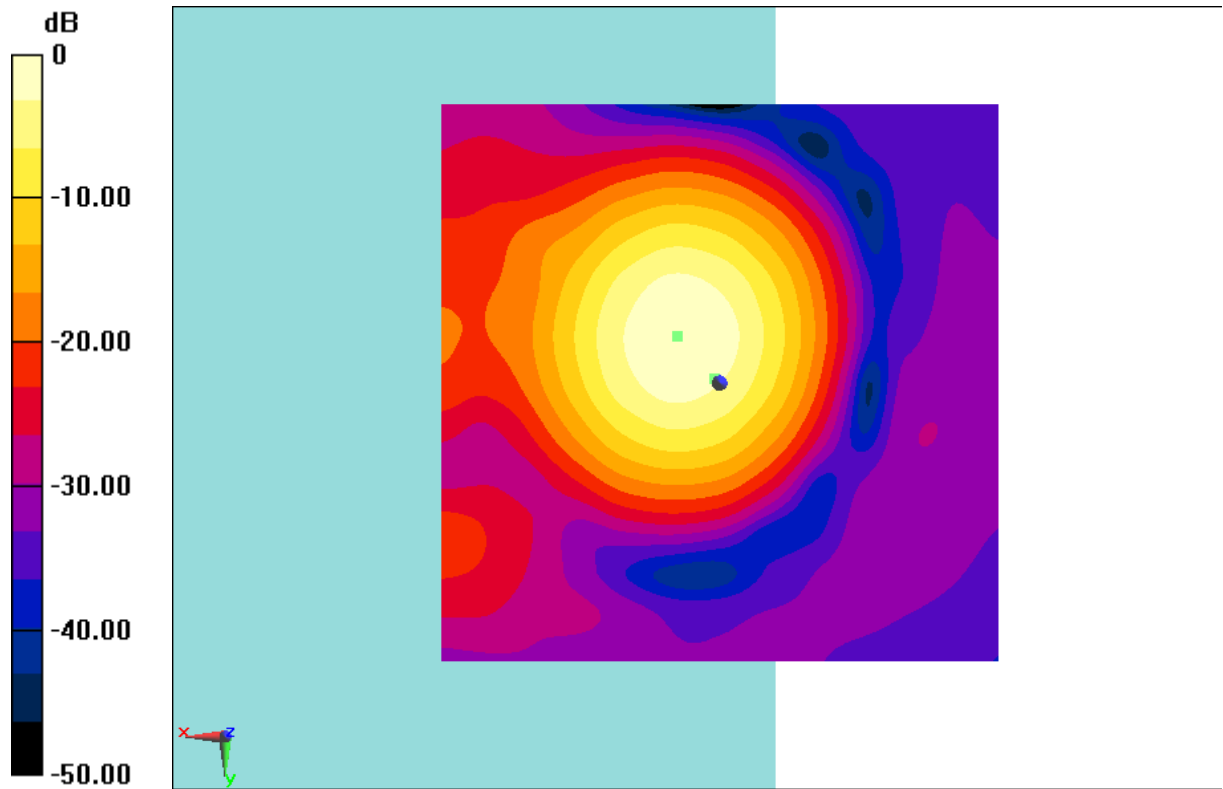
Fig B.22 T-Coil LTE B26
