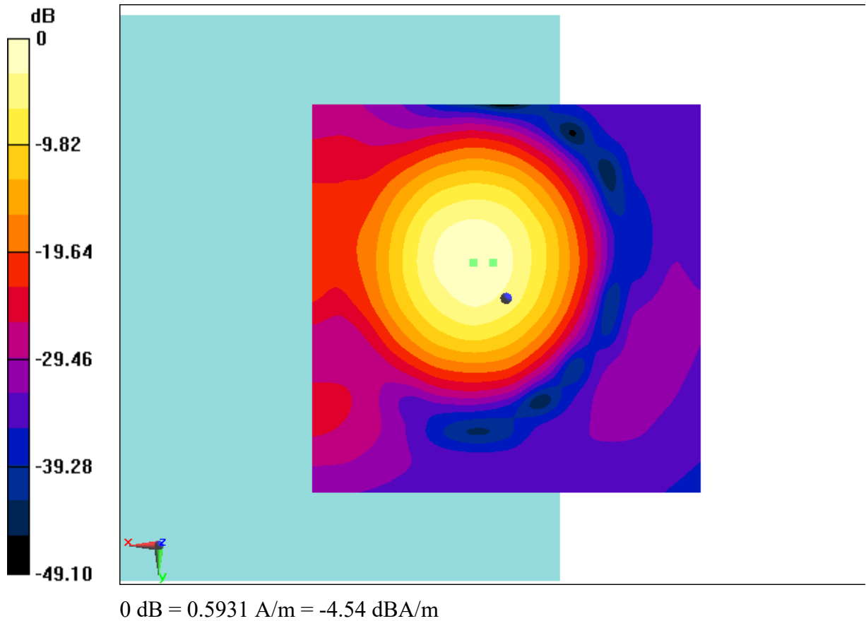
Fig B.24 T-Coil LTE B41
