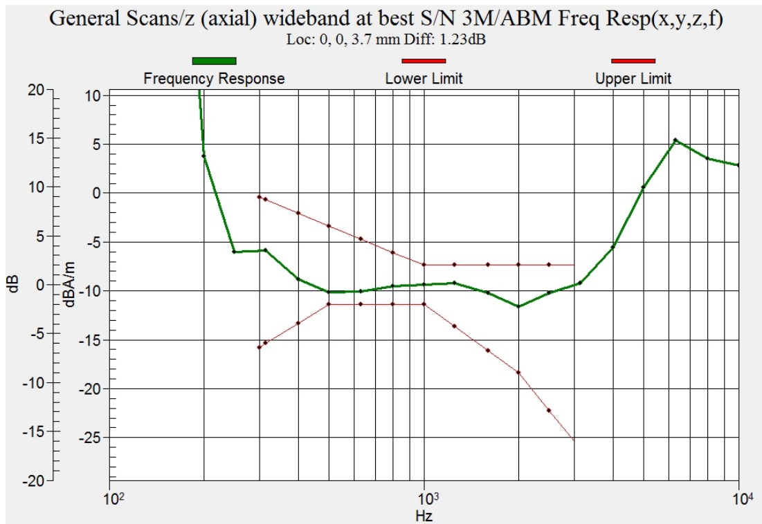
Figure C.11 Frequency Response of LTE B26
