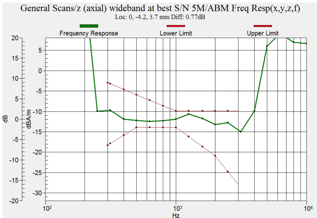
Figure C.12 Frequency Response of LTE B41
