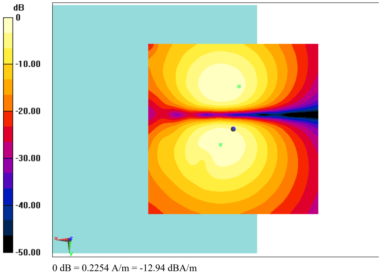
Fig B.27 T-Coil WiFi-5G
