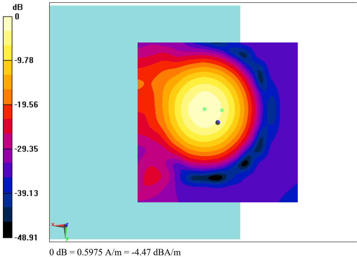
Fig B.26 T-Coil WiFi-2.4G
