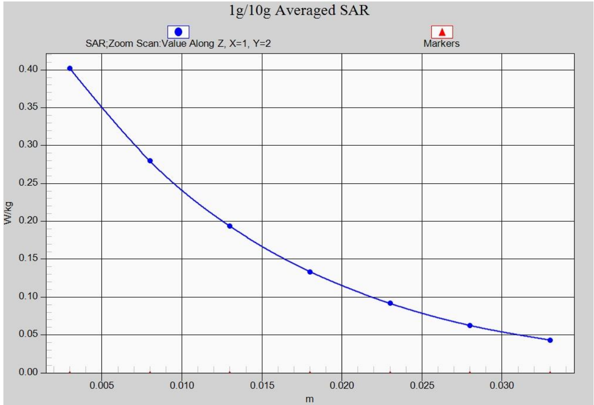
Fig. 30-1 Z-Scan at power reference point (LTE Band 26)
