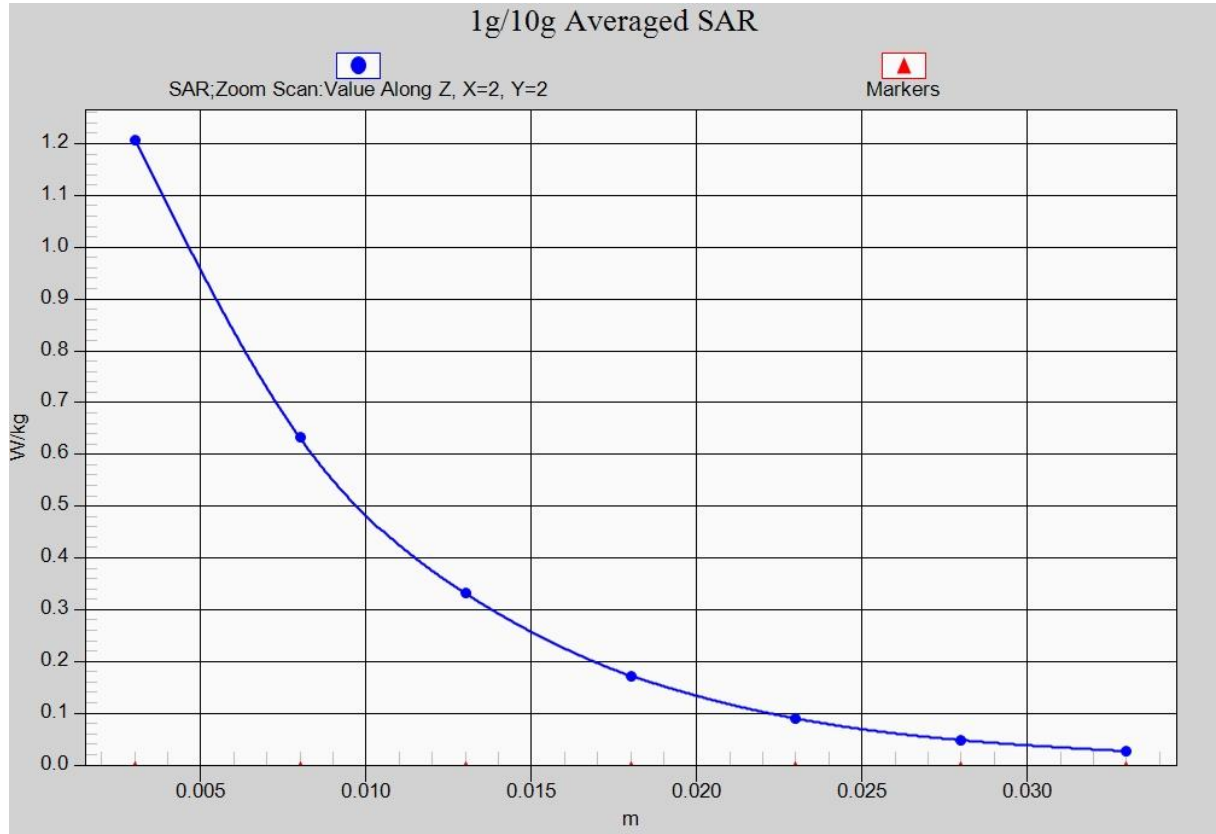
Fig. 25-1 Z-Scan at power reference point (LTE Band 41)
