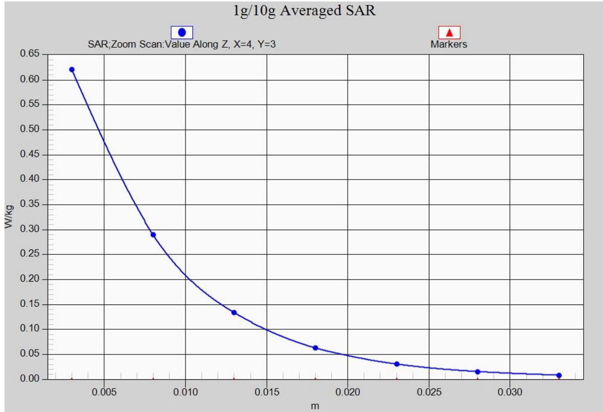
Fig. 31-1 Z-Scan at power reference point (2450 MHz)
