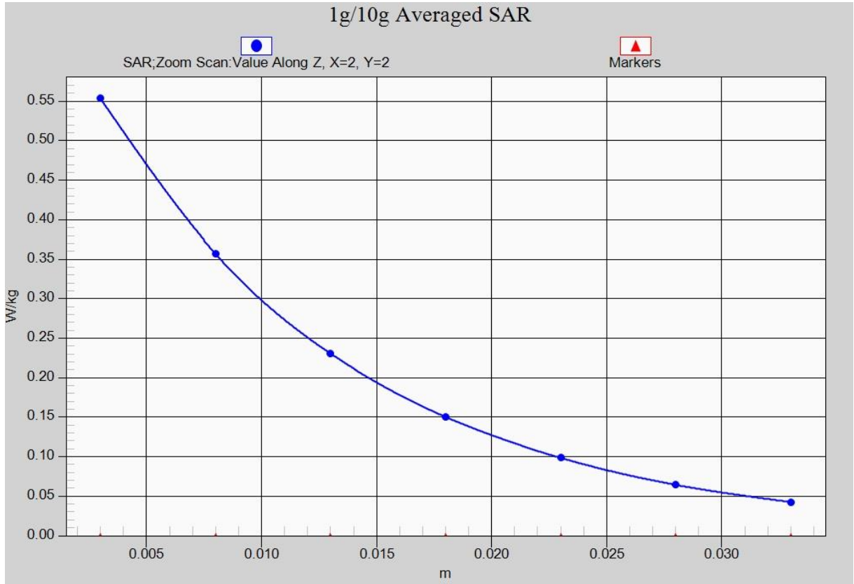
Fig. 28-1 Z-Scan at power reference point (LTE Band4)
