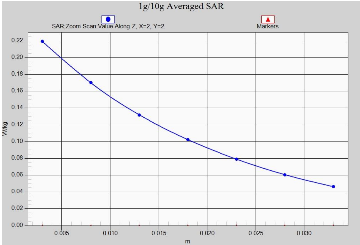
Fig. 29-1 Z-Scan at power reference point (LTE Band 26)
