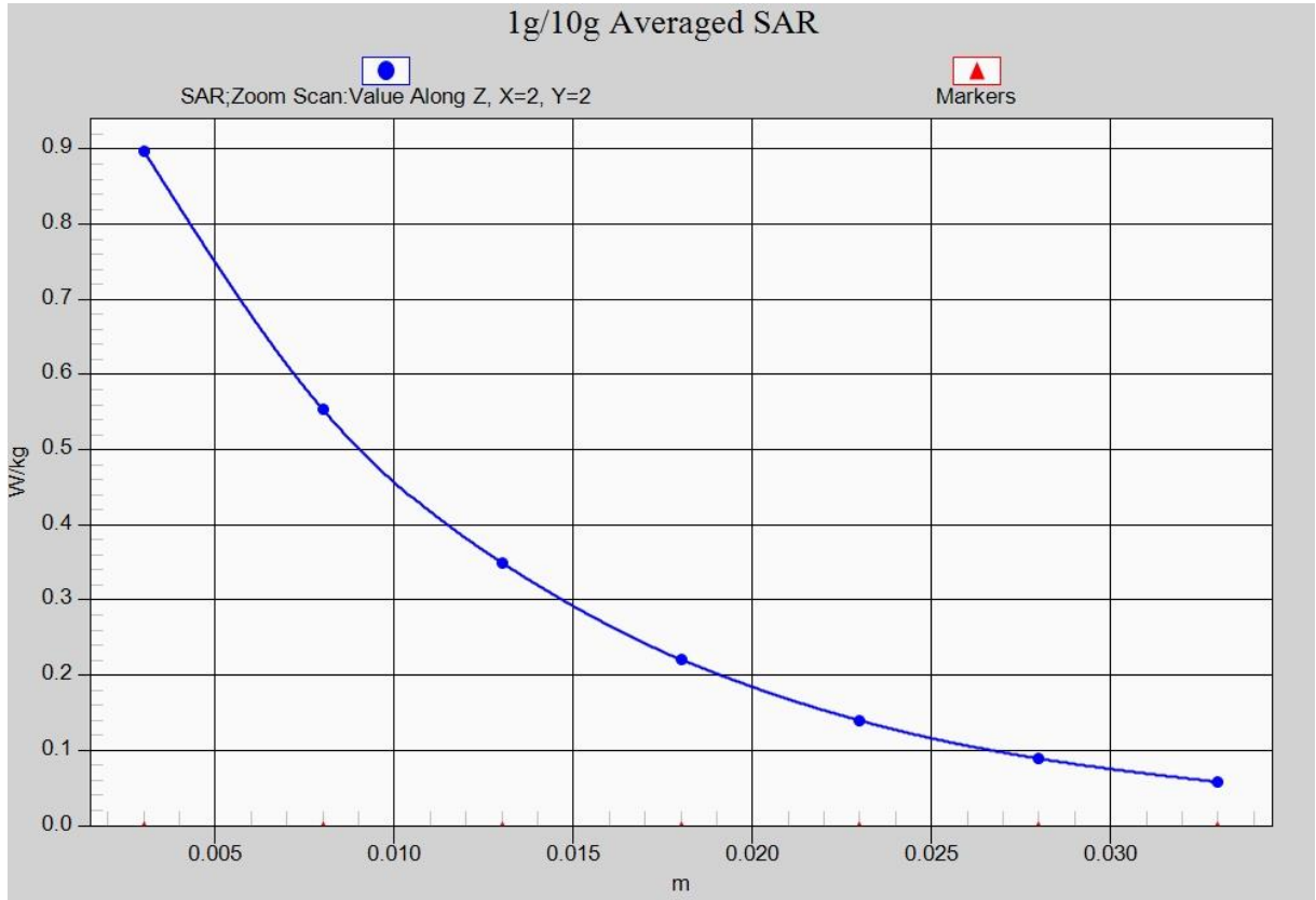
Fig. 27-1 Z-Scan at power reference point (LTE Band4)
