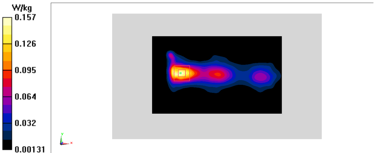
Fig.32 2450 MHz
