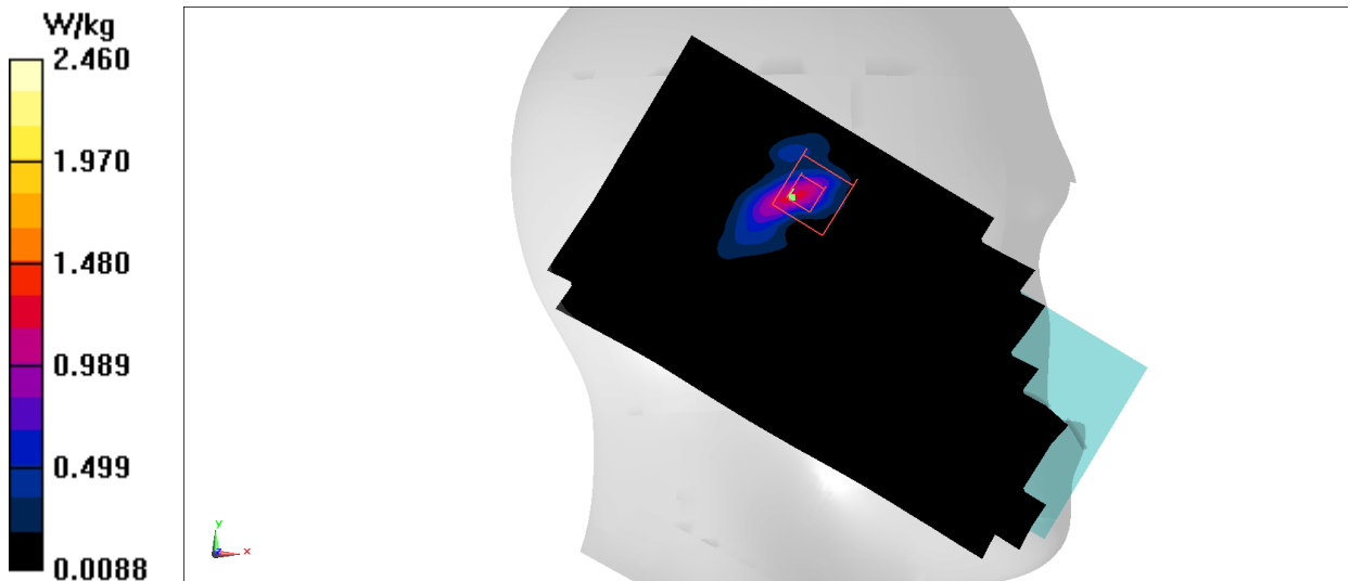
Fig.33 5GHz
