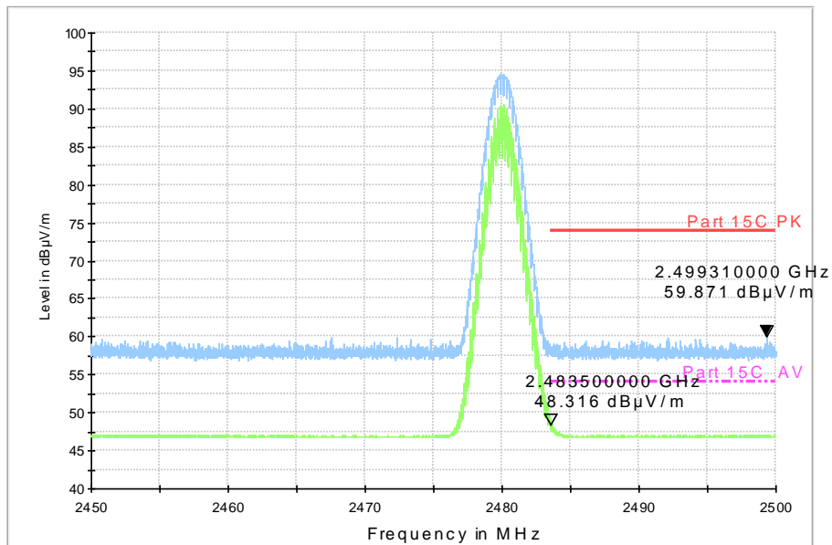
RE - Power-2.45GHz-2.5GHz
