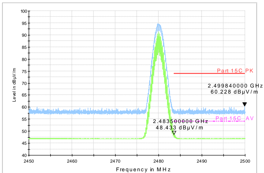
RE - Power-2.45GHz-2.5GHz
