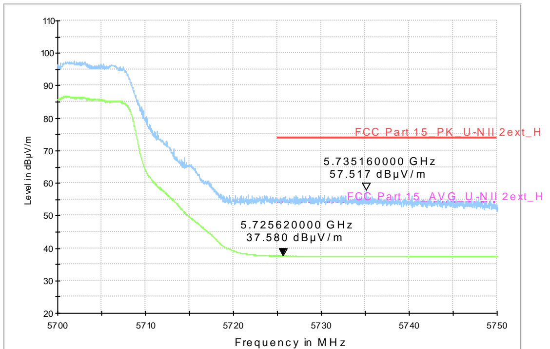
Fig. 49 Band Edges (802.11a, 5700MHz)
