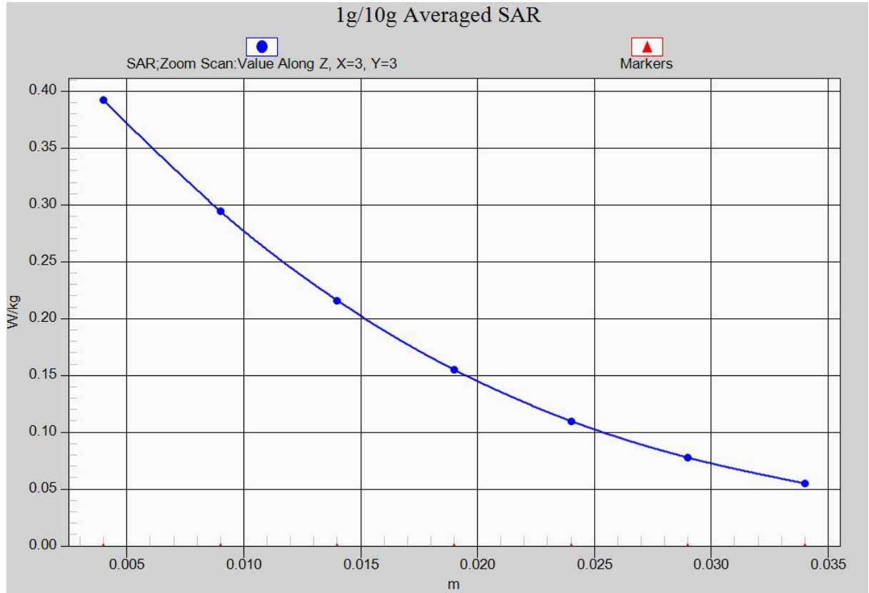
Fig. 27-1 Z-Scan at power reference point (LTE Band14)
