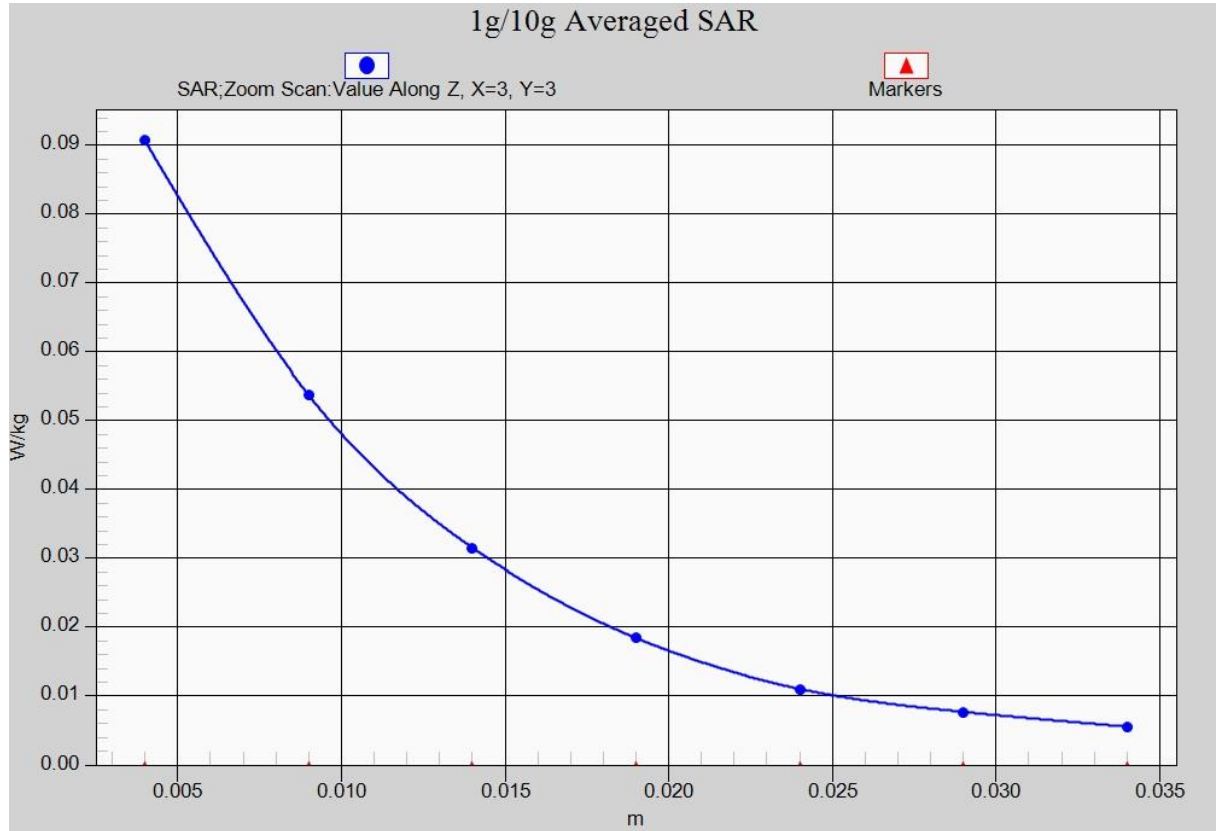
Fig. 28-1 Z-Scan at power reference point (LTE Band30)
