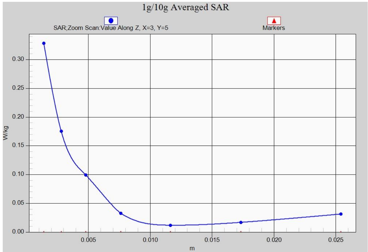
Fig. 39-1 Z-Scan at power reference point (5GHz)
