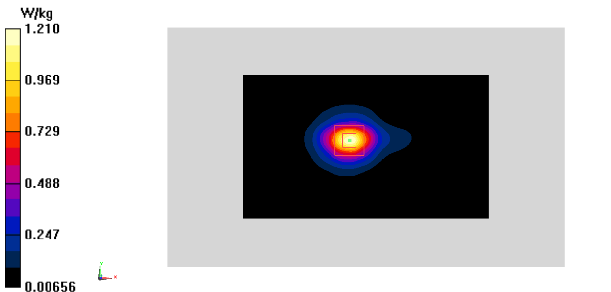
Fig.32 LTE Band 41
