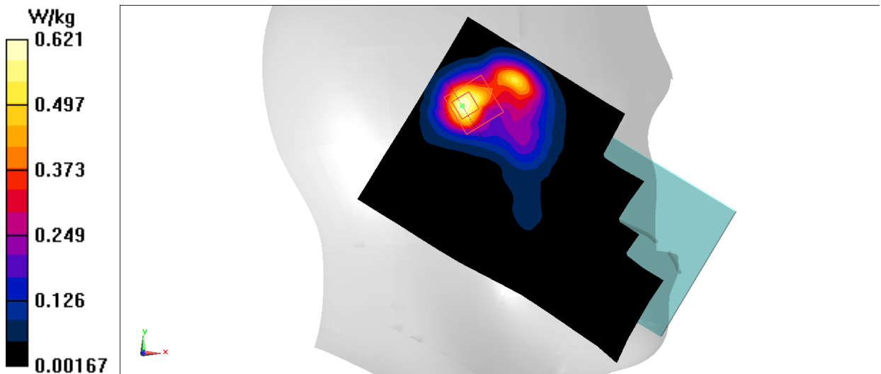
Fig.36 2450 MHz
