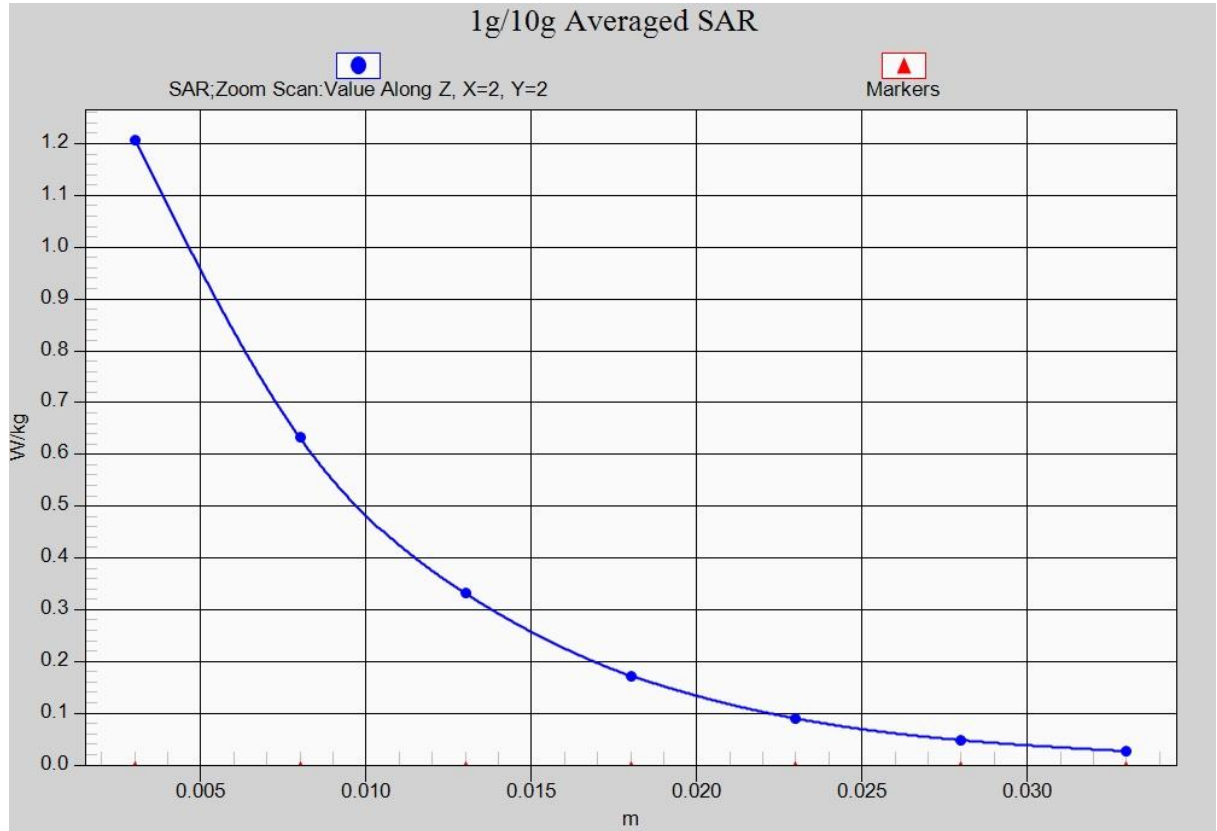
Fig. 32-1 Z-Scan at power reference point (LTE Band 41)
