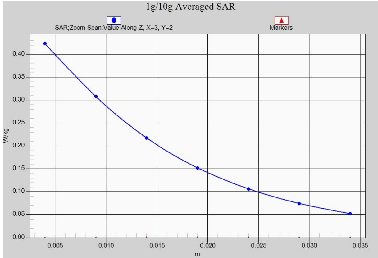
Fig. 25-1 Z-Scan at power reference point (LTE Band13)
