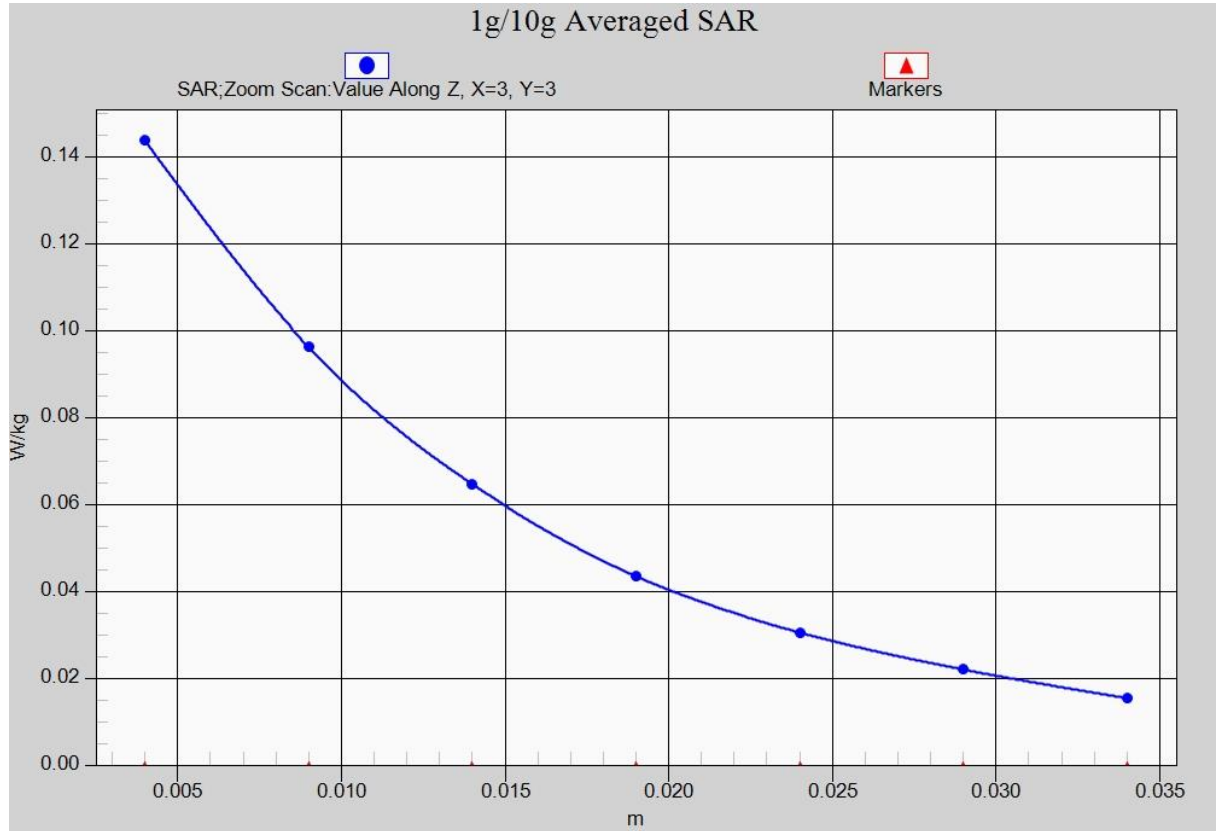
Fig. 33-1 Z-Scan at power reference point (LTE Band66)
