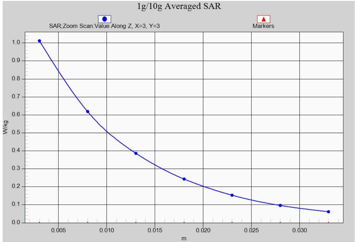
Fig. 34-1 Z-Scan at power reference point (LTE Band66)
