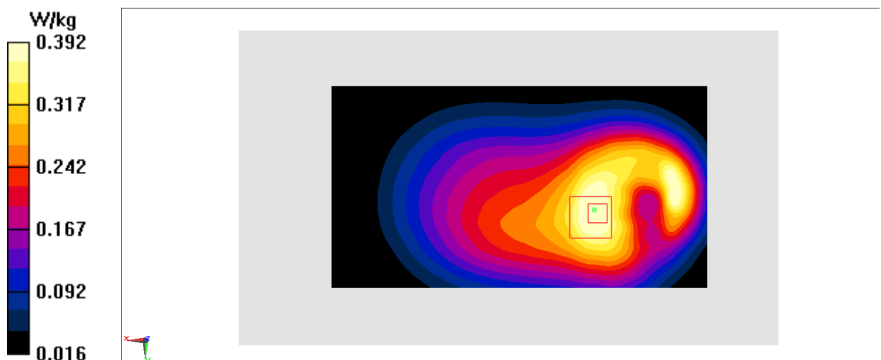
Fig.27 LTE Band14
