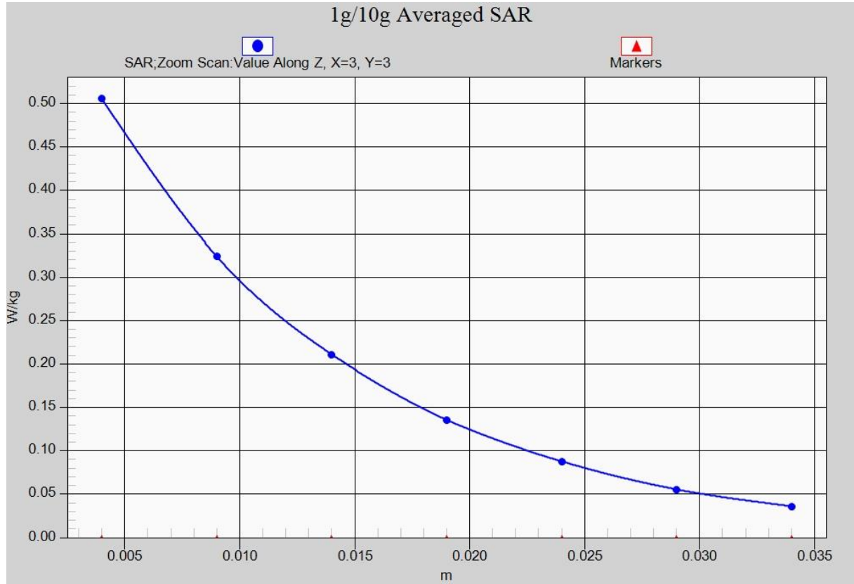
Fig. 35-1 Z-Scan at power reference point (LTE Band66)
