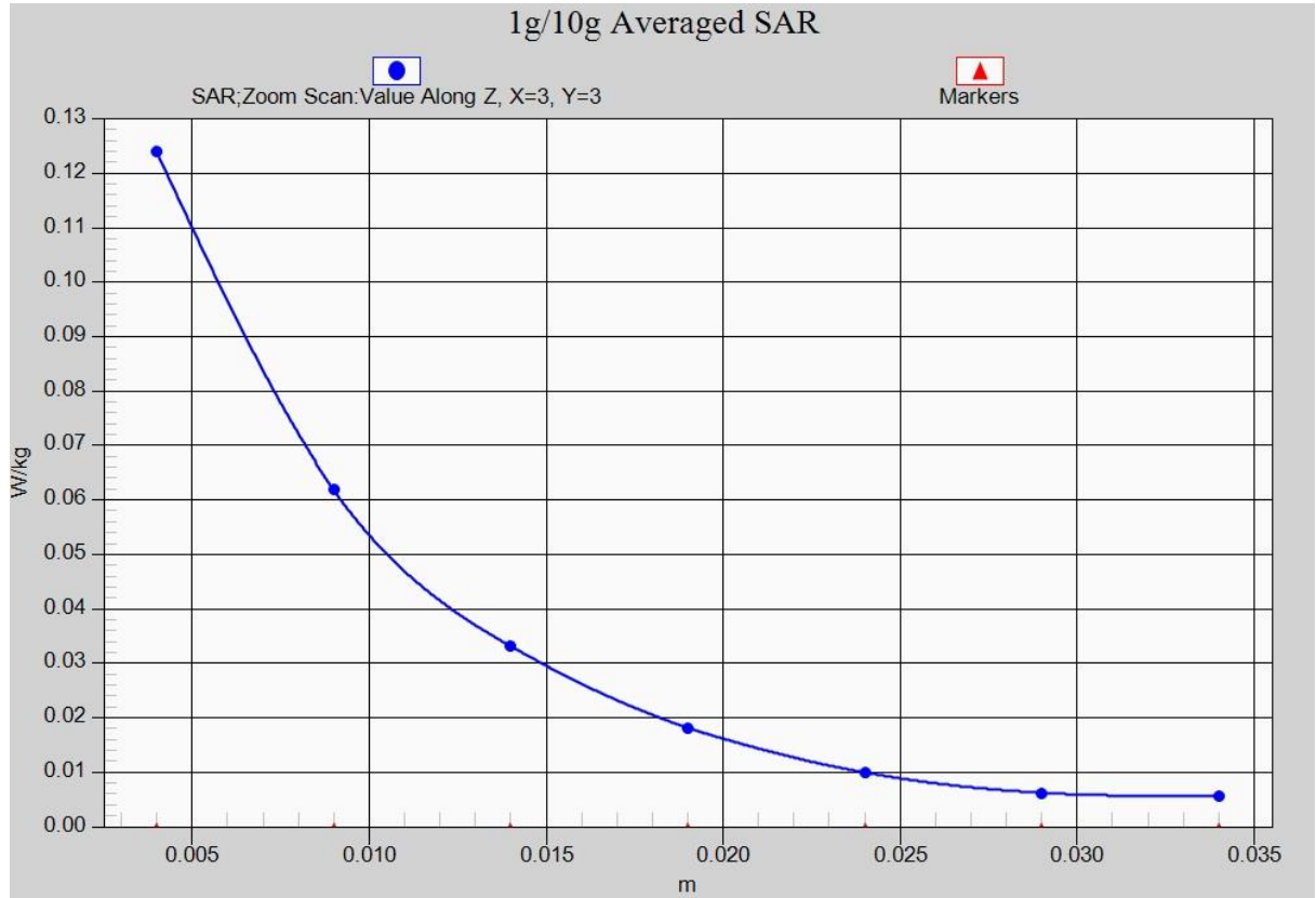
Fig. 31-1 Z-Scan at power reference point (LTE Band 41)
