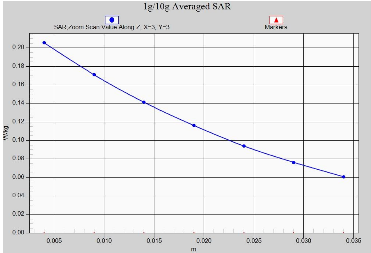
Fig. 24-1 Z-Scan at power reference point (LTE Band13)
