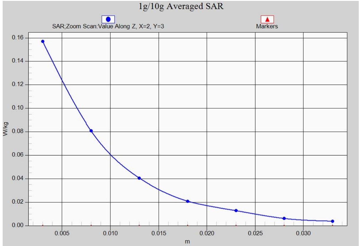
Fig. 37-1 Z-Scan at power reference point (2450 MHz)
