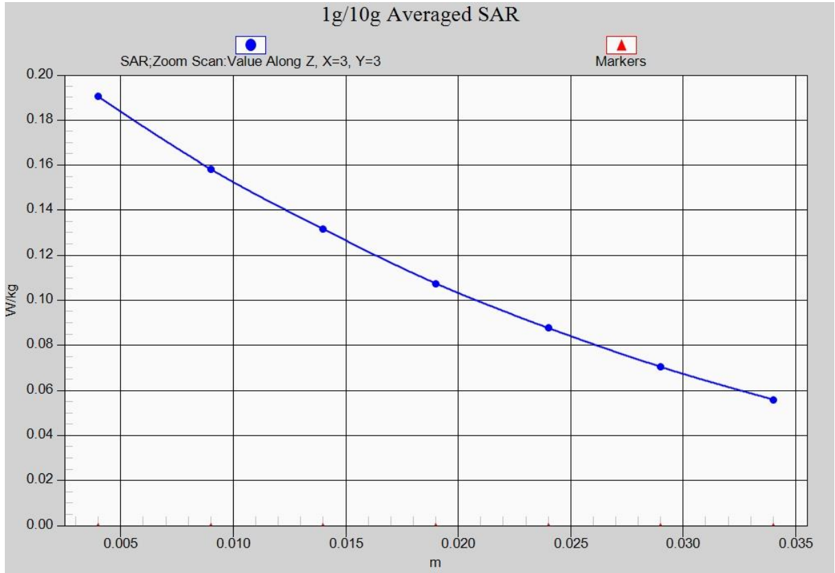
Fig. 26-1 Z-Scan at power reference point (LTE Band14)
