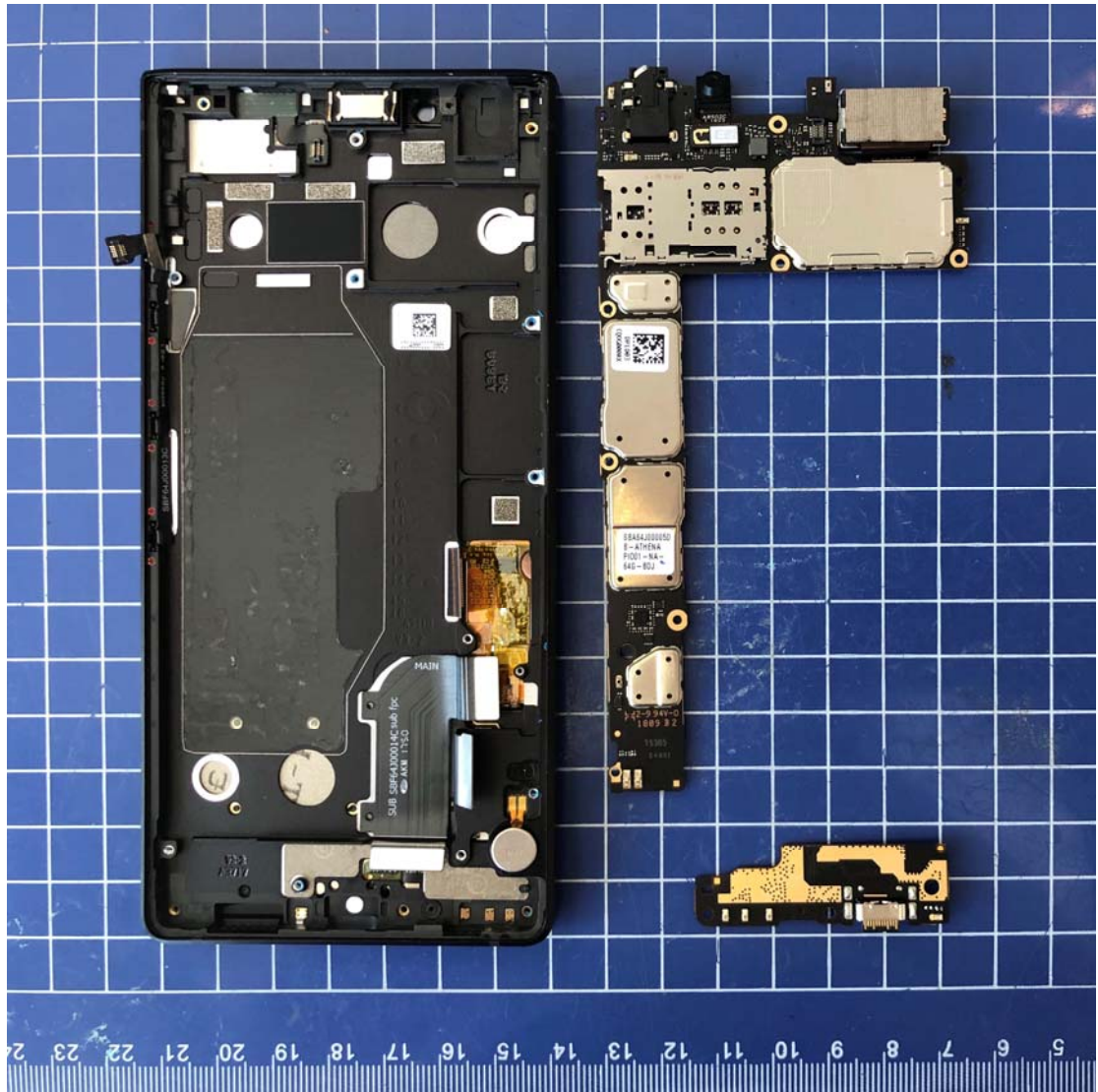
Pic A-3 Mobile phone Disassembly
