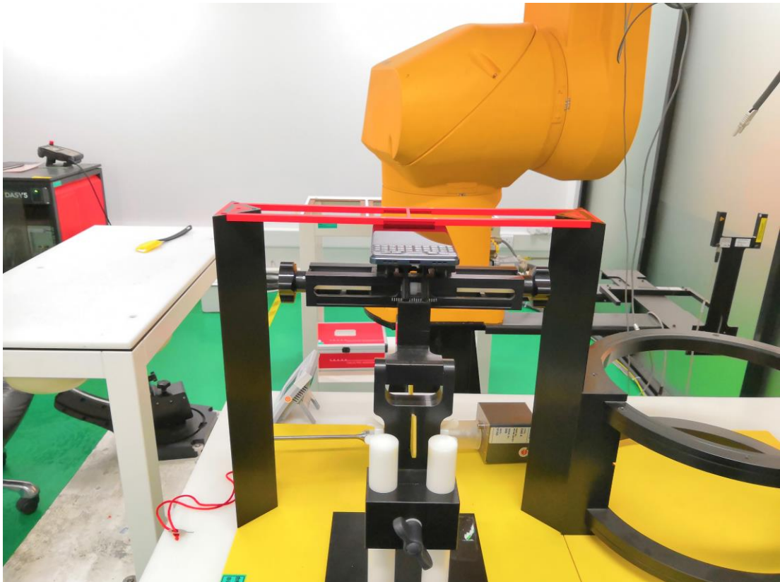
Picture 2: EUT Positioning for RF/T-coil
