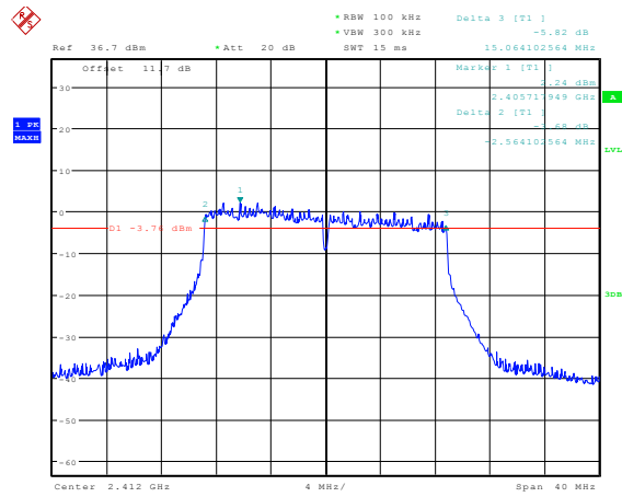
Fig.A.4.7 Occupied 6dB Bandwidth (802.11n-20MHz, Ch 1)
