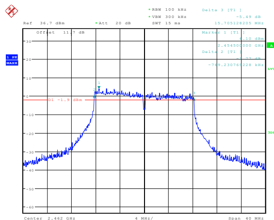
Fig.A.4.6 Occupied 6dB Bandwidth (802.11g, Ch 11)
