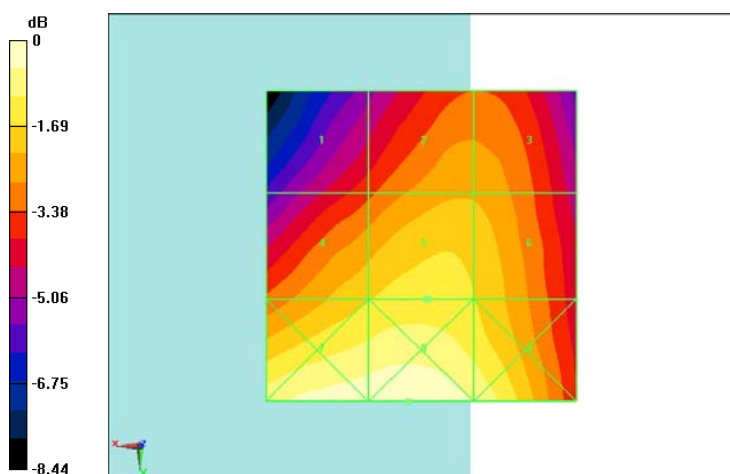
Fig B.1 HAC RF E-Field GSM 850 High
